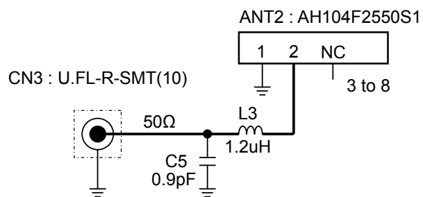
Type D Antenna
