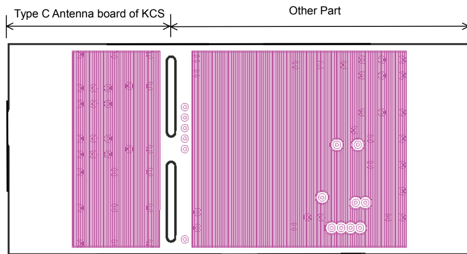
Fig. Component Layout (Solder side)
