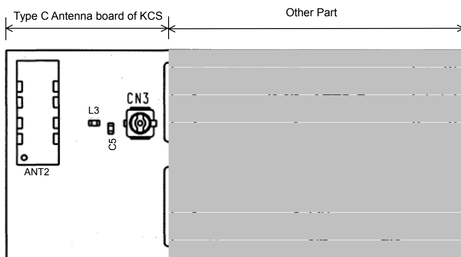
Fig. Component Layout (Component side)
