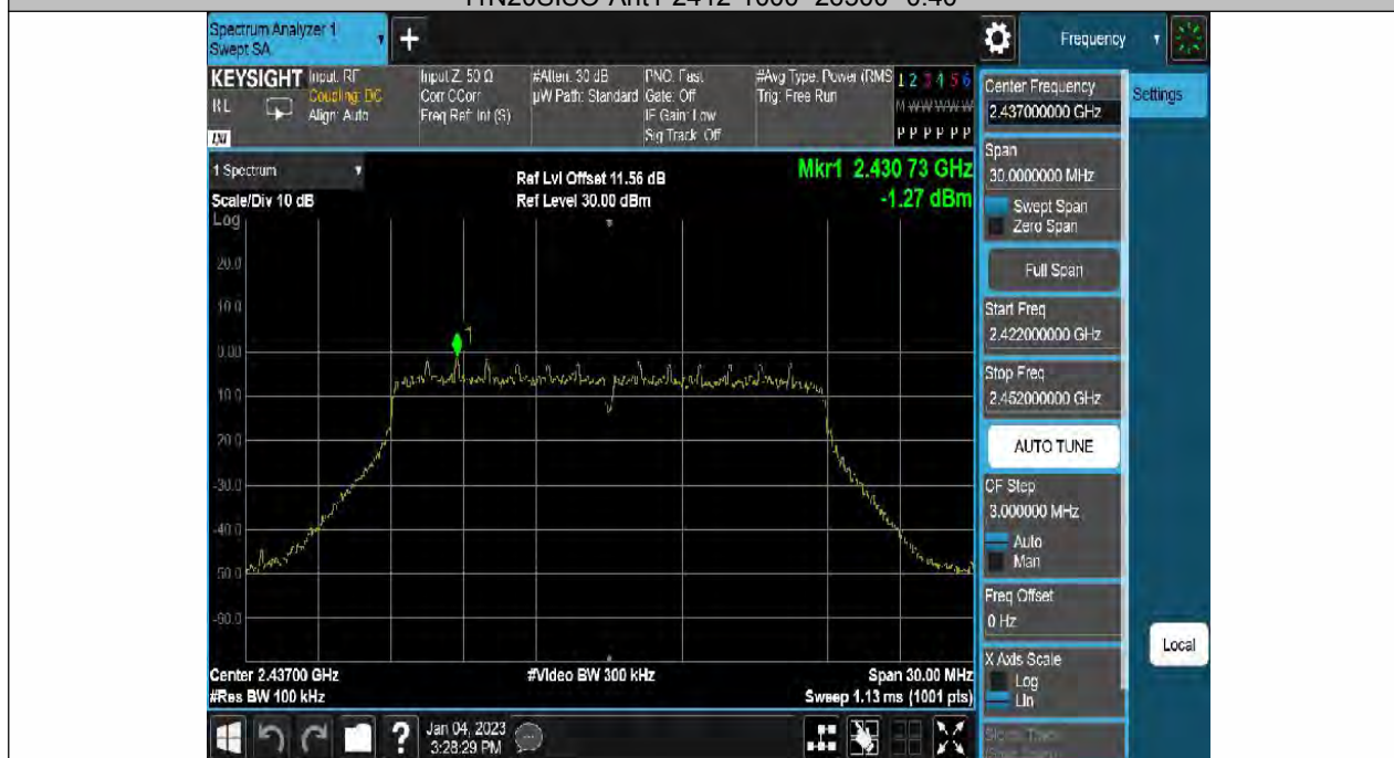
11N20SISO-Ant1-2437-0~Reference--1.27
