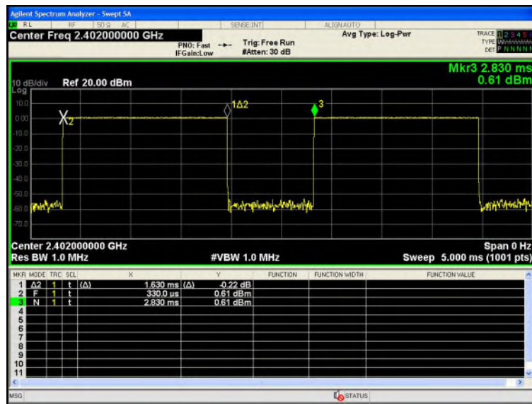
Test Mode: BDR---DH3
