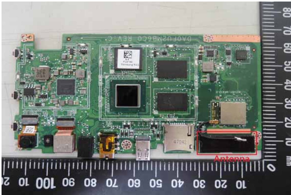
Antenna-1 Part No.: DQ614A00013
