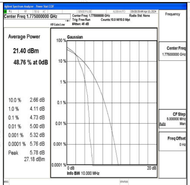
Band66-10MHz-16QAM-132622-1RB#0-PASS
