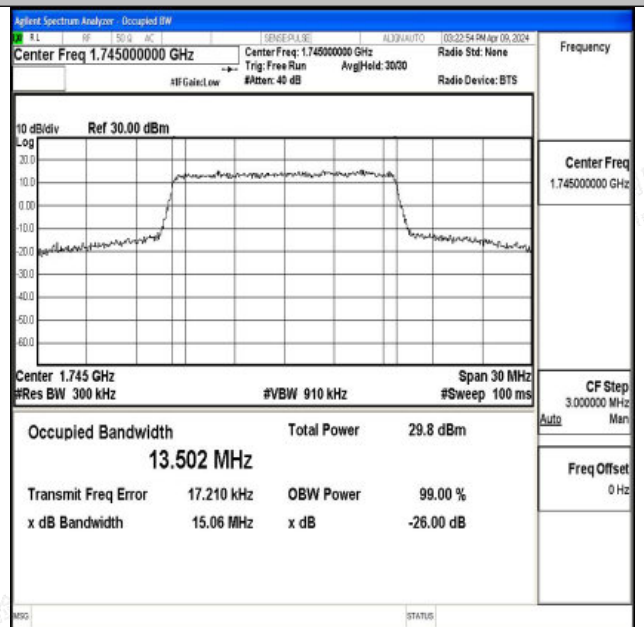
Band66-15MHz-16QAM-132322-75RB#0-PASS
