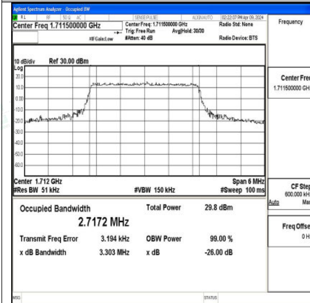
Band66-3MHz-QPSK-131987-15RB#0-PASS
