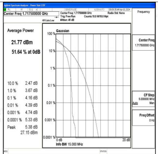
Band66-15MHz-16QAM-132047-1RB#0-PASS
