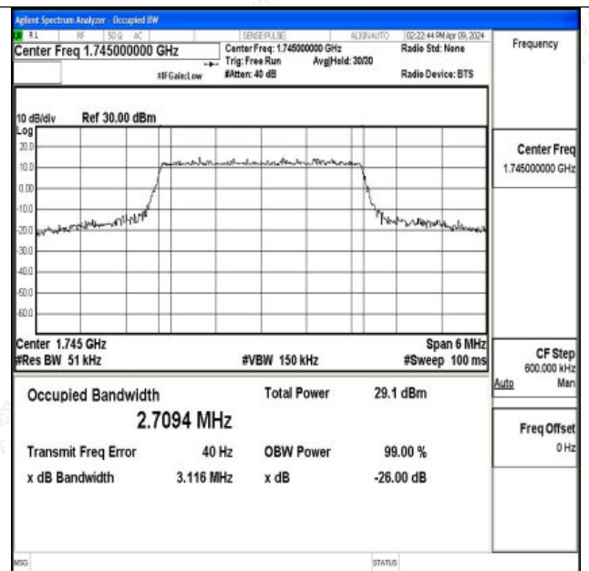
Band66-3MHz-16QAM-132322-15RB#0-PASS
