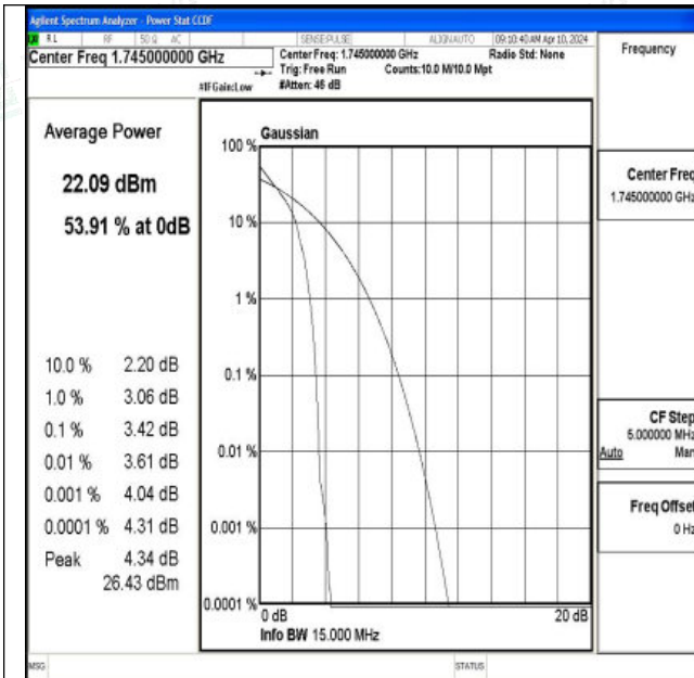
Band66-15MHz-QPSK-132322-1RB#0-PASS
