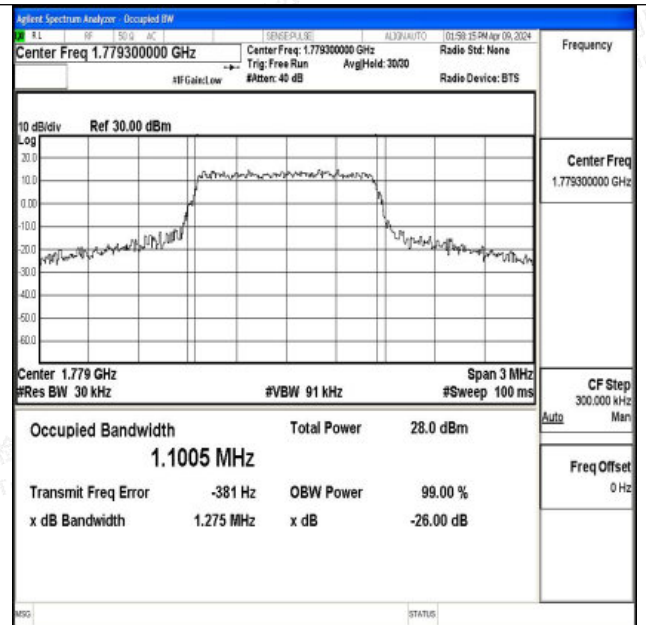
Band66-1.4MHz-16QAM-132665-6RB#0-PASS
