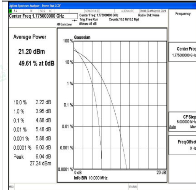
Band66-10MHz-QPSK-132622-50RB#0-PASS
