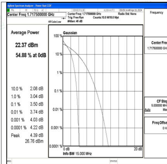
Band66-15MHz-QPSK-132047-1RB#0-PASS
