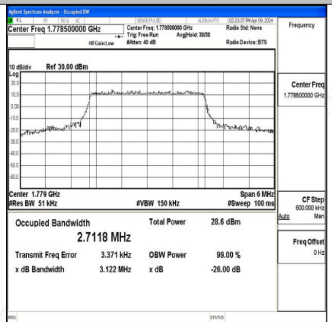
Band66-3MHz-16QAM-132657-15RB#0-PASS
