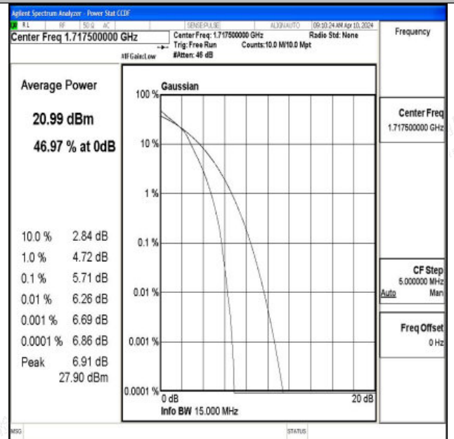
Band66-15MHz-16QAM-132047-75RB#0-PASS
