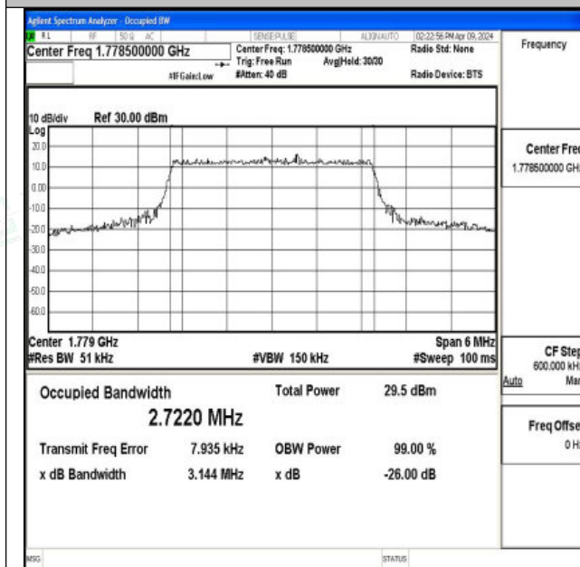
Band66-3MHz-QPSK-132657-15RB#0-PASS
