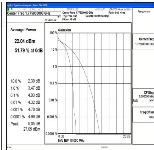
Band66-10MHz-QPSK-132622-1RB#0-PASS
