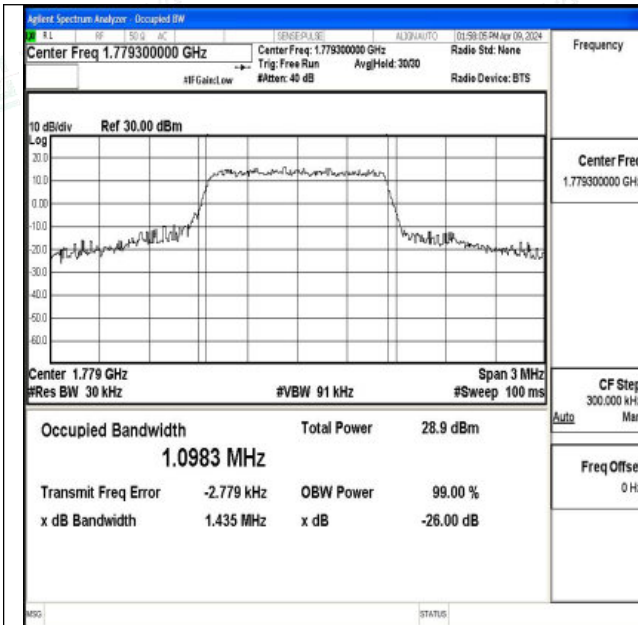
Band66-1.4MHz-QPSK-132665-6RB#0-PASS
