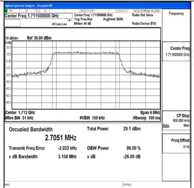
Band66-3MHz-16QAM-131987-15RB#0-PASS
