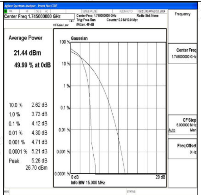
Band66-15MHz-16QAM-132322-1RB#0-PASS
