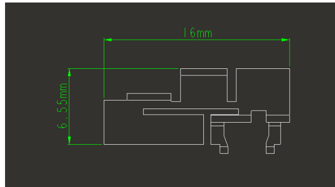
Thread antenna
