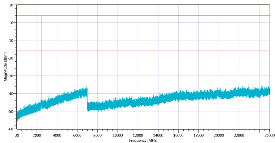
Plot_FCC Part 15.247 TX Spurious Conducted ~ WLAN2G4 b-mode 2437_14102020_103916.png
