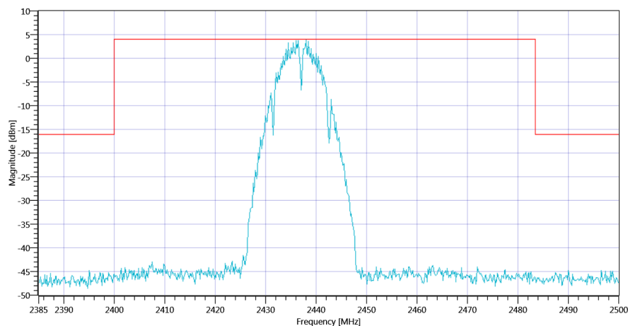
Plot_FCC Part 15.247 TX Spurious Conducted ~ WLAN2G4 b-mode 2437_14102020_103919.png
