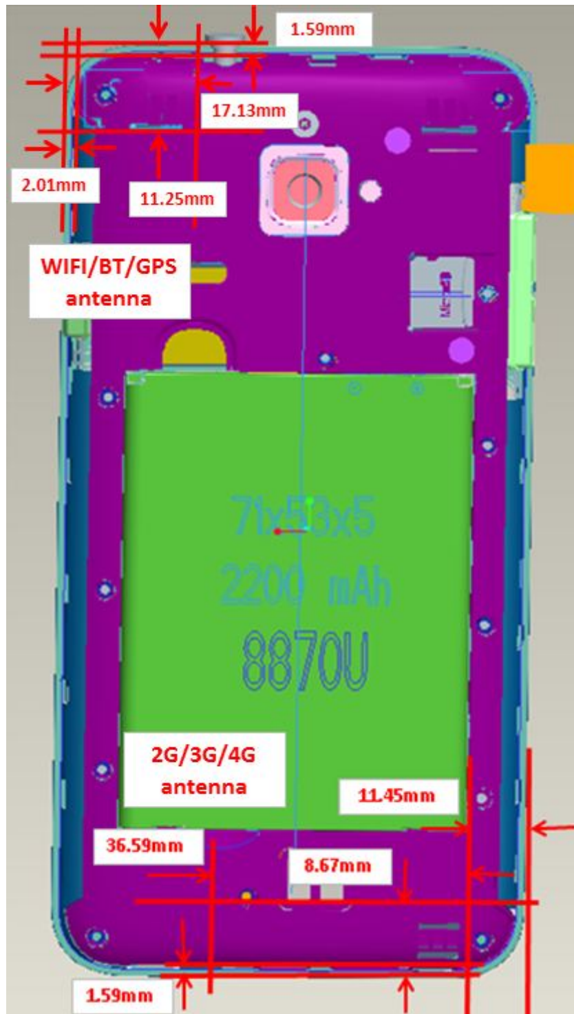
Antenna Location
