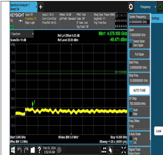
Band13_5MHz_QPSK_23205_1RB#0_3000~10000_3000~10000
