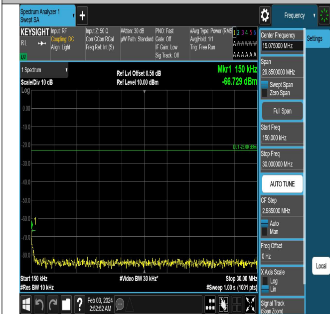
Band13_5MHz_QPSK_23230_1RB#0_0.15~30_0.15~30
