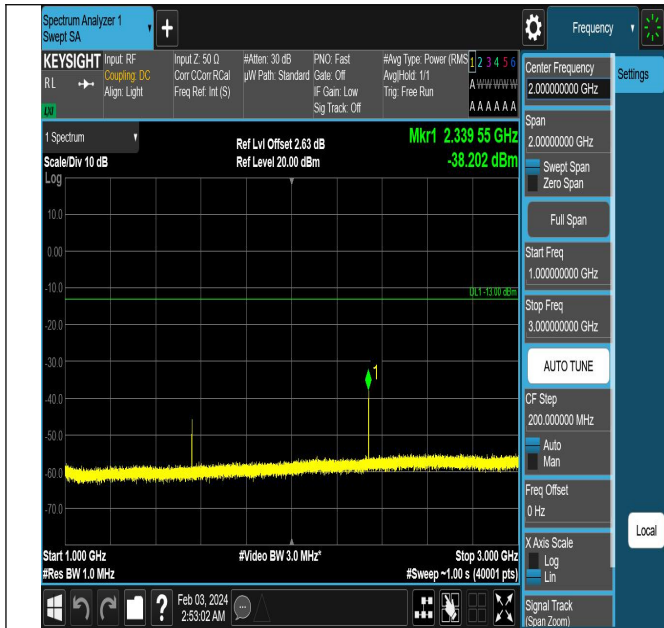
Band13_5MHz_QPSK_23230_1RB#0_1000~3000_1000~3000
