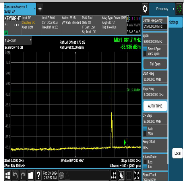
Band13_5MHz_QPSK_23230_1RB#0_30~1000_30~1000
