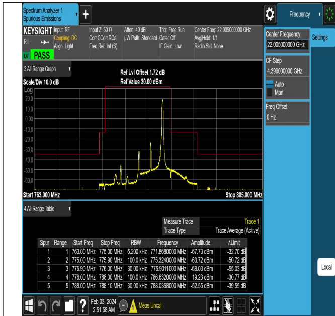
Band13_5MHz_QPSK_23255_1RB#24
