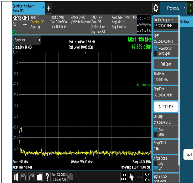
Band13_10MHz_QPSK_23230_1RB#0_0.15~30_0.15~30
