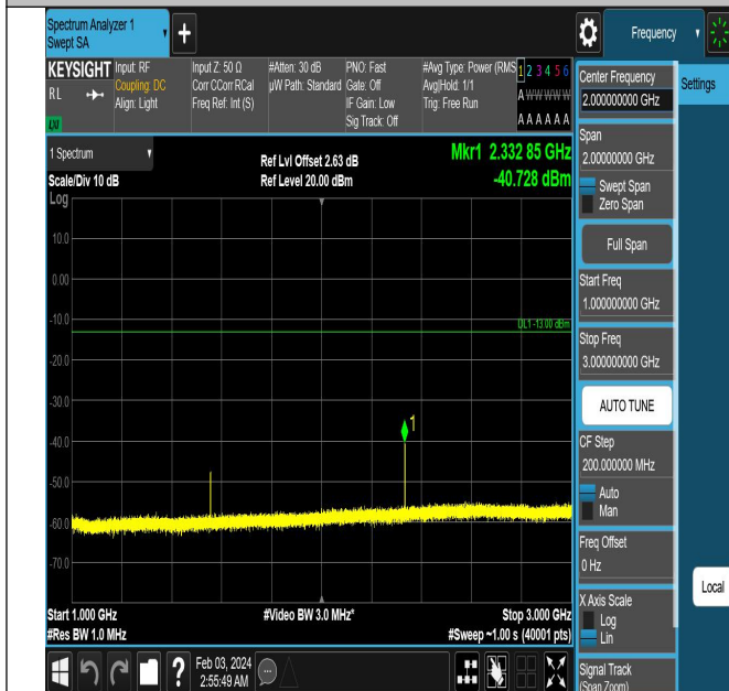
Band13_10MHz_QPSK_23230_1RB#0_1000~3000_1000~30
