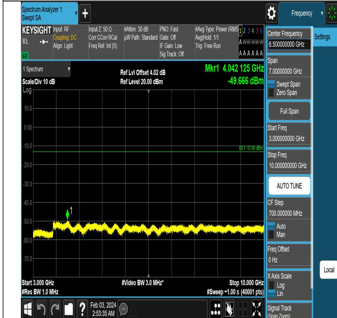
Band13_5MHz_QPSK_23255_1RB#0_3000~10000_3000~10000
