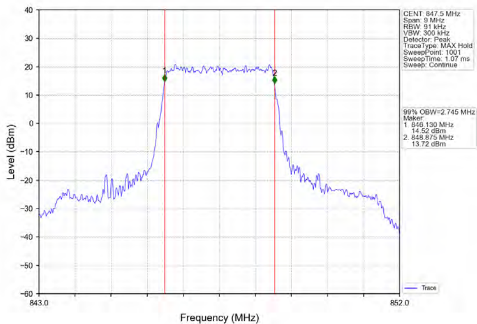
Band5_3MHz_QPSK_HCH_847.5MHz_RB_15_0_NTNV
