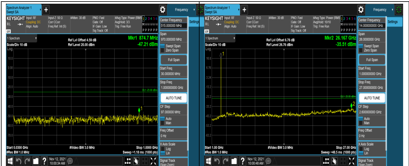
Band41-5MHz-QPSK-41215-1RB#0-Range1:30~1000MHz
