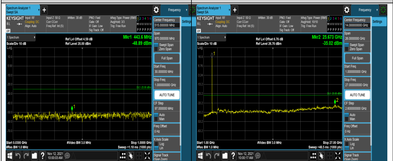
Band41-5MHz-16QAM-40065-1RB#0-Range1:30~1000MHz
