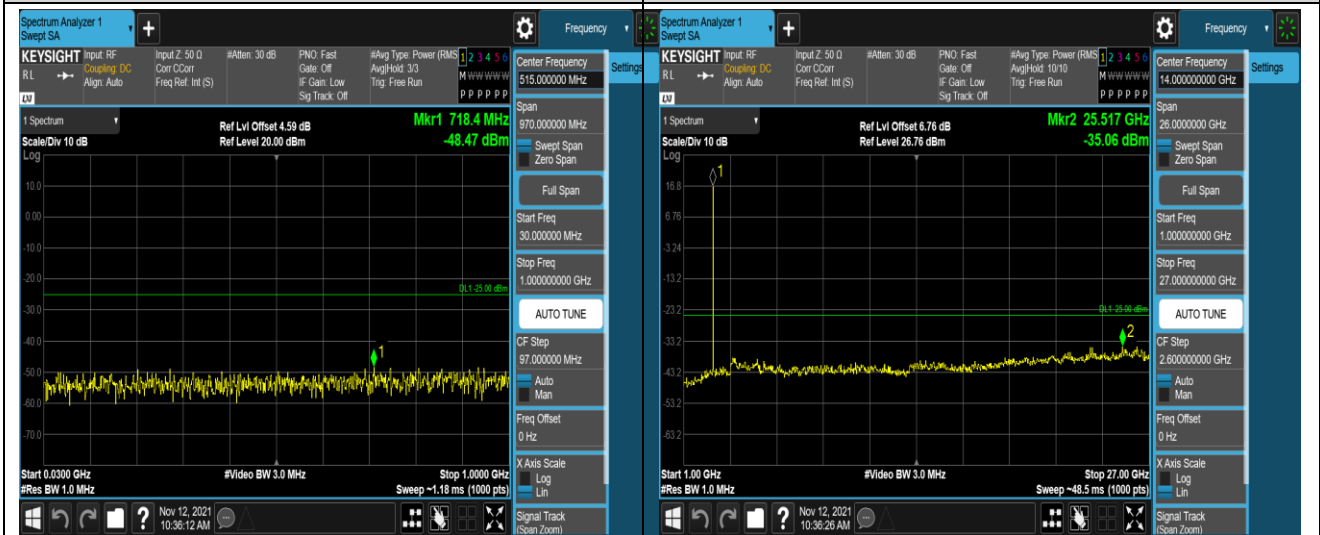
Band41-20MHz-QPSK-41140-1RB#0-Range1:30~1000MHz
