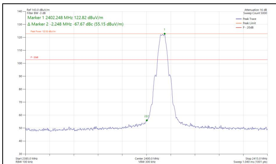
Figure 227 - Bluetooth LE1M, MIMO, Core 0 - Core 1 - 2402 MHz Band Edge Frequency 2400 MHz
