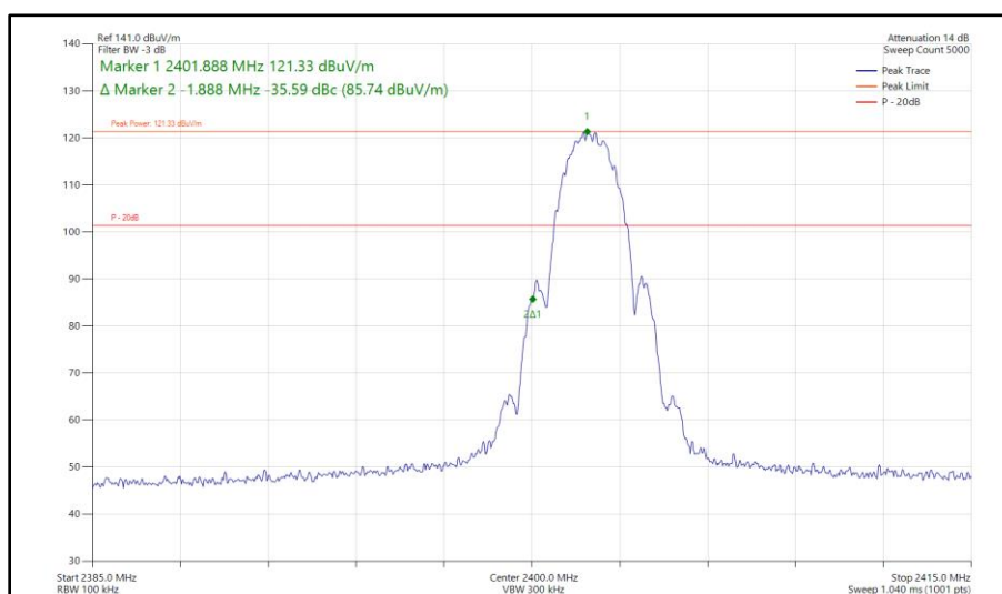
Figure 228 - Bluetooth LE2M, MIMO, Core 0 - Core 1 - 2402 MHz Band Edge Frequency 2400 MHz
