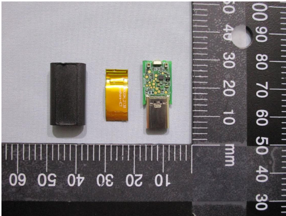
Internal Photos UD2202u Pic 1
