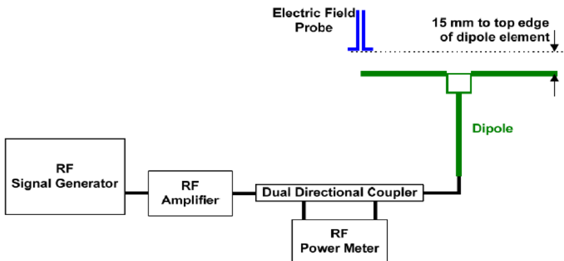
Fig.4 System verification
