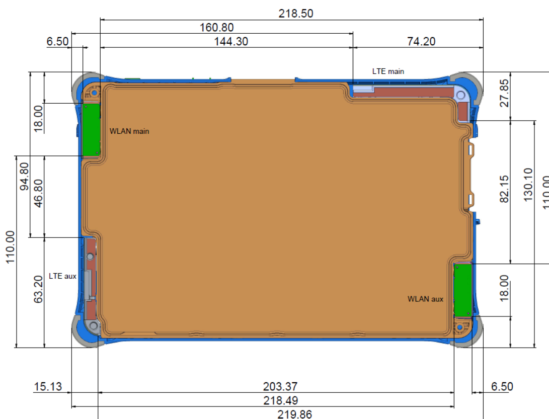
Test Position of Portable Devices
