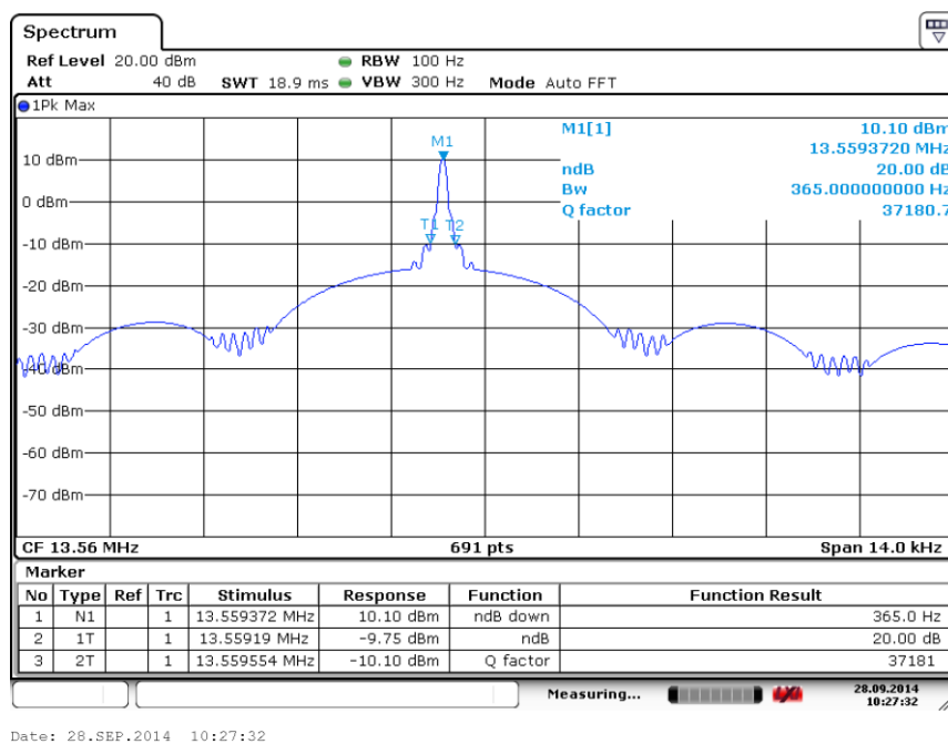
Fig. 4 Occupied 20dB Bandwidth
