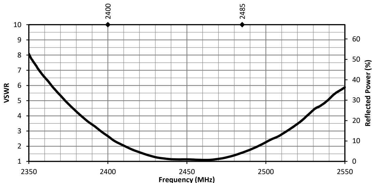
Figure 2. 2.4-CPA VSWR
