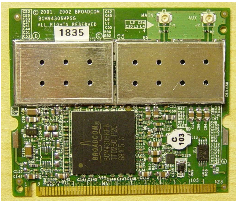
WLAN – Top view
