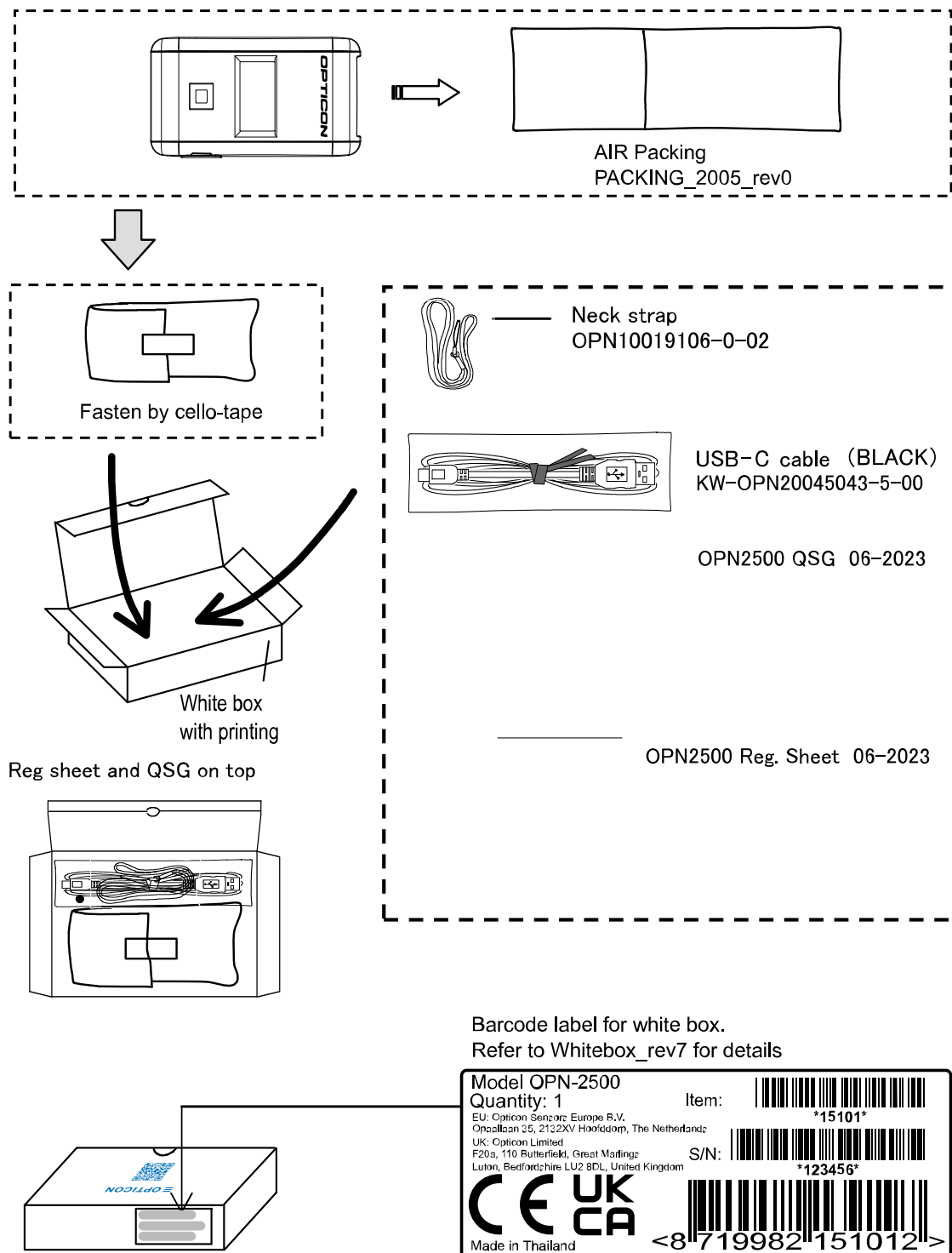
Figure 11: Individual Packaging
