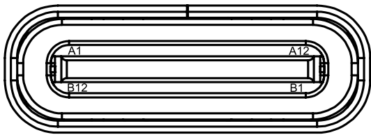
Figure 8: USB B connector
