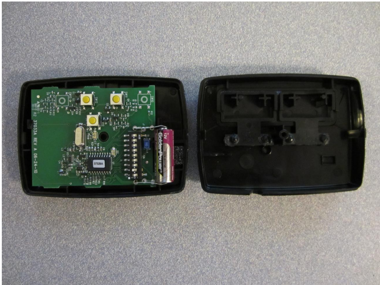
Figure 1: Internal Photos / PCB Top
