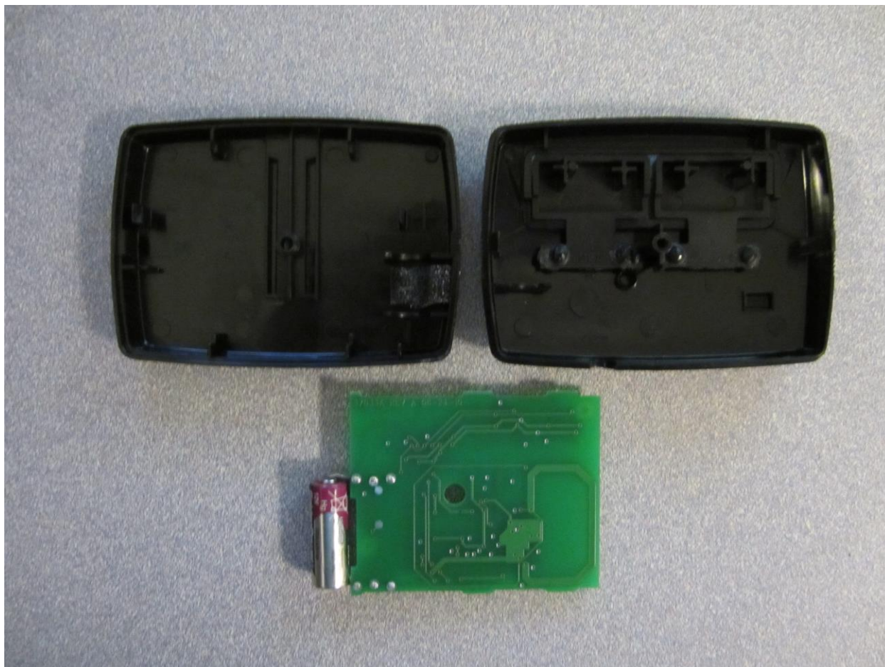
Figure 2: Internal Photos / PCB Bottom
