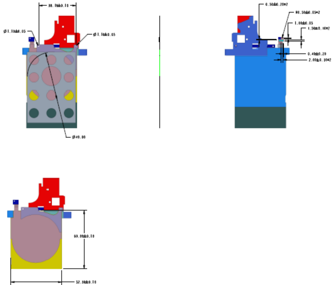
Mechanical Drawing
