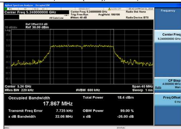
U-NII-1,802.11n(HT20),5240MHz,Ant1
