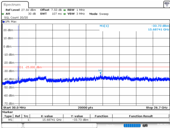
20MHz_High_QPSK_1@0(30MHz~26.7GHz)
