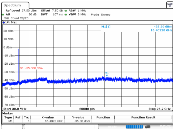
20MHz_Low_QPSK_1@0(30MHz~26.7GHz)
