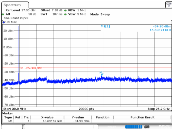
15MHz_Middle_QPSK_1@0(30MHz~26.7GHz)
