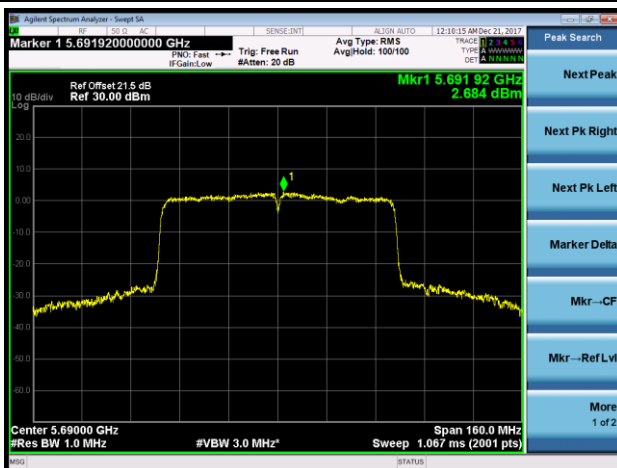
Channel 138 (5690MHz)
