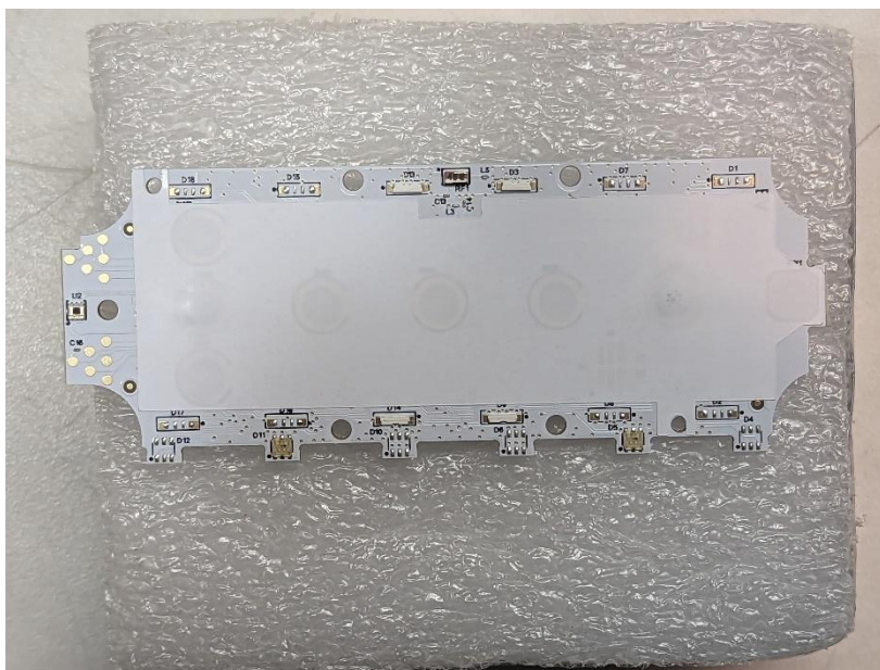
Photograph 26: Keypad PCB Face 1
