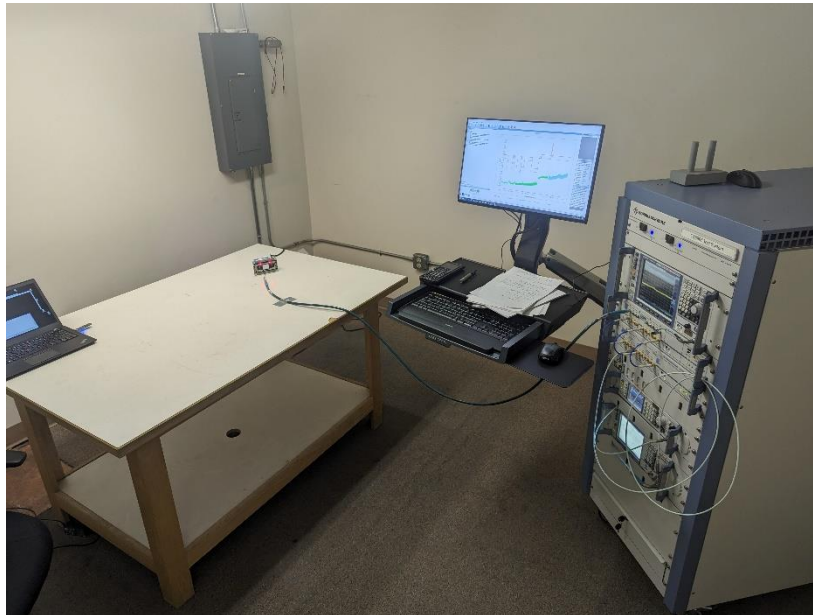
Photograph 8: Antenna Port Conducted Test Setup
