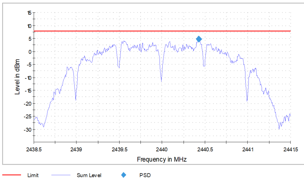
Graph 13: Middle Channel 10 kHz PSD Plot
