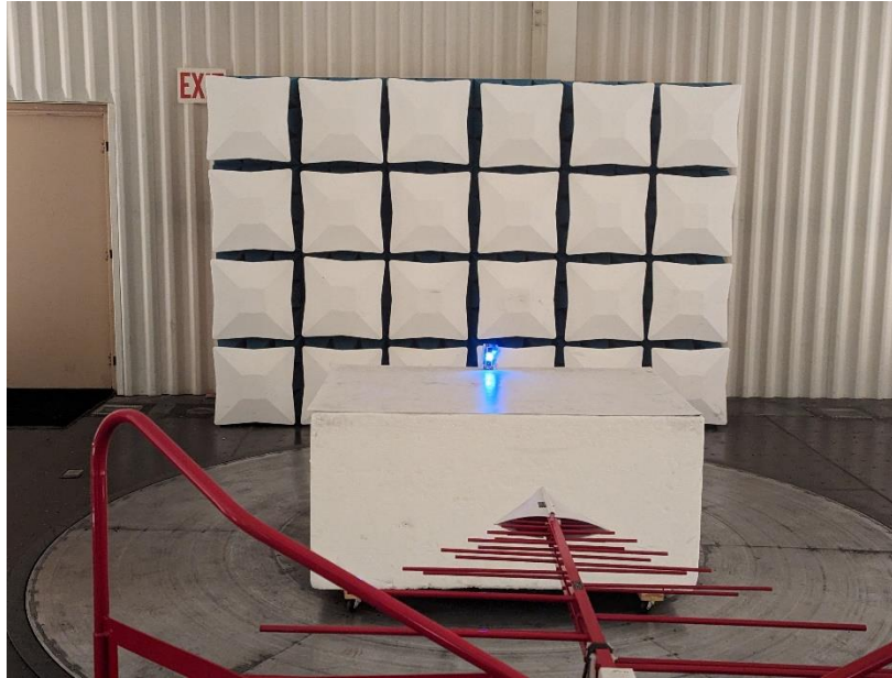
Photograph 1: Front View Radiated Emissions Worst-Case Configuration – Frequencies Below 1000 MHz
