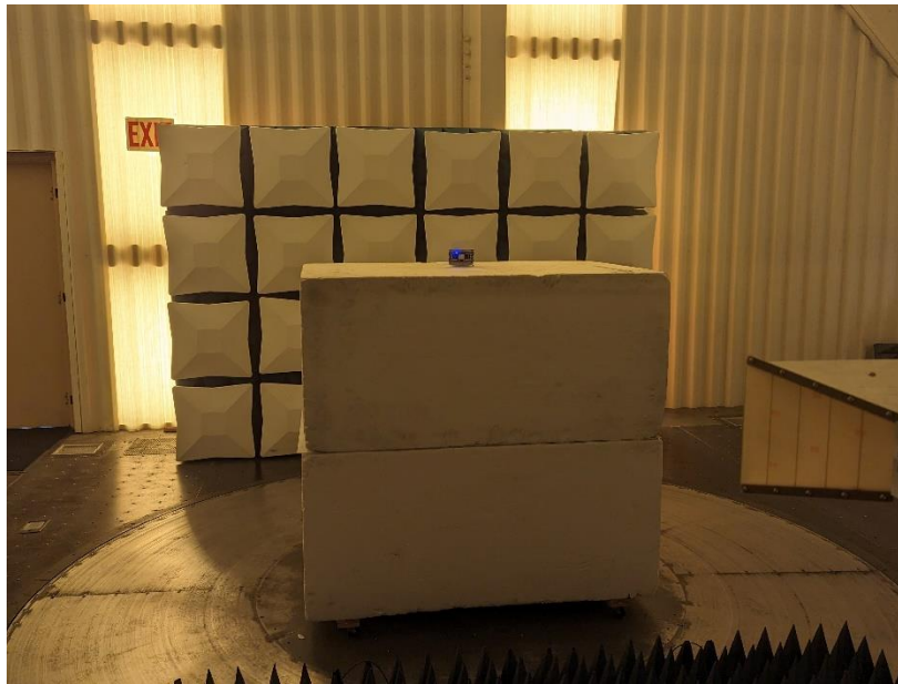
Photograph 3: Front View Radiated Emissions Worst-Case Configuration “Long Edge” Orientation—Frequencies Above 1000 MHz
