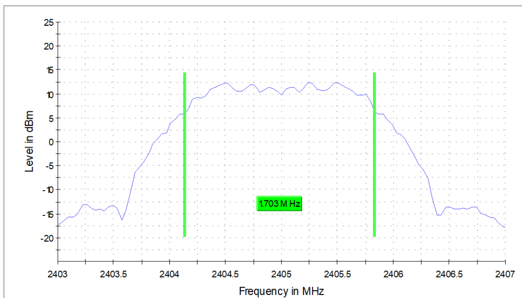
6 dB Bandwidth
