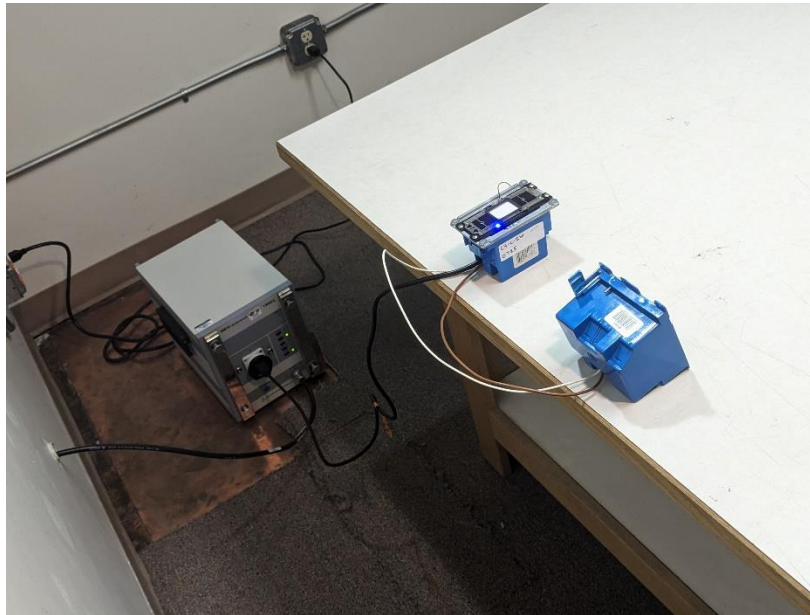
Photograph 10: Back View Conducted Emissions Worst-Case Configuration
