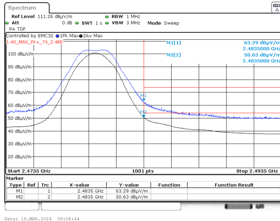
Graph 8: Upper Band Edge Plot (Transmitting 2480MHz, Power Level 18)
