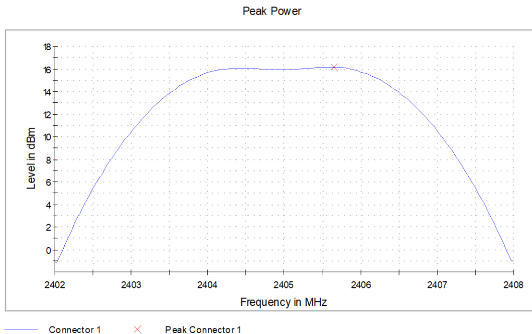
Graph 4: Lowest Channel Output Power Plot
