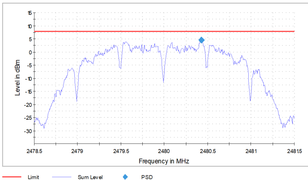
Graph 14: Highest Channel Output 10 kHz PSD Plot
