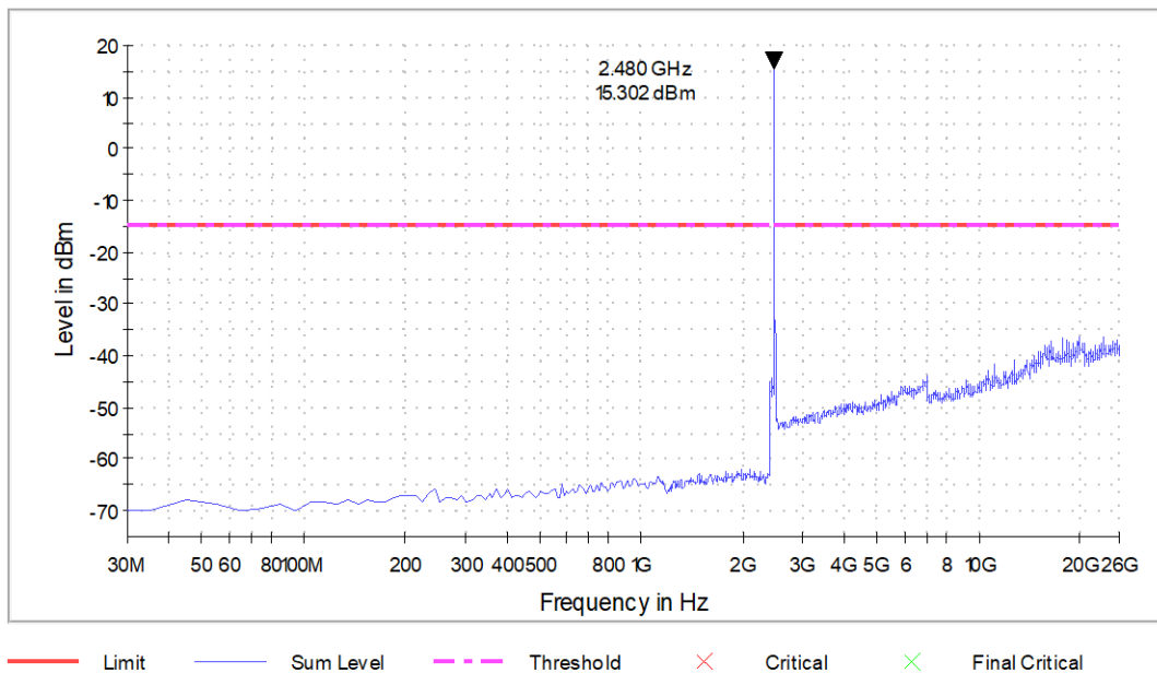
Graph 11: Transmitting on 2480MHz (Power Level 18)
