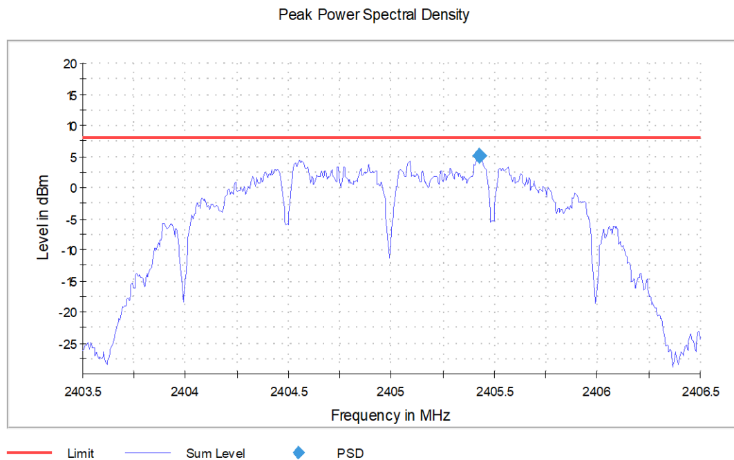
Graph 12: Lowest Channel 10 kHz PSD Plot
