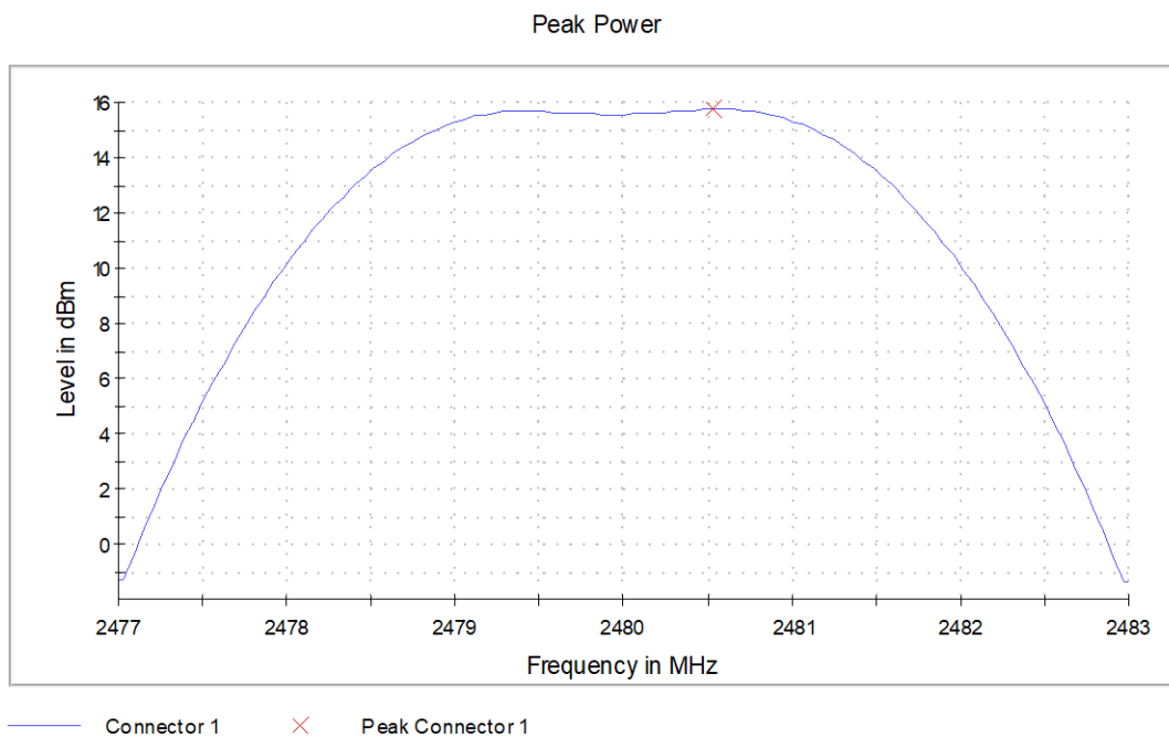
Graph 6: Highest Channel Output Power Plot
