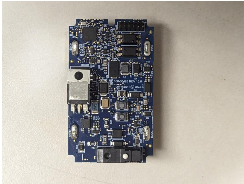
Photograph 20: Motherboard PCB Face 1
