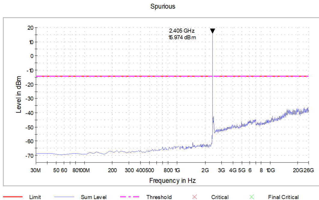
Graph 9: Transmitting on 2405MHz (Power Level 18)
