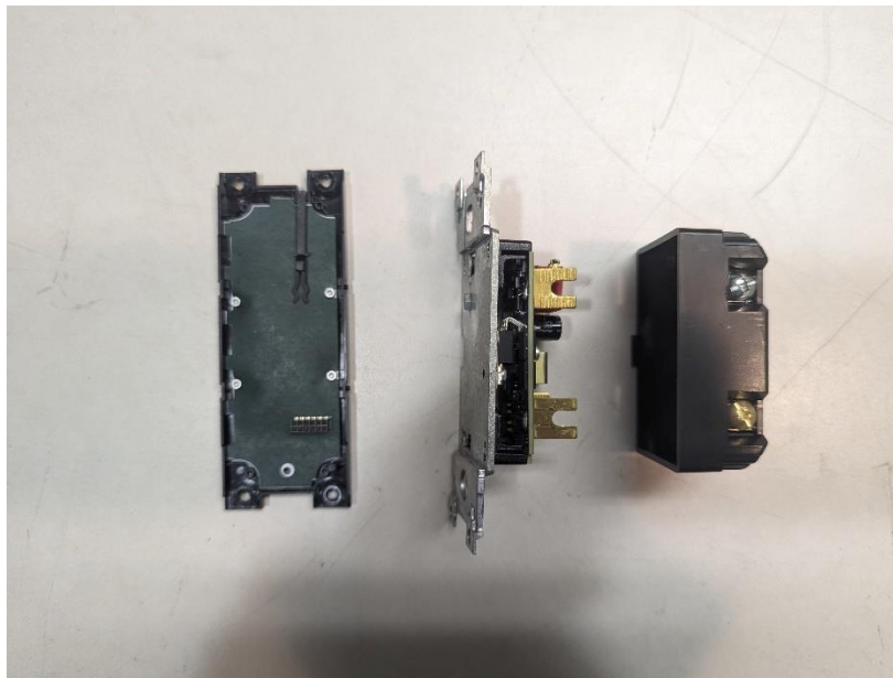
Photograph 18: EUT Keypad, Motherboard, and Enclosure
