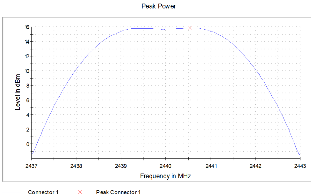
Graph 5: Middle Channel Output Power
