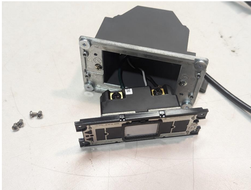
Photograph 17: EUT Placement in Junction Box Enclosure
