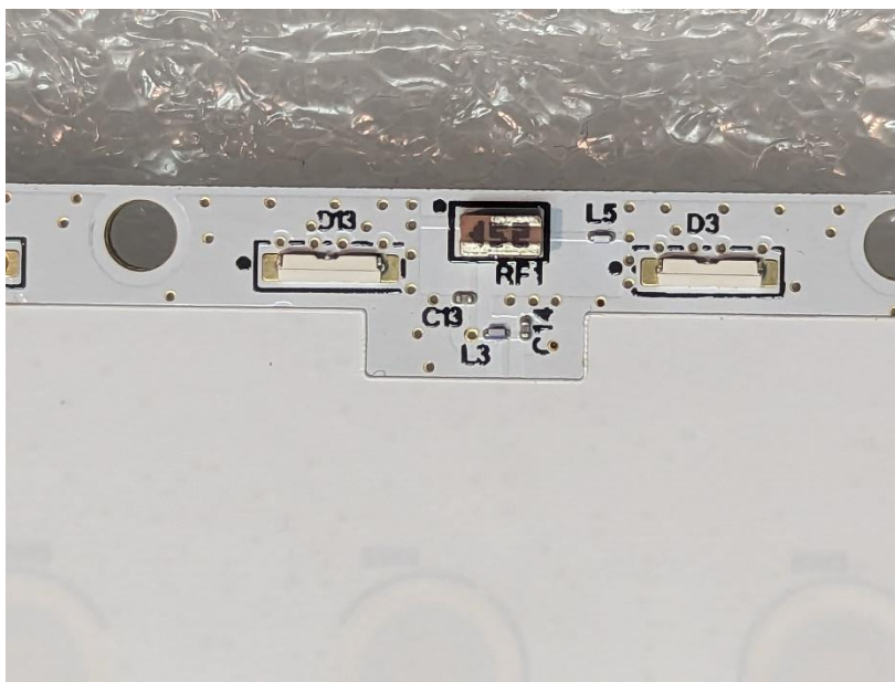
Photograph 32: Antenna Circuitry Close-Up
