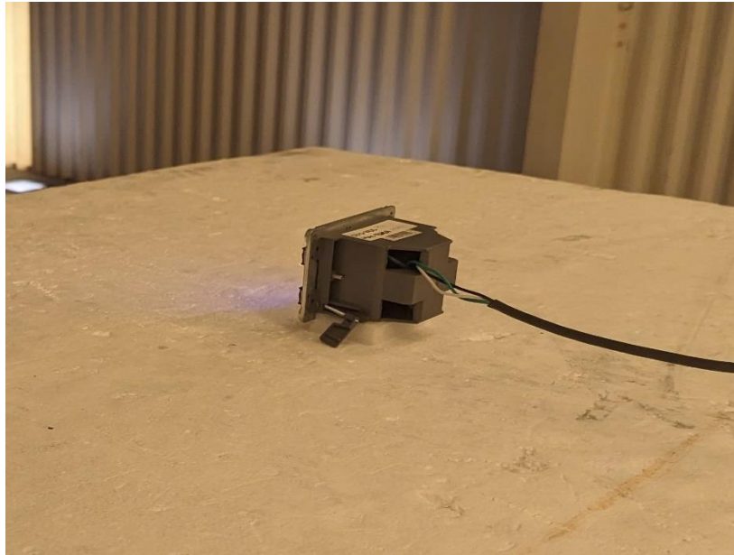
Photograph 5: Tested Orientation 1 – “Long Edge Orientation”
