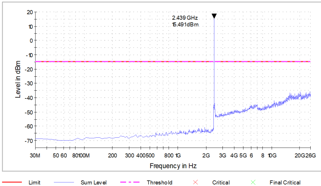
Graph 10: Transmitting on 2440MHz (Power Level 18)
