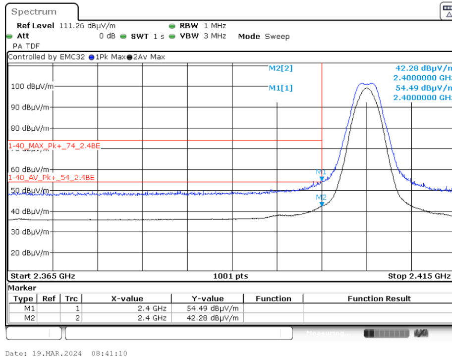
Graph 7: Lower Band Edge Plot (Transmitting 2405MHz, Power Level 18)
