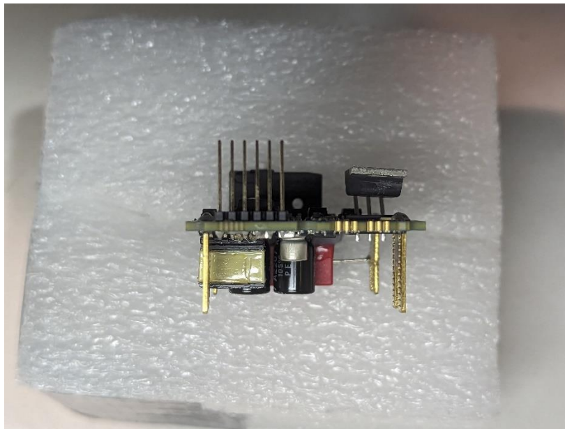
Photograph 22: Motherboard PCB Face 3
