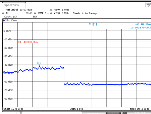
Band4_1.4MHz_QPSK_19957_1_0_Low_12000_26500_-41.4_PASS__
