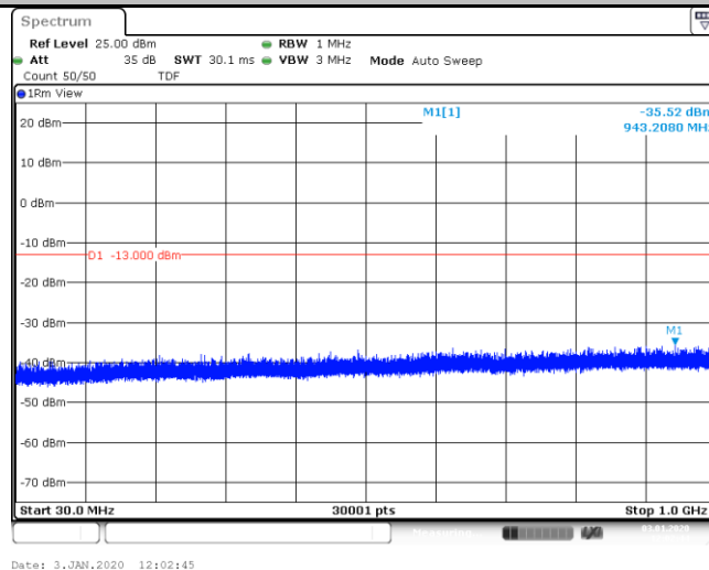
Band4_1.4MHz_16QAM_20393_1_5_Low_30_1000_-35.52_PASS__
