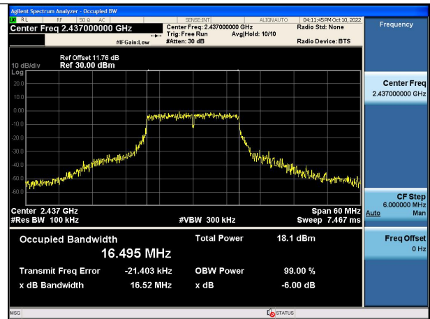
Test Mode:802.11g 2437MHz Chain0
