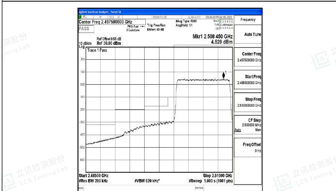
Band7_10MHz_QPSK_20800_50RB#0
