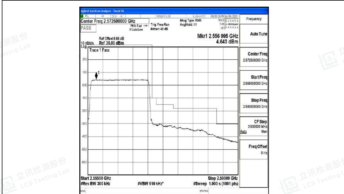
Band7_15MHz_16QAM_21375_75RB#0
