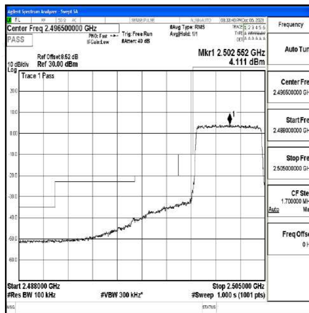
Band7_5MHz_16QAM_20775_25RB#0
