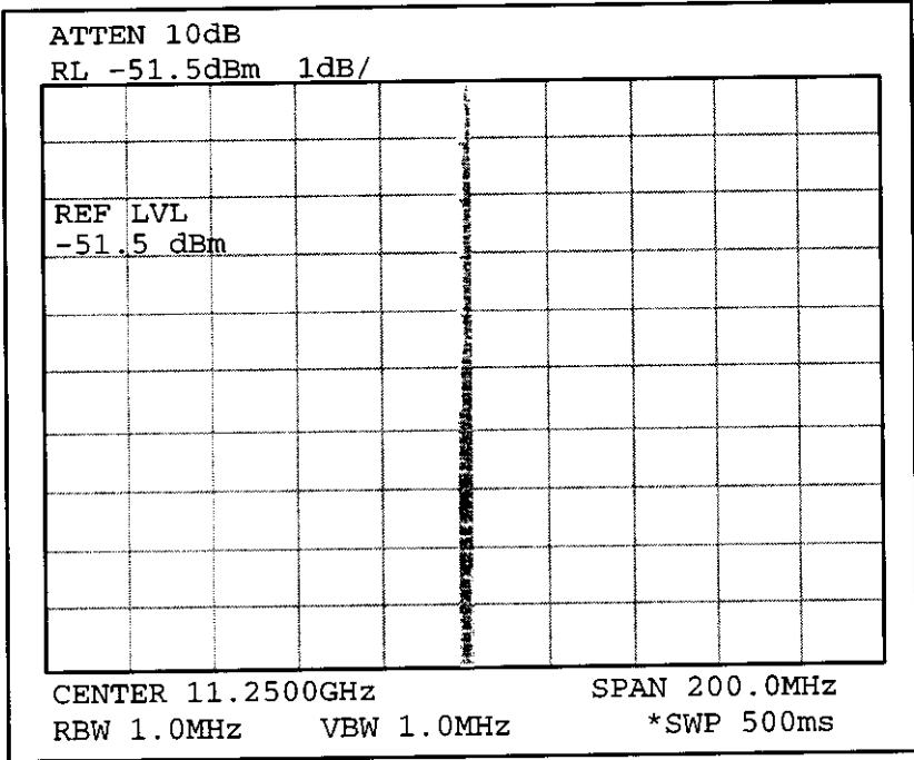
Figure 15. 5.625 GHz Second Harmonic Calibration Factor
