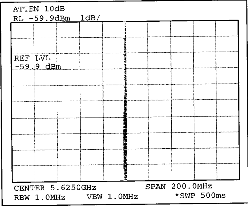
Figure 14. 5.625 GHz First Harmonic Calibration Factor
