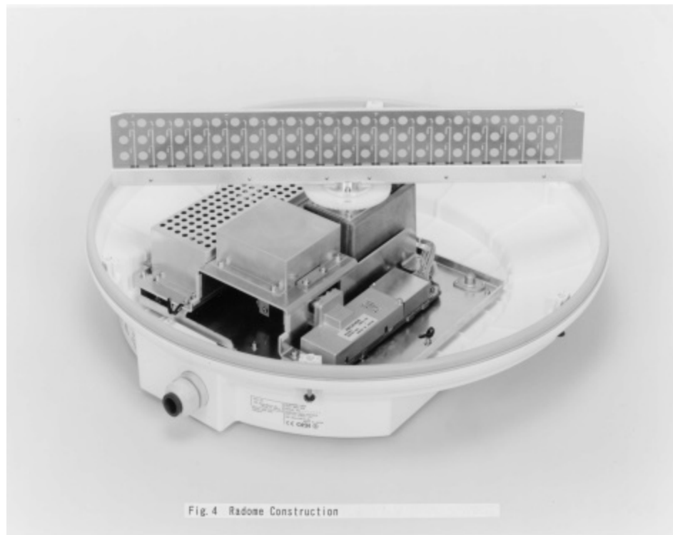
Internal photo of Antenna.
