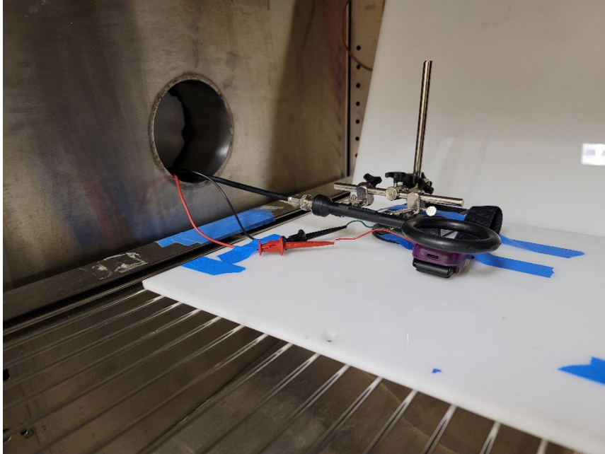
CONFIGURATION 1 - BATTERY
