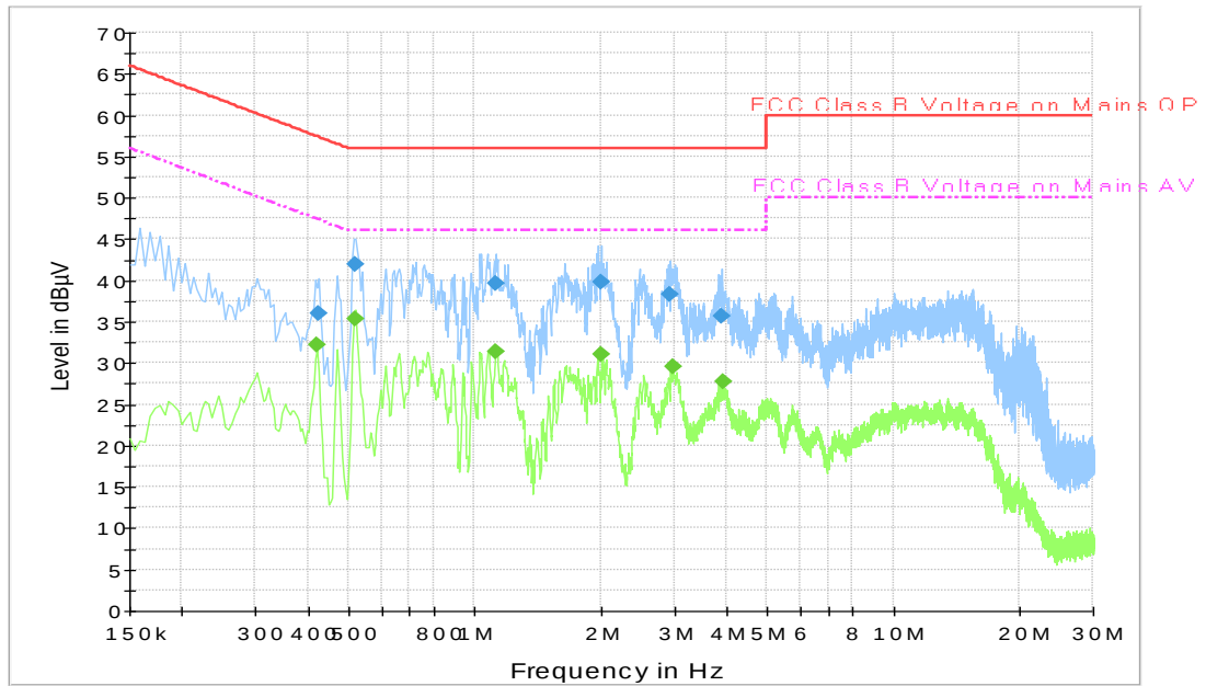
Fig.57 Conducted Emission (802.11a, Ch36, TX)
