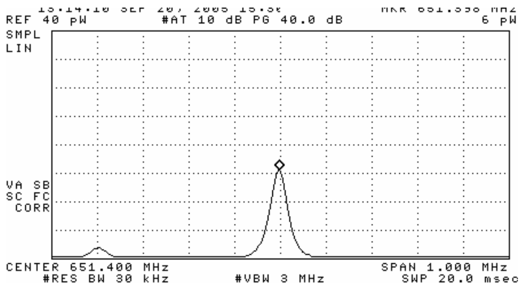
Figure 6.1. Relative receiver emissions (Antenna-Conducted).
