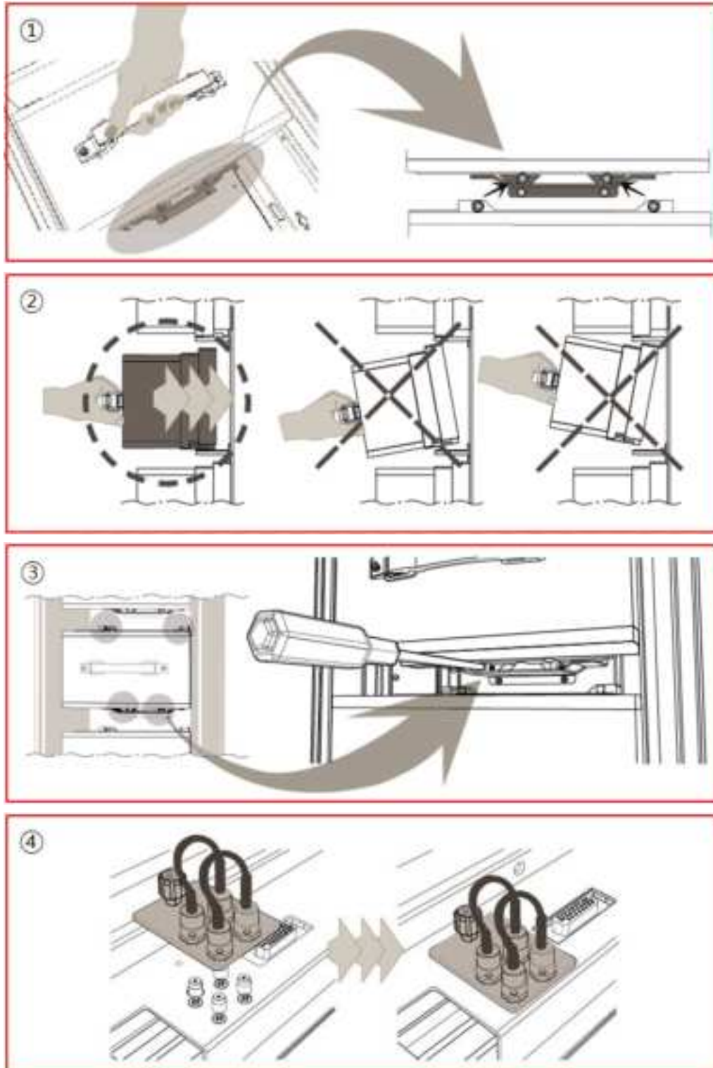
Figure 28.How to mount HRDU
