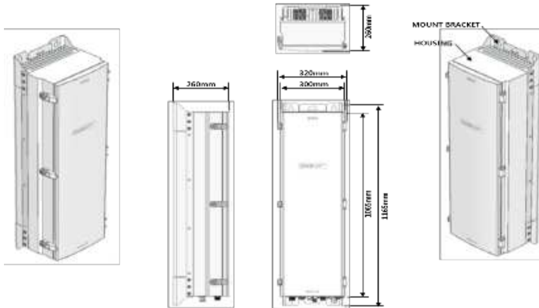
Figure 2. HROU outer Look
