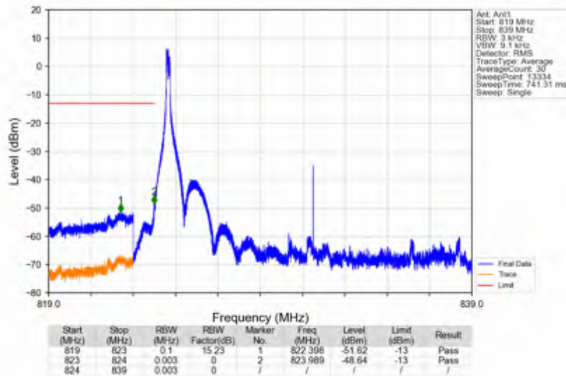
n5 15kHz SISO NTNV 15MHz DFT-s-OFDM PI/2 BPSK 831.5MHz Inner 1RB Left
