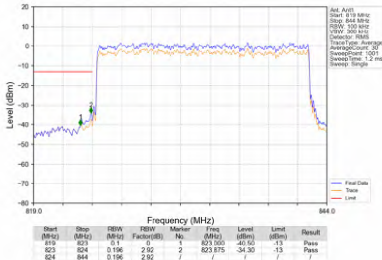
n5_15kHz_SISO_NTNV_20MHz_DFT-s-OFDM QPSK_834MHz_Outer_Full
