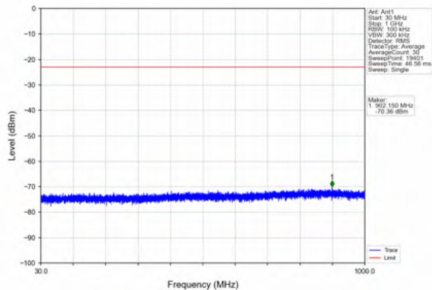
n2_30kHz_SISO_NTNV_20MHz_DFT-s-OFDM_QPSK_1860MHz_Outer_Full
