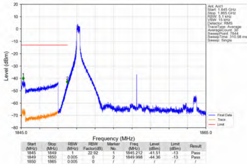
n2_30kHz_SISO_NTNV_15MHz_DFT-s-OFDM QPSK_1857.5MHz_Inner_1RB_Left
