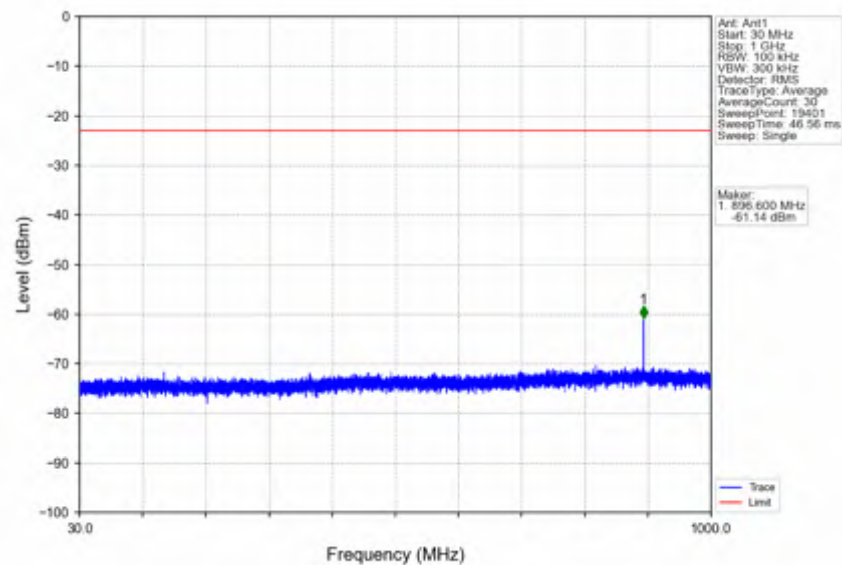
n2_30kHz_SISO_NTNV_20MHz_DFT-s-OFDM PI/2 BPSK_1900MHz_Outer_Full
