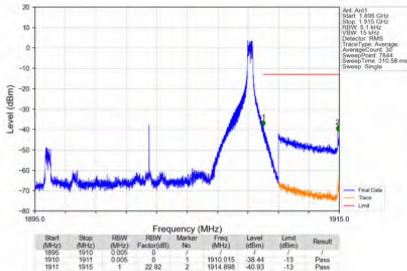
n2_30kHz_SISO_NTNV_15MHz_DFT-s-OFDM QPSK_1902.5MHz_Edge_1RB_Right
