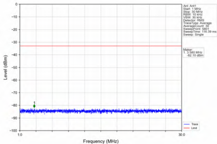
n2_30kHz_SISO_NTNV_15MHz_DFT-s-OFDM QPSK_1902.5MHz_Inner_1RB_Right
