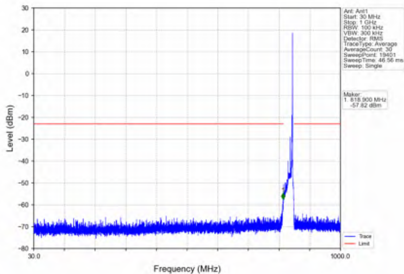
n5_15kHz_SISO_NTNV_15MHz_CP-OFDM_QPSK_841.5MHz_Edge_1RB_Right
