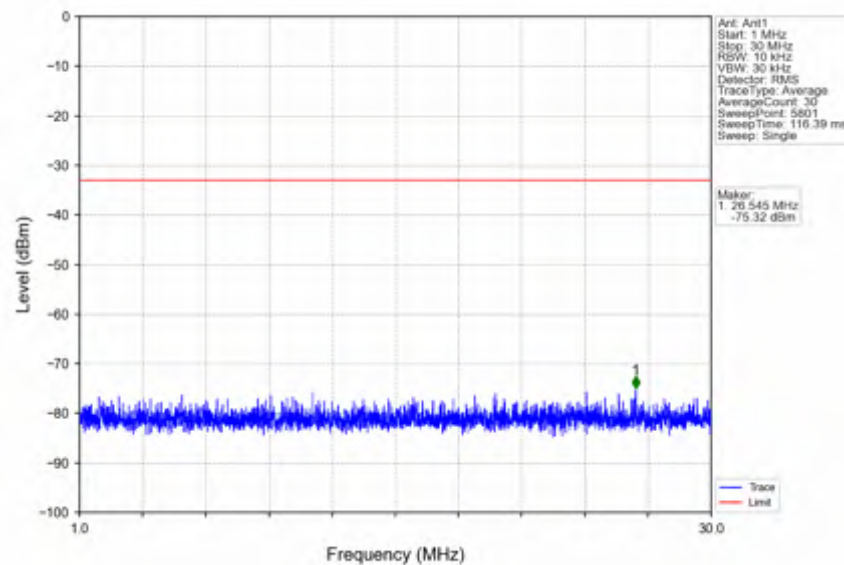
n5_15kHz_SISO_NTNV_5MHz_CP-OFDM QPSK_826.5MHz_Edge_1RB_Left
