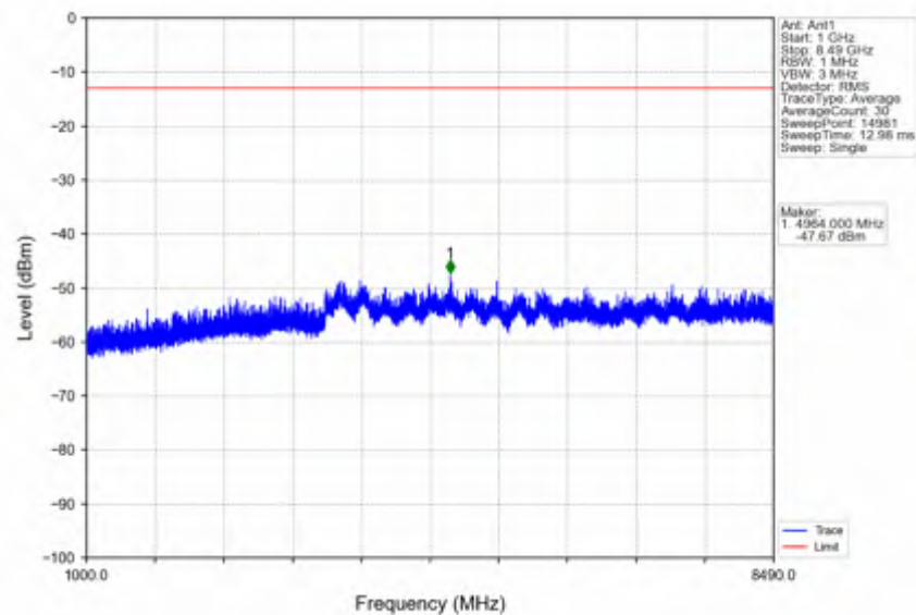
n5_15kHz_SISO_NTNV_10MHz_CP-OFDM QPSK_844MHz_Edge_1RB_Right
