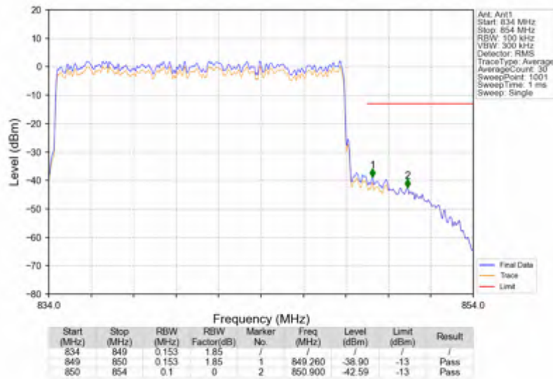
n5_15kHz_SISO_NTNV_15MHz_DFT-s-OFDM QPSK_841.5MHz_Outer_Full
