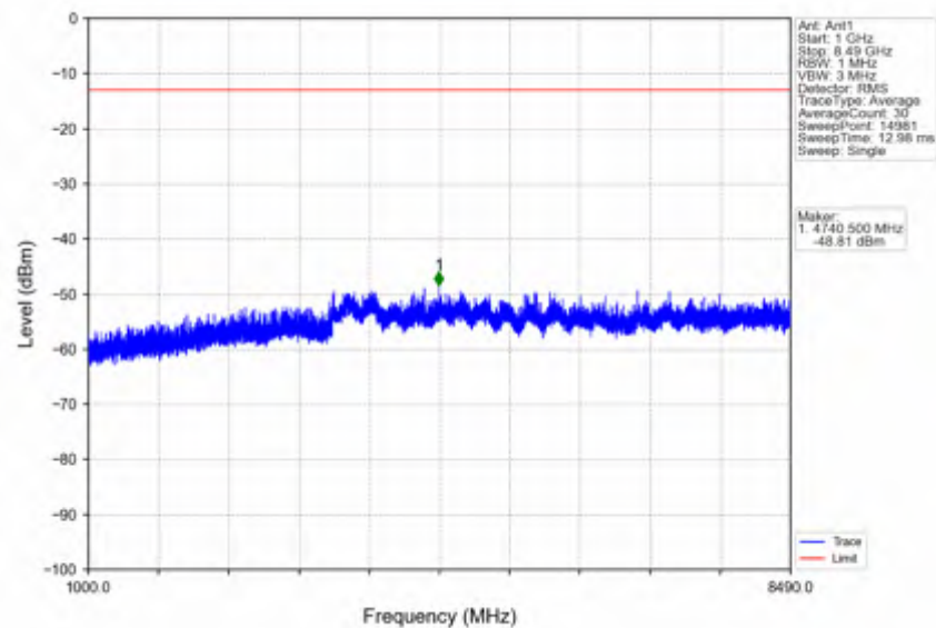
n5_15kHz_SISO_NTNV_10MHz_CP-OFDM QPSK_829MHz_Outer_Full
