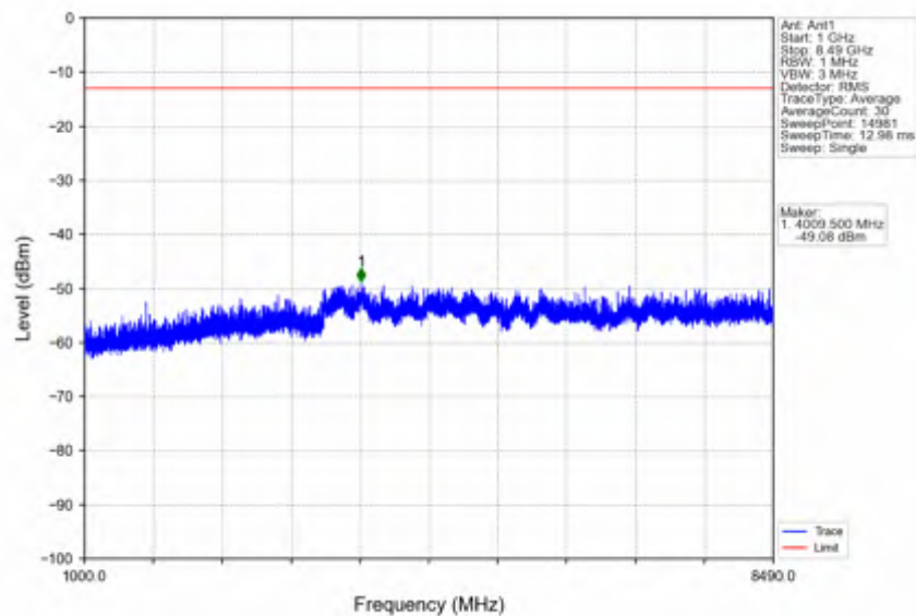
n5_15kHz_SISO_NTNV_5MHz_DFT-s-OFDM QPSK_846.5MHz_Edge_1RB_Right
