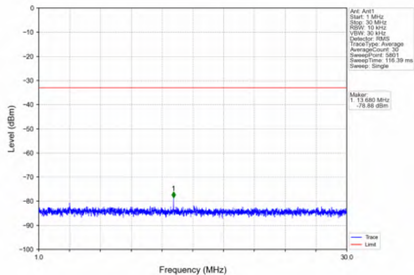
n2_30kHz_SISO_NTNV_20MHz_DFT-s-OFDM_QPSK_1860MHz_Outer_Full
