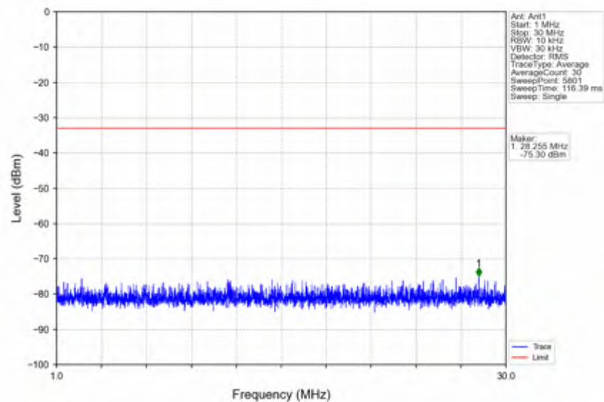
n5_15kHz_SISO_NTNV_5MHz_CP-OFDM QPSK_836.5MHz_Edge_1RB_Left
