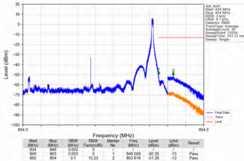
n5_15kHz_SISO_NTNV_15MHz_DFT-s-OFDM QPSK_841.5MHz_Inner_1RB_Right
