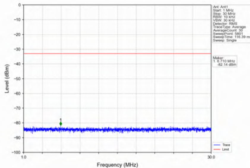
n2_30kHz_SISO_NTNV_15MHz_CP-OFDM QPSK_1902.5MHz_Inner_1RB_Right
