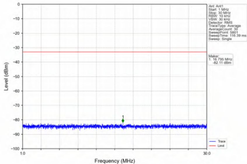
n2_30kHz_SISO_NTNV_20MHz_DFT-s-OFDM_QPSK_1900MHz_Edge_1RB_Right
