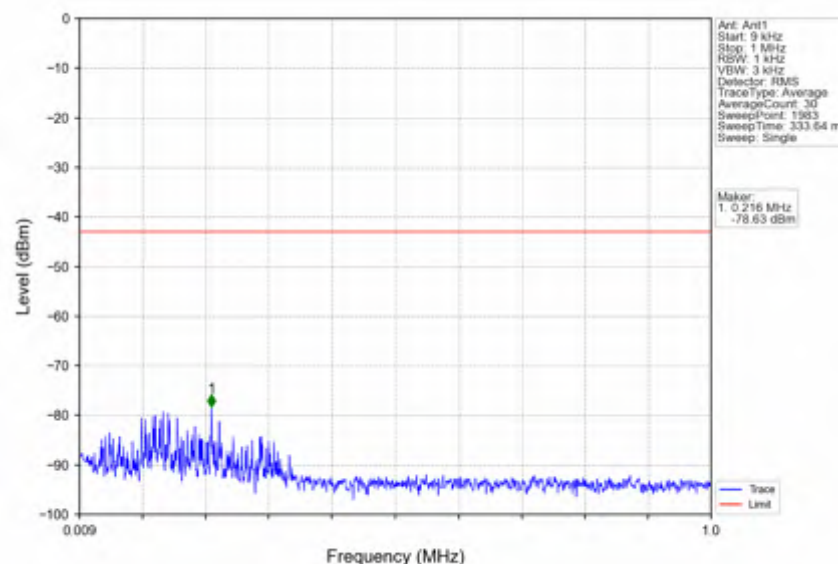
n2 30kHz SISO NTNV 15MHz DFT-s-OFDM QPSK 1880MHz Edge 1RB Left
