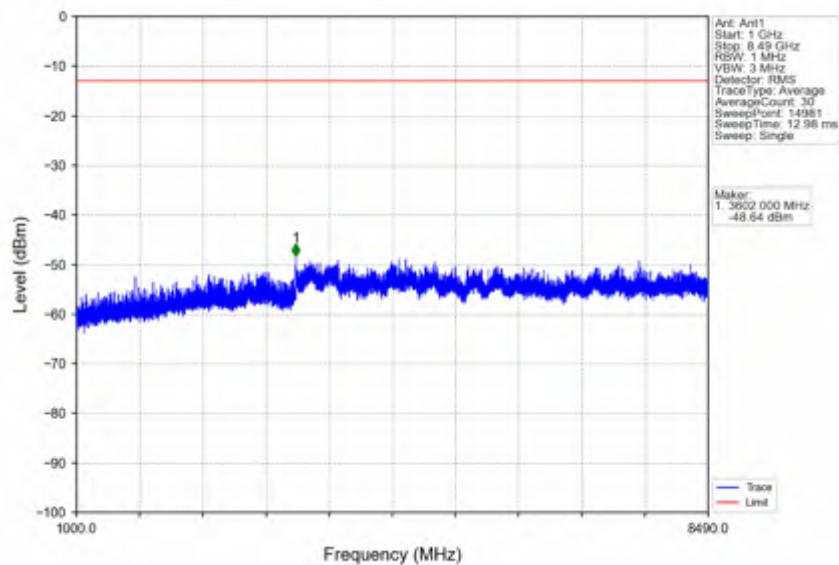
n5_15kHz_SISO_NTNV_20MHz_DFT-s-OFDM_QPSK_839MHz_Edge_1RB_Right
