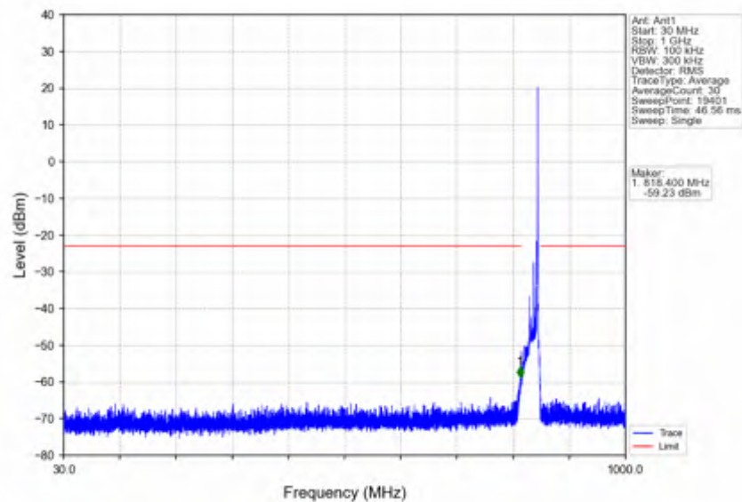
n5_15kHz_SISO_NTNV_15MHz_DFT-s-OFDM_QPSK_841.5MHz_Edge_1RB_Right
