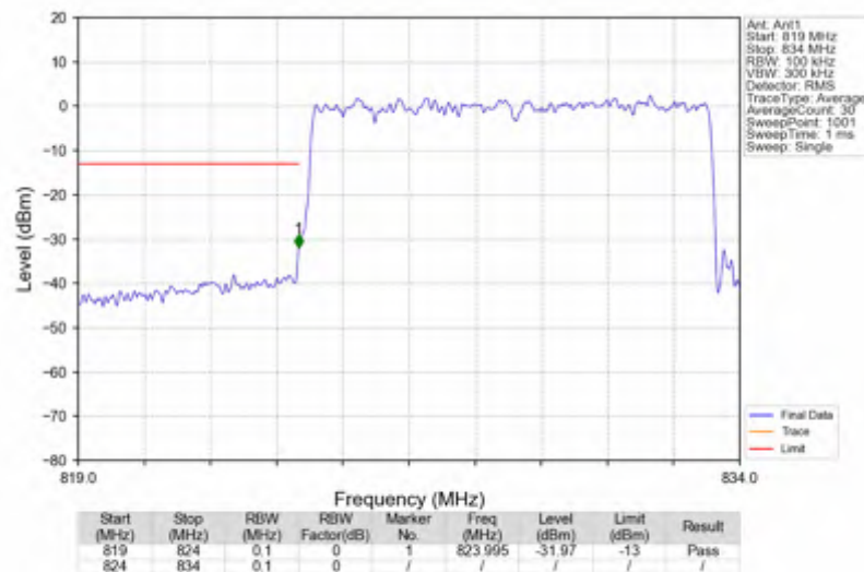
n5_15kHz_SISO_NTNV_10MHz_DFT-s-OFDM QPSK_829MHz_Outer_Full
