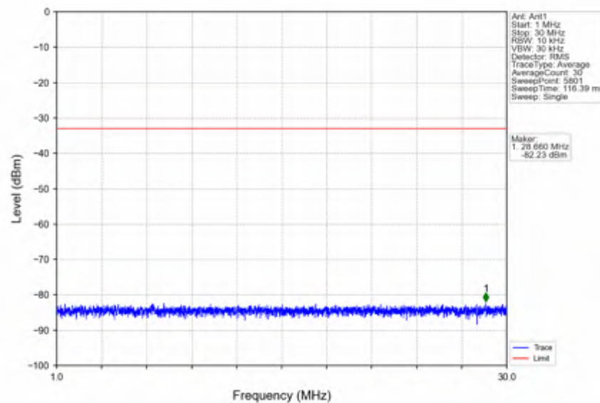
n2_30kHz_SISO_NTNV_15MHz_CP-OFDM_QPSK_1857.5MHz_Inner_1RB_Left
