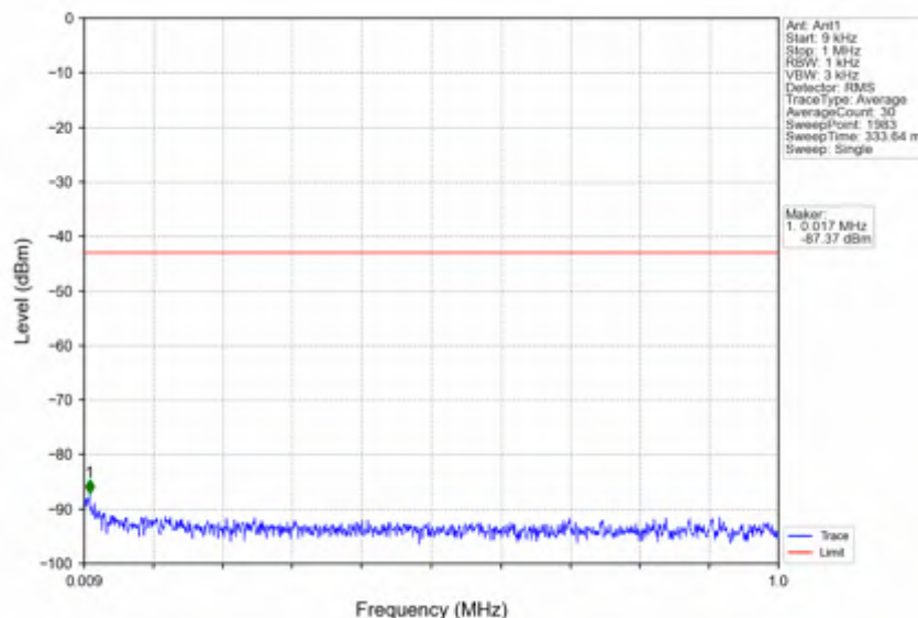
n2_30kHz_SISO_NTNV_15MHz_DFT-s-OFDM_QPSK_1902.5MHz_Outer_Full
