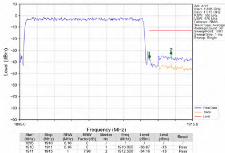
n2_30kHz_SISO_NTNV_15MHz_CP-OFDM QPSK_1902.5MHz_Outer_Full
