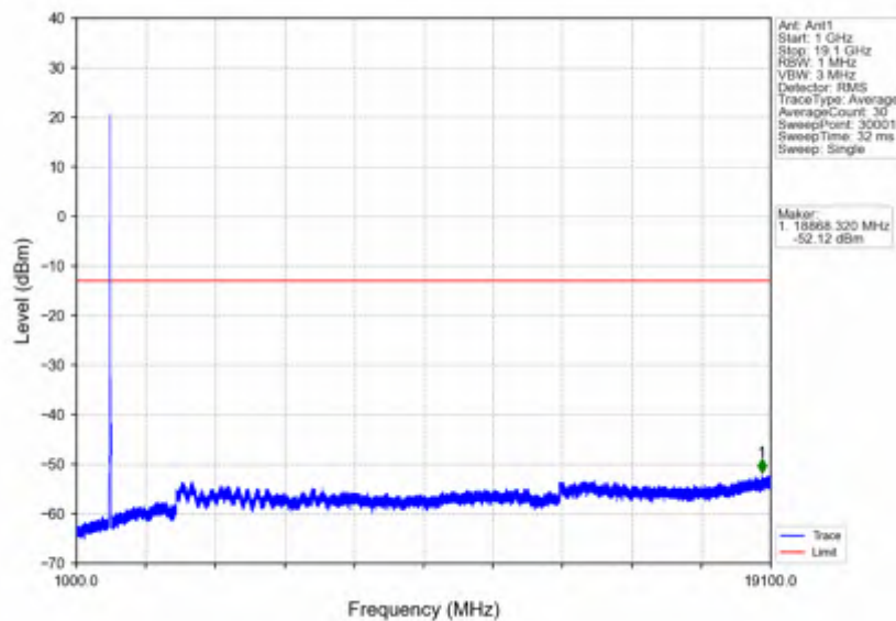
n2_30kHz_SISO_NTNV_15MHz_DFT-s-OFDM QPSK_1902.5MHz_Edge_1RB_Right
