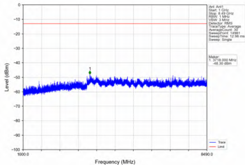
n5_15kHz_SISO_NTNV_10MHz_DFT-s-OFDM QPSK_829MHz_Outer_Full
