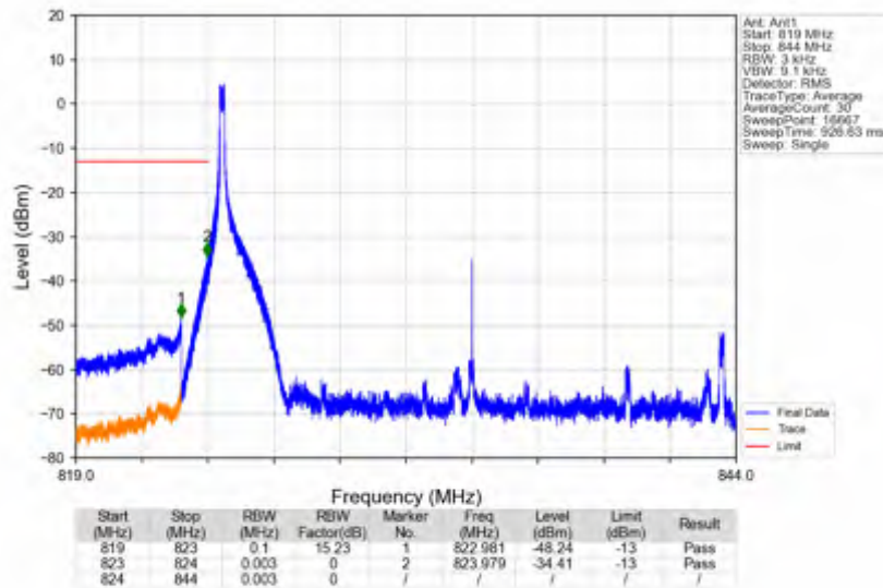
n5_15kHz_SISO_NTNV_20MHz_DFT-s-OFDM_QPSK_834MHz_Edge_1RB_Left
