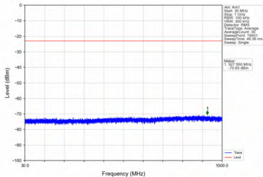
n2_30kHz_SISO_NTNV_15MHz_DFT-s-OFDM_QPSK_1902.5MHz_Inner_1RB_Right
