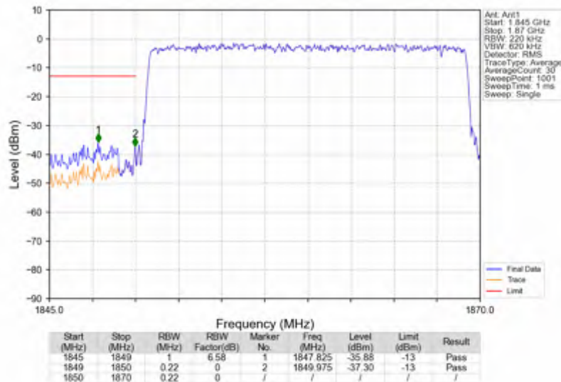
n2_30kHz_SISO_NTNV_20MHz_CP-OFDM QPSK_1860MHz_Outer_Full
