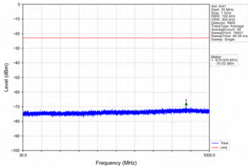
n2_30kHz_SISO_NTNV_20MHz_CP-OFDM_QPSK_1860MHz_Outer_Full
