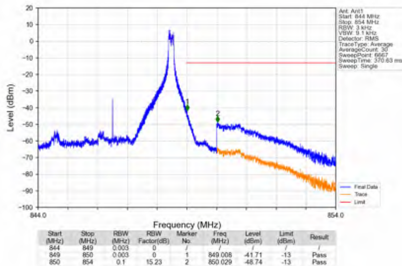
n5_15kHz_SISO_NTNV_5MHz_DFT-s-OFDM QPSK_846.5MHz_Inner_1RB_Right
