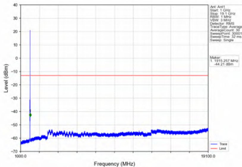
n2_30kHz_SISO_NTNV_20MHz_DFT-s-OFDM_PI/2_BPSK_1900MHz_Outer_Full
