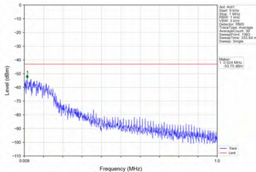
n5_15kHz_SISO_NTNV_10MHz_CP-OFDM_QPSK_829MHz_Edge_1RB_Left
