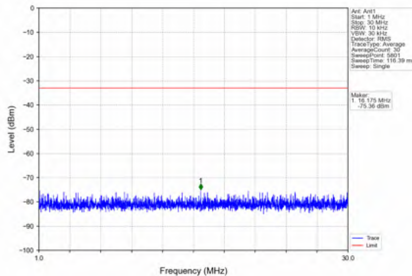
n5_15kHz_SISO_NTNV_20MHz_DFT-s-OFDM_QPSK_836.5MHz_Edge_1RB_Left
