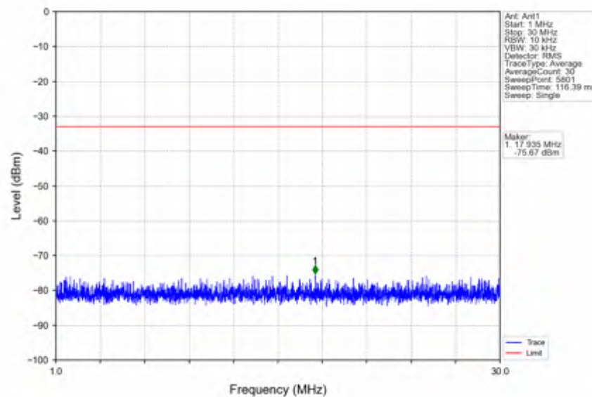
n5_15kHz_SISO_NTNV_10MHz_DFT-s-OFDM QPSK_829MHz_Edge_1RB_Left
