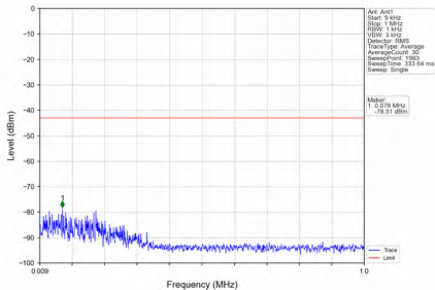
n2_30kHz_SISO_NTNV_15MHz_CP-OFDM QPSK_1880MHz_Edge_1RB_Left
