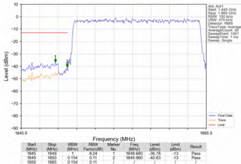
n2_30kHz_SISO_NTNV_15MHz_CP-OFDM QPSK_1857.5MHz_Outer_Full
