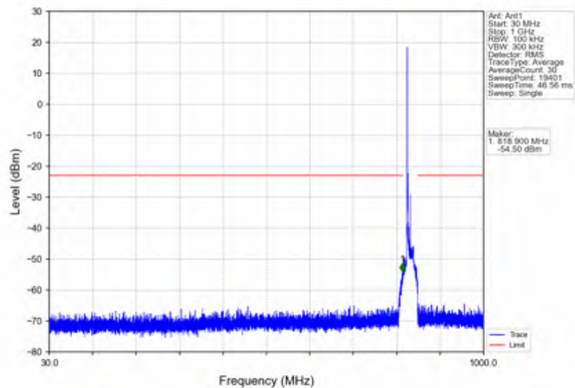
n5_15kHz_SISO_NTNV_15MHz_CP-OFDM_QPSK_836.5MHz_Edge_1RB_Left
