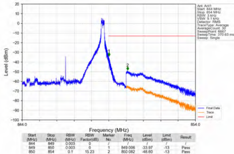
n5_15kHz_SISO_NTNV_5MHz_DFT-s-OFDM QPSK_846.5MHz_Edge_1RB_Right
