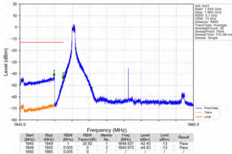
n2 30kHz SISO NTNv 15MHz CP-OFDM QPSK 1857.5MHz Inner 1RB Left
