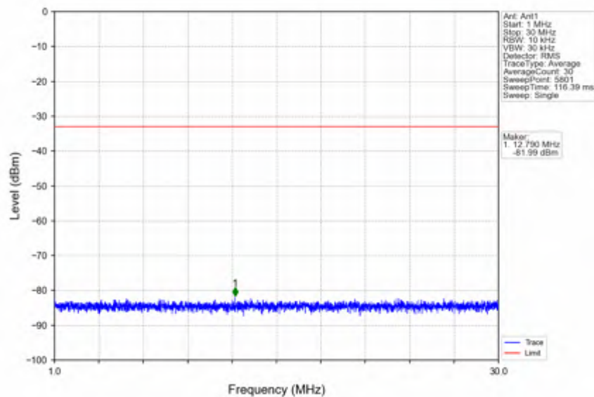
n2_30kHz_SISO_NTNV_15MHz_CP-OFDM_QPSK_1902.5MHz_Edge_1RB_Right
