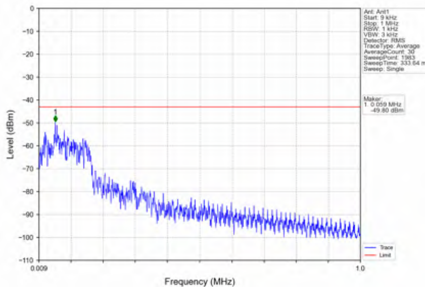
n5_15kHz_SISO_NTNV_10MHz_DFT-s-OFDM_QPSK_829MHz_Edge_1RB_Left
