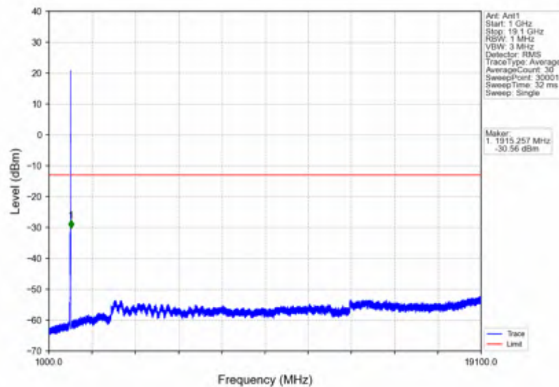
n2_30kHz_SISO_NTNV_15MHz_DFT-s-OFDM_QPSK_1902.5MHz_Inner_1RB_Right
