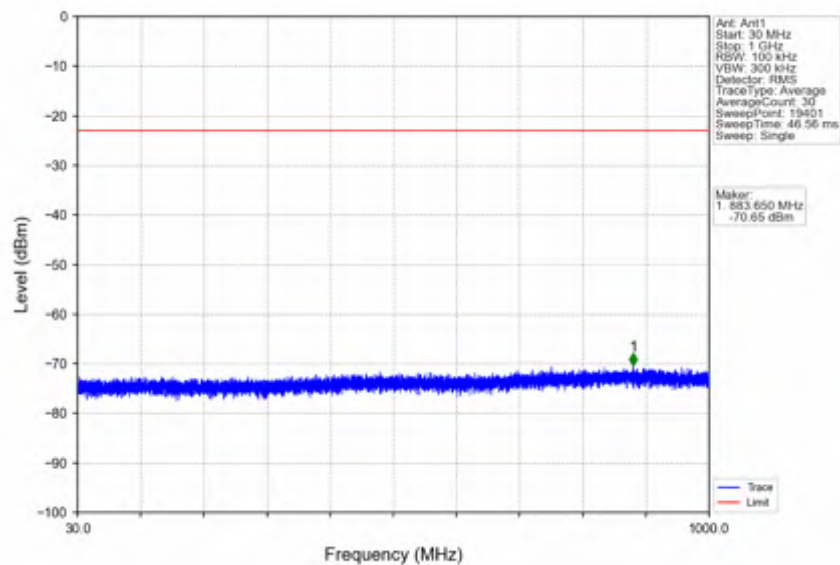
n2_30kHz_SISO_NTNV_15MHz_CP-OFDM QPSK_1857.5MHz_Outer_Full
