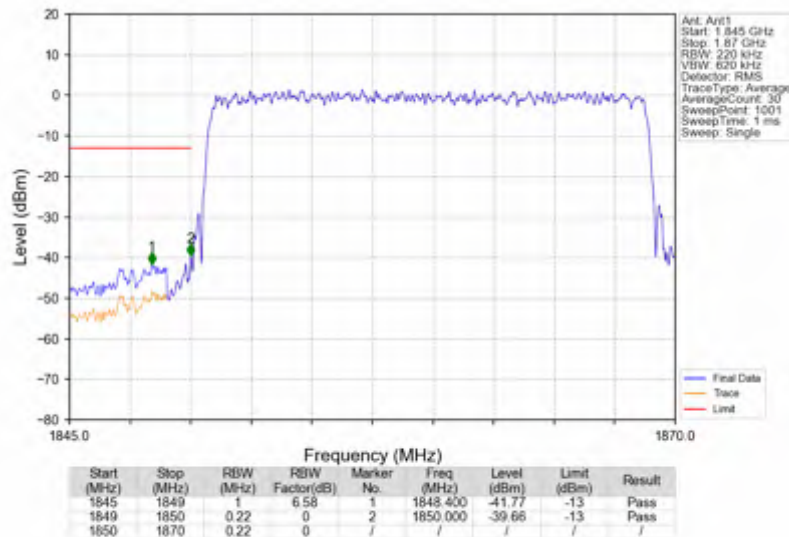
n2_30kHz_SISO_NTNV_20MHz_DFT-s-OFDM PI/2 BPSK_1860MHz_Outer_Full
