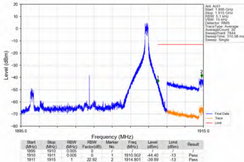
n2_30kHz_SISO_NTNV_15MHz_DFT-s-OFDM QPSK_1902.5MHz_Inner_1RB_Right
