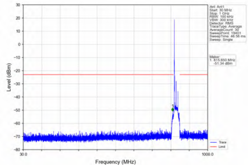
n5_15kHz_SISO_NTNV_20MHz_CP-OFDM_QPSK_834MHz_Edge_1RB_Left
