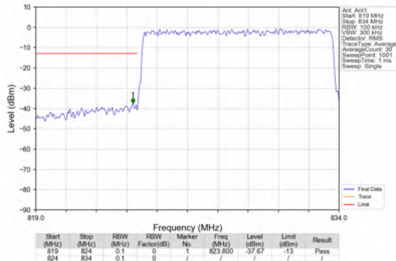
n5_15kHz_SISO_NTNV_10MHz_CP-OFDM QPSK_829MHz_Outer_Full
