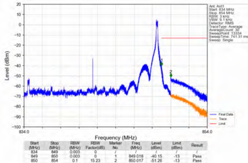
n5_15kHz_SISO_NTNV_15MHz_DFT-s-OFDM QPSK_841.5MHz_Edge_1RB_Right
