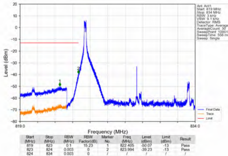
n5_15kHz_SISO_NTNV_10MHz_DFT-s-OFDM QPSK_829MHz_Inner_1RB_Left
