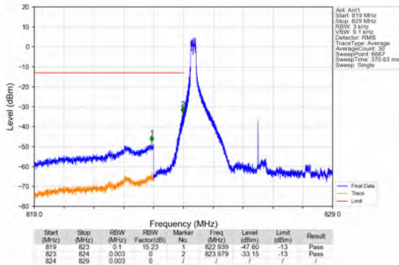
n5_15kHz_SISO_NTNV_5MHz_DFT-s-OFDM QPSK 826.5MHz_Edge_1RB_Left
