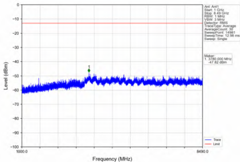
n5_15kHz_SISO_NTNV_10MHz_DFT-s-OFDM_QPSK_844MHz_Edge_1RB_Right
