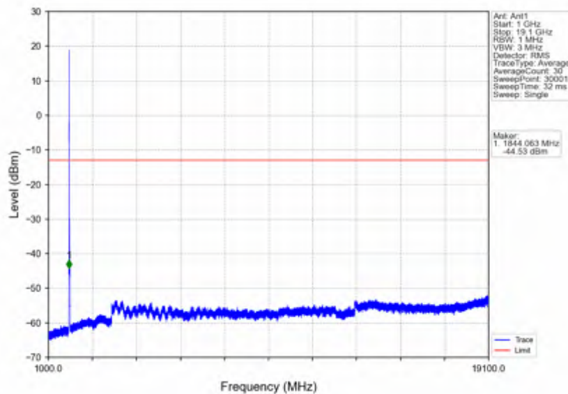
n2_30kHz_SISO_NTNV_15MHz_CP-OFDM QPSK_1857.5MHz_Outer_Full
