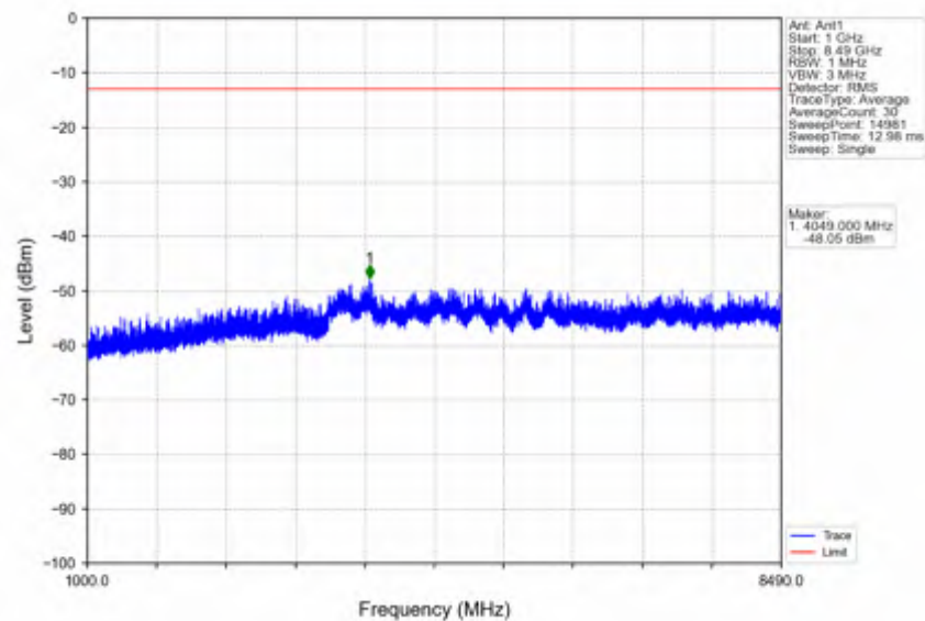
n5_15kHz_SISO_NTNV_15MHz_DFT-s-OFDM QPSK_831.5MHz_Outer_Full
