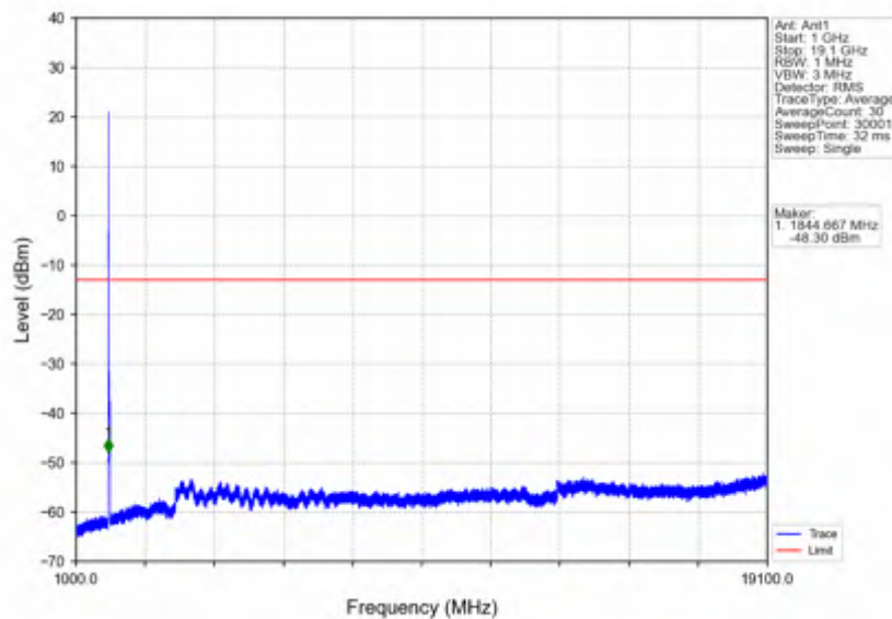
n2_30kHz_SISO_NTNV_20MHz_DFT-s-OFDM PI/2 BPSK_1860MHz_Outer_Full
