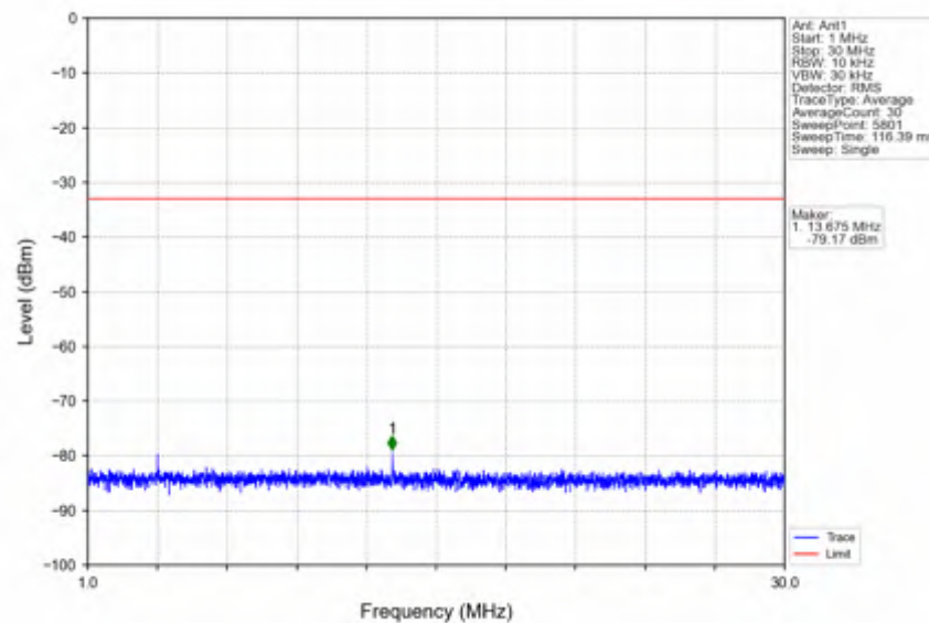
n2_30kHz_SISO_NTNV_20MHz_DFT-s-OFDM_QPSK_1900MHz_Outer_Full
