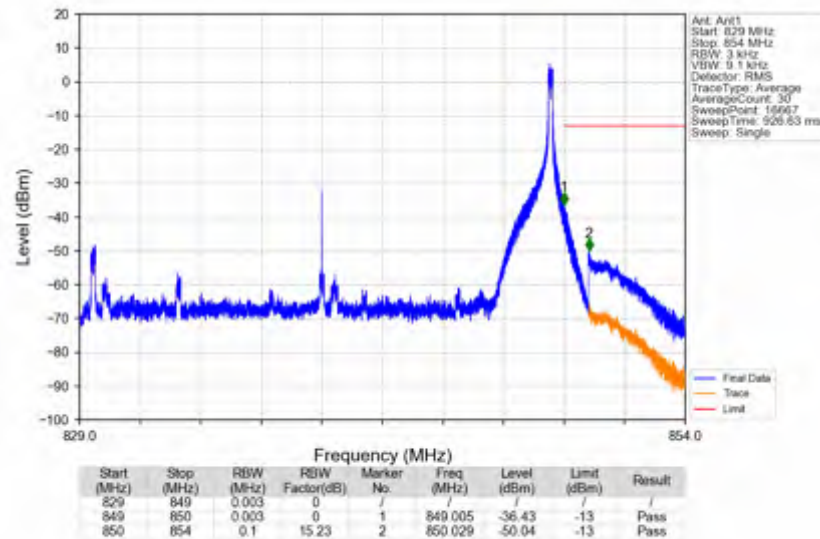
n5_15kHz_SISO_NTNV_20MHz_DFT-s-OFDM_QPSK_839MHz_Edge_1RB_Right
