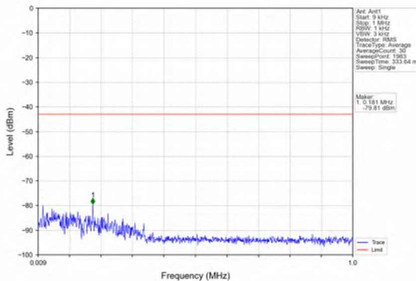
n2_30kHz_SISO_NTNV_15MHz_CP-OFDM_QPSK_1902.5MHz_Edge_1RB_Right
