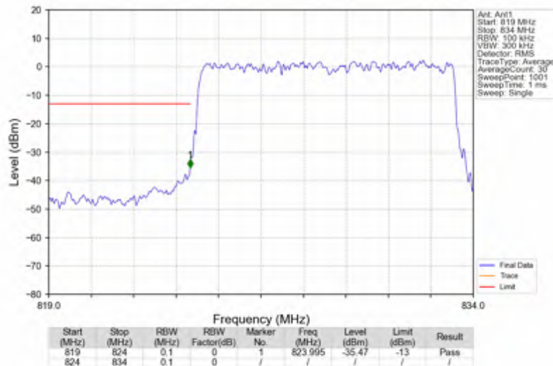
n5_15kHz_SISO_NTNV_10MHz_DFT-s-OFDM PI/2 BPSK_829MHz_Outer_Full
