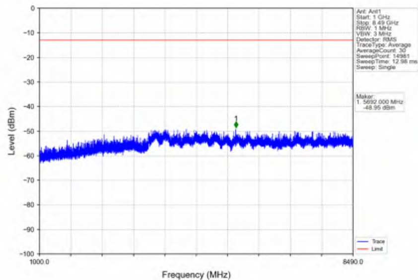
n5_15kHz_SISO_NTNV_10MHz_DFT-s-OFDM QPSK_844MHz_Edge_1RB_Right
