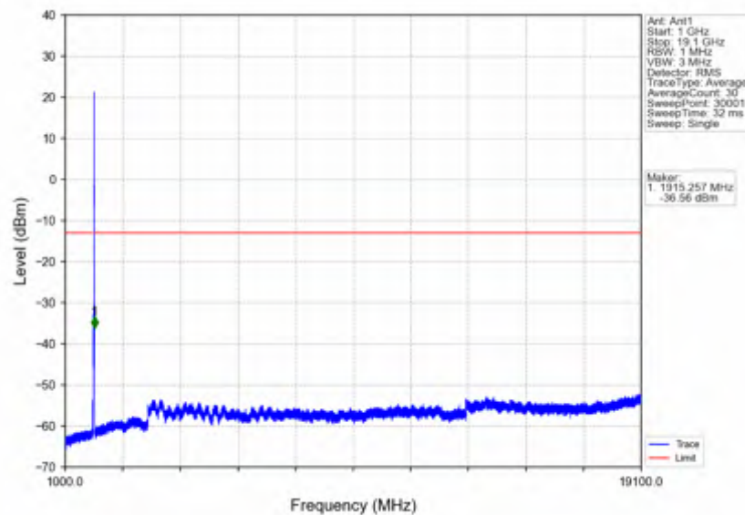
n2_30kHz_SISO_NTV_15MHz_DFT-s-OFDM_QPSK_1902.5MHz_Edge_1RB_Right
