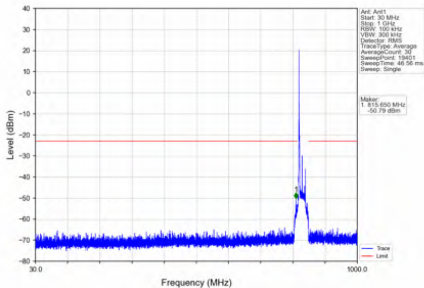
n5_15kHz_SISO_NTNV_20MHz_DFT-s-OFDM QPSK_834MHz_Edge_1RB_Left
