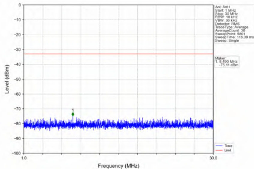
n5_15kHz_SISO_NTNV_10MHz_DFT-s-OFDM_QPSK_836.5MHz_Edge_1RB_Left
