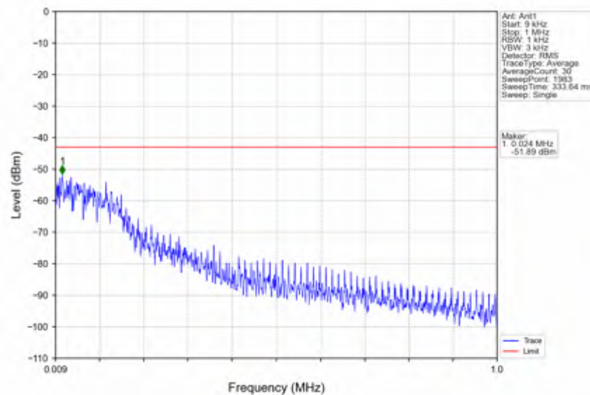
n5_15kHz_SISO_NTNV_15MHz_CP-OFDM QPSK_841.5MHz_Edge_1RB_Right
