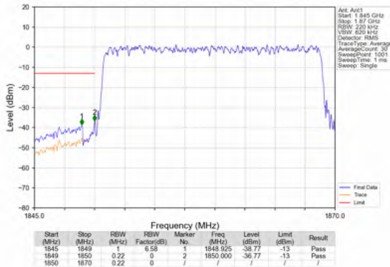
n2_30kHz_SISO_NTNV_20MHz_DFT-s-OFDM_QPSK_1860MHz_Outer_Full
