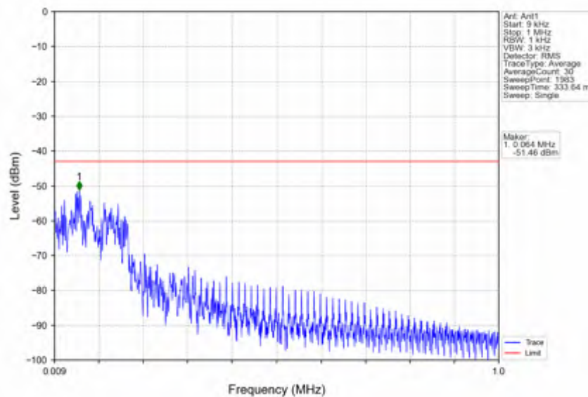
n5_15kHz_SISO_NTNV_15MHz_DFT-s-OFDM_PI/2_BPSK_836.5MHz_Edge_1RB_Left
