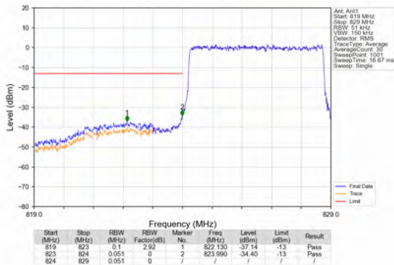
n5_15kHz_SISO_NTNV_5MHz_DFT-s-OFDM QPSK_826.5MHz_Outer_Full
