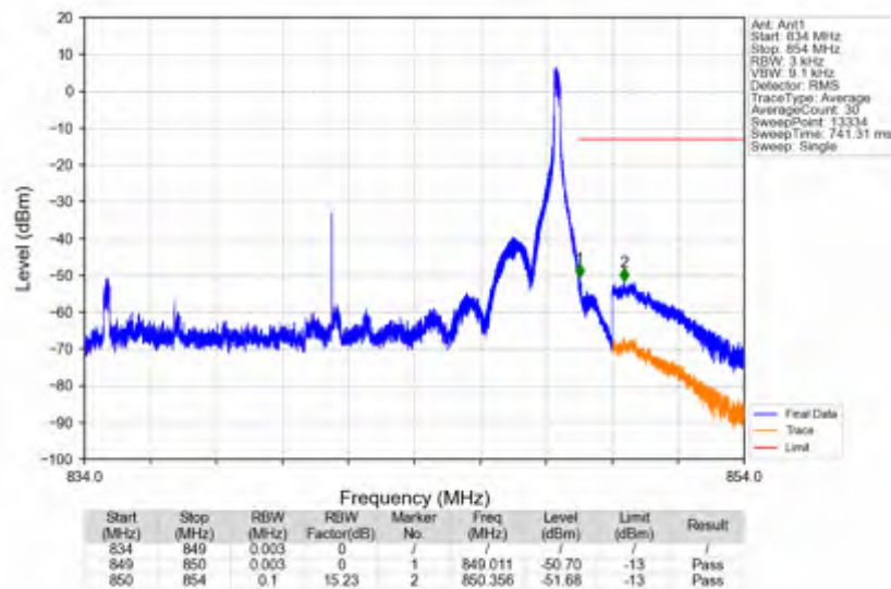
n5_15kHz_SISO_NTNV_15MHz_DFT-s-OFDM PI/2 BPSK_841.5MHz_Inner_1RB_Right
