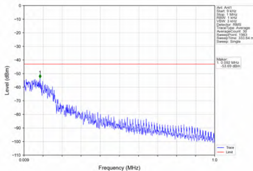
n5_15kHz_SISO_NTNV_10MHz_CP-OFDM QPSK_836.5MHz_Edge_1RB_Left
