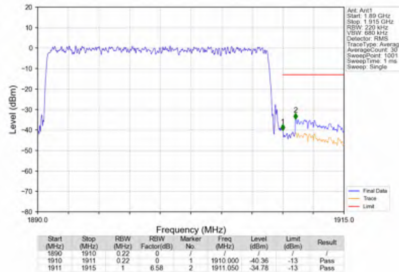
n2_30kHz_SISO_NTNV_20MHz_DFT-s-OFDM_QPSK_1900MHz_Outer_Full
