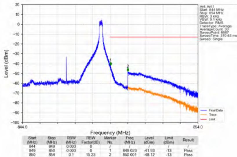
n5_15kHz_SISO_NTNV_5MHz_CP-OFDM QPSK_846.5MHz_Inner_1RB_Right
