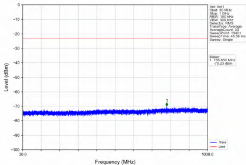
n2_30kHz_SISO_NTNV_15MHz_CP-OFDM QPSK_1880MHz_Edge_1RB_Left
