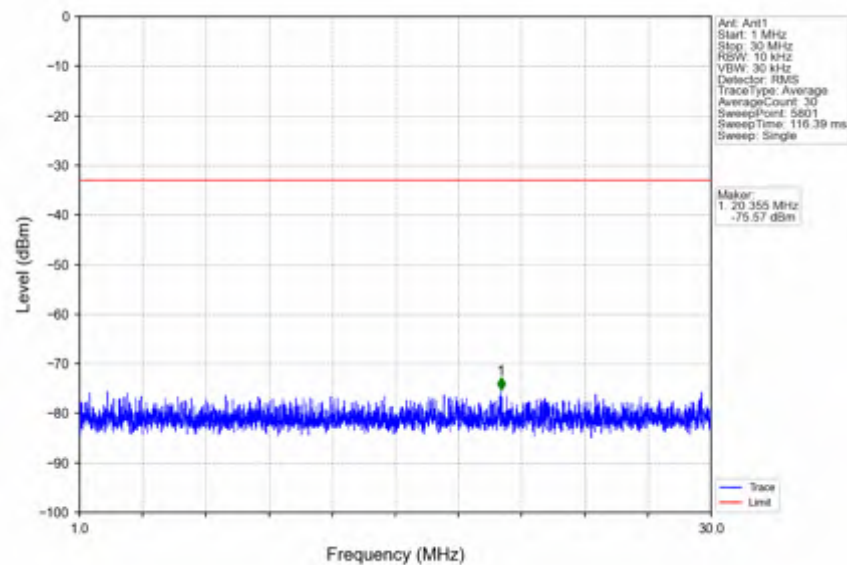
n5_15kHz_SISO_NTNV_10MHz_DFT-s-OFDM_QPSK_844MHz_Edge_1RB_Right
