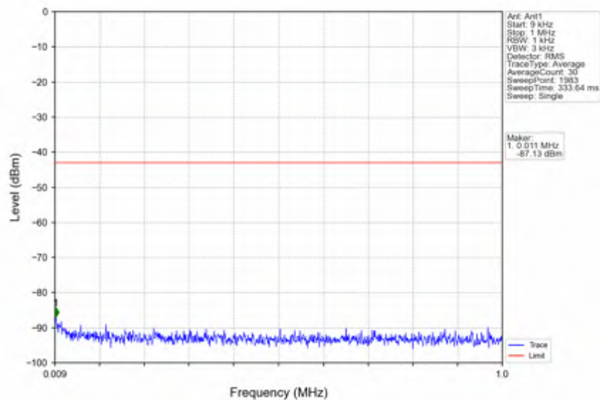
n2 30kHz SISO NTNV 15MHz CP-OFDM QPSK 1857.5MHz Outer Full
