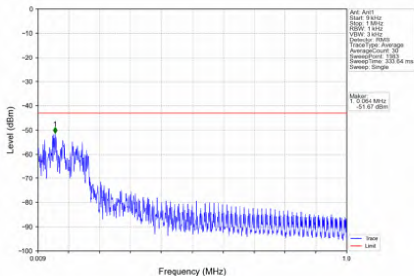
n5_15kHz_SISO_NTNV_20MHz_DFT-s-OFDM_PI/2_BPSK_834MHz_Edge_1RB_Left
