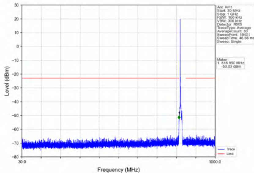
n5_15kHz_SISO_NTNV_5MHz_CP-OFDM QPSK_826.5MHz_Edge_1RB_Left
