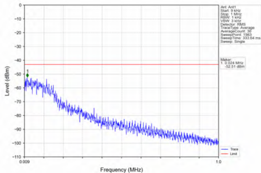
n5_15kHz_SISO_NTNV_5MHz_CP-OFDM_QPSK_846.5MHz_Edge_1RB_Right
