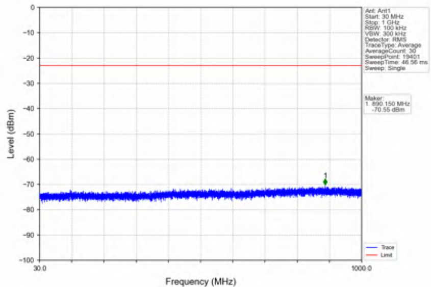
n2_30kHz_SISO_NTNV_15MHz_DFT-s-OFDM QPSK_1880MHz_Edge_1RB_Left
