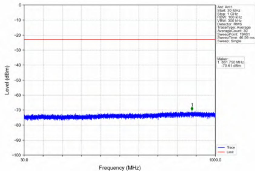
n2_30kHz_SISO_NTV_15MHz_DFT-s-OFDM_QPSK_1902.5MHz_Edge_1RB_Right
