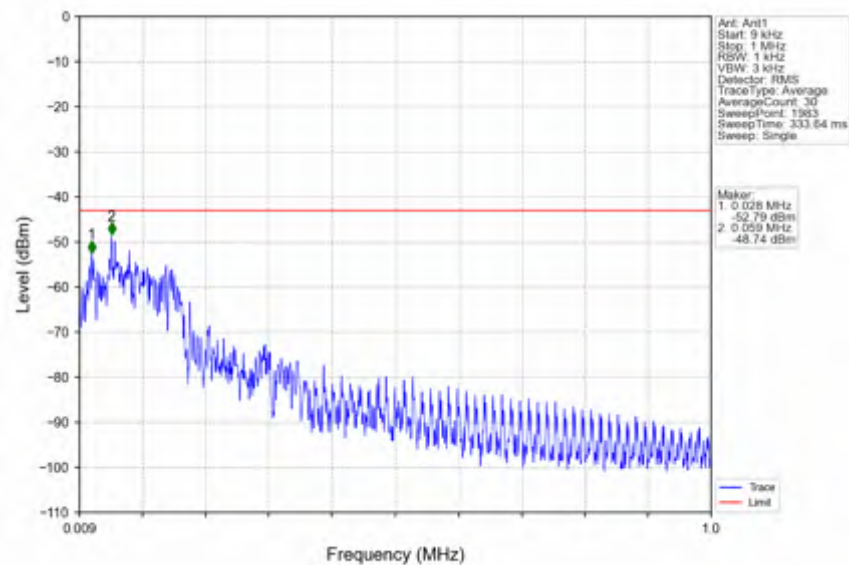
n5_15kHz_SISO_NTNV_15MHz_DFT-s-OFDM QPSK 841.5MHz_Edge_1RB_Right
