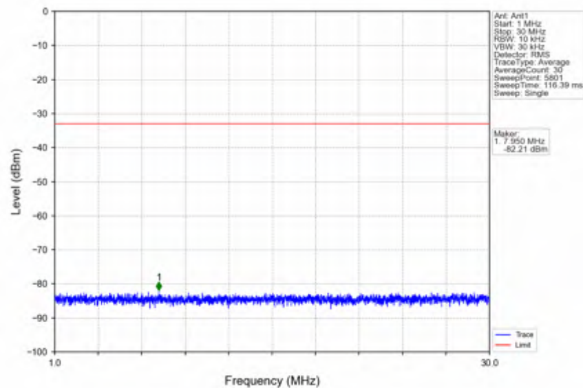
n2_30kHz_SISO_NTNV_20MHz_CP-OFDM QPSK_1900MHz_Edge_1RB_Right
