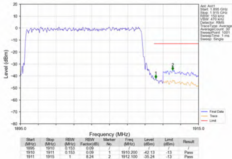
n2_30kHz_SISO_NTNV_15MHz_DFT-s-OFDM_QPSK_1902.5MHz_Outer_Full
