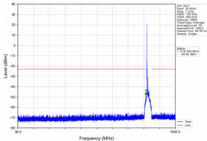
n5_15kHz_SISO_NTNV_15MHz_DFT-s-OFDM_QPSK_831.5MHz_Edge_1RB_Left
