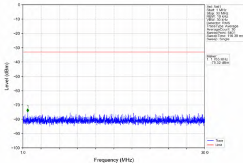
n5_15kHz_SISO_NTNV_15MHz_DFT-s-OFDM_QPSK_831.5MHz_Edge_1RB_Left
