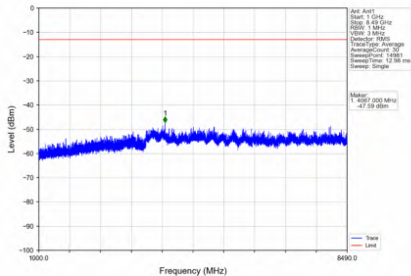
n5_15kHz_SISO_NTNV_20MHz_DFT-s-OFDM_QPSK_839MHz_Edge_1RB_Right
