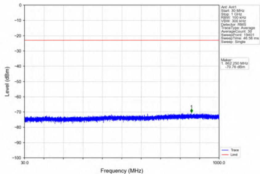
n2_30kHz_SISO_NTNV_15MHz_CP-OFDM QPSK_1857.5MHz_Edge_1RB_Left
