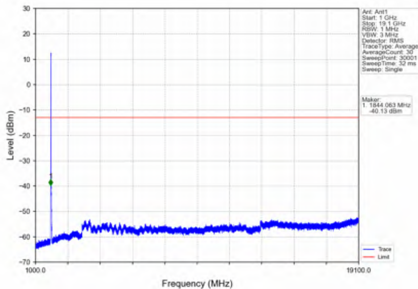
n2_30kHz_SISO_NTNV_15MHz_DFT-s-OFDM QPSK_1857.5MHz_Inner_1RB_Left
