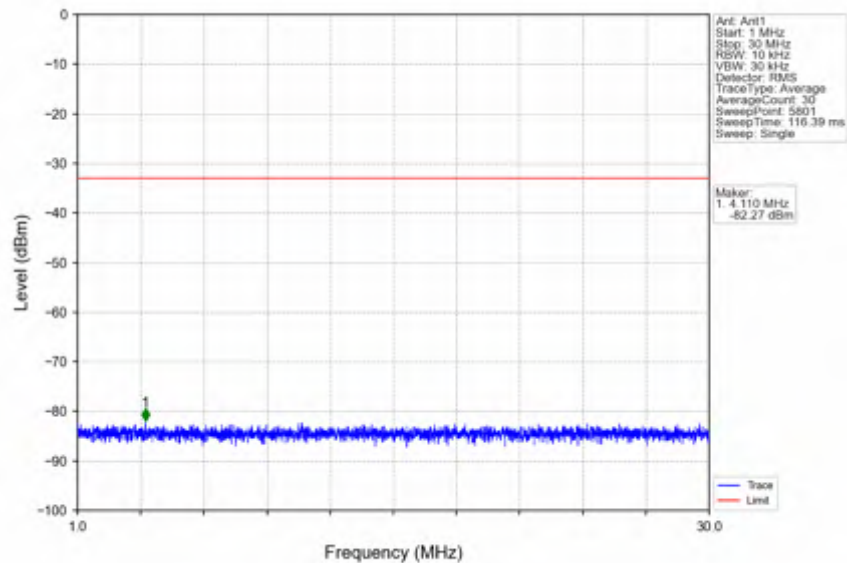
n2_30kHz_SISO_NTV_15MHz_DFT-s-OFDM_QPSK_1902.5MHz_Edge_1RB_Right
