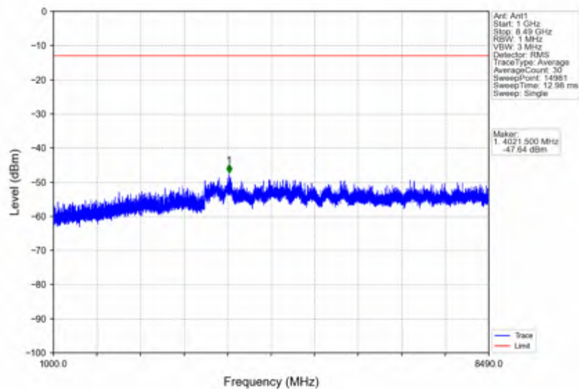
n5_15kHz_SISO_NTNV_5MHz_CP-OFDM QPSK_826.5MHz_Outer_Full
