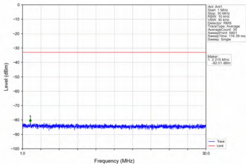
n2_30kHz_SISO_NTNV_20MHz_CP-OFDM_QPSK_1860MHz_Outer_Full
