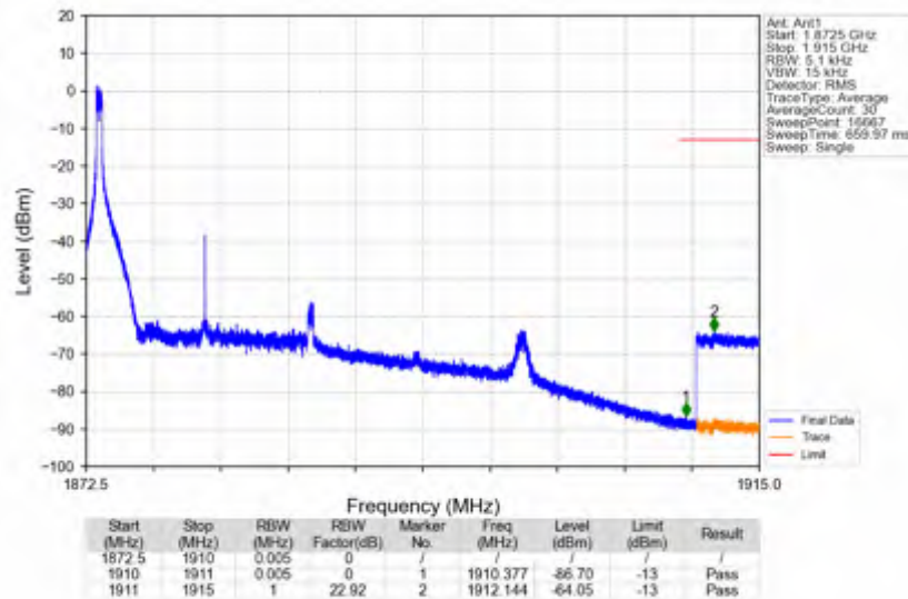
n2_30kHz_SISO_NTNV_15MHz_CP-OFDM QPSK_1880MHz_Edge_1RB_Left
