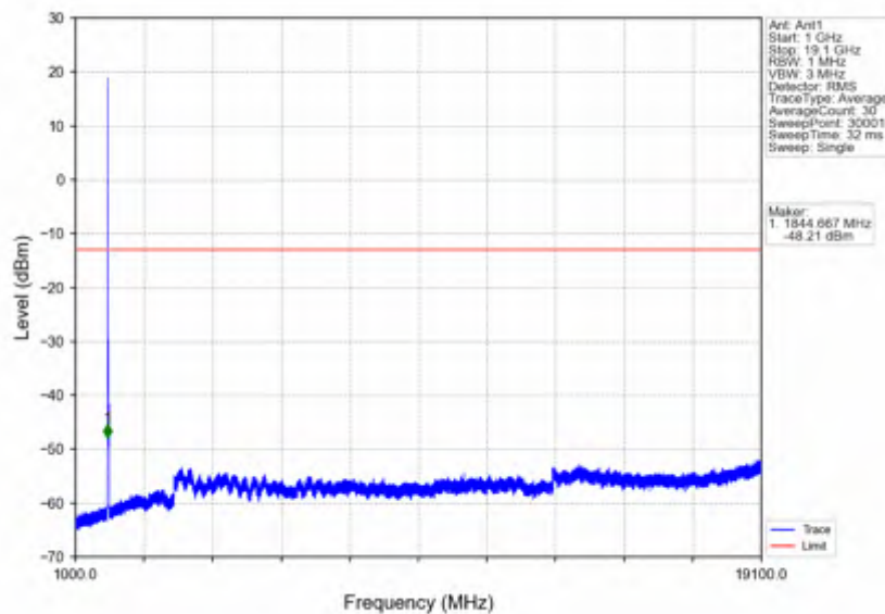
n2_30kHz_SISO_NTNV_20MHz_CP-OFDM QPSK_1860MHz_Outer_Full
