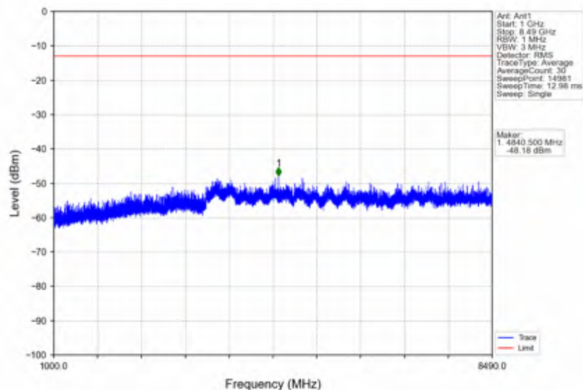
n5_15kHz_SISO_NTNV_5MHz_CP-OFDM QPSK_846.5MHz_Edge_1RB_Right
