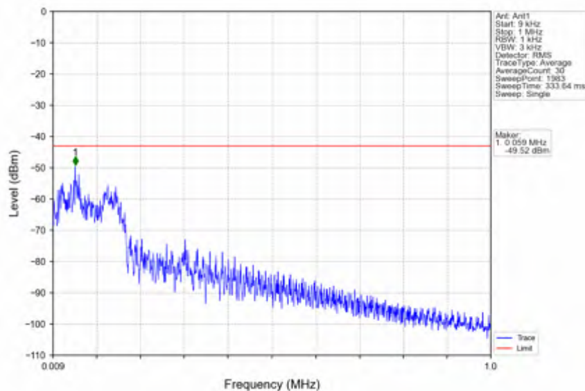
n5_15kHz_SISO_NTNV_5MHz_DFT-s-OFDM_PI/2_BPSK_826.5MHz_Edge_1RB_Left
