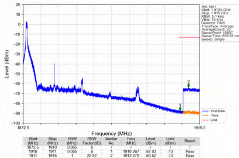
n2 30kHz SISO NTN 15MHz DFT-s-OFDM QPSK 1880MHz Edge 1RB Left
