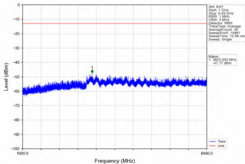
n5_15kHz_SISO_NTNV_5MHz_DFT-s-OFDM QPSK_826.5MHz_Outer_Full
