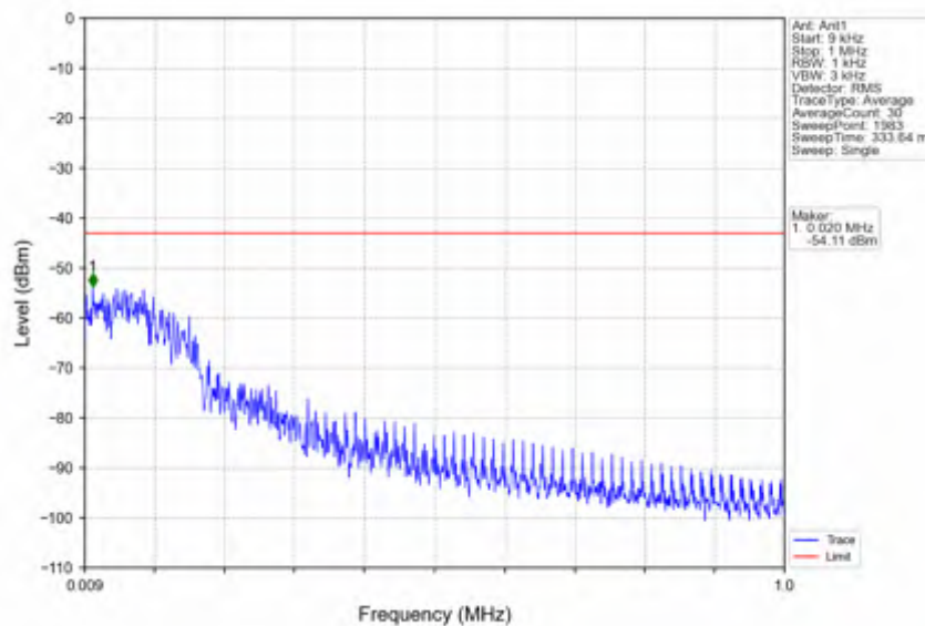
n5_15kHz_SISO_NTV_15MHz_CP-OFDM_QPSK_836.5MHz_Edge_1RB_Left
