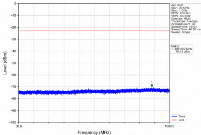
n2_30kHz_SISO_NTNV_20MHz_CP-OFDM_QPSK_1900MHz_Outer_Full
