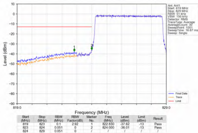
n5_15kHz_SISO_NTNV_5MHz_CP-OFDM QPSK_826.5MHz_Outer_Full
