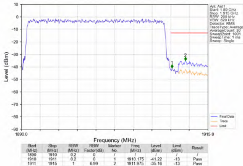
n2_30kHz_SISO_NTNV_20MHz_CP-OFDM QPSK_1900MHz_Outer_Full
