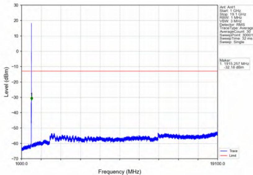
n2_30kHz_SISO_NTNV_20MHz_CP-OFDM QPSK_1900MHz_Outer_Full
