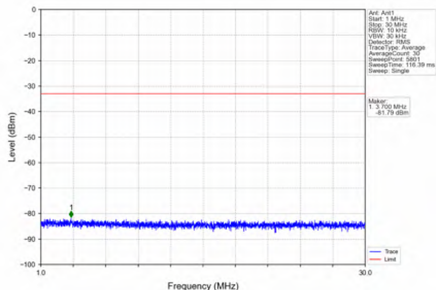
n2 30kHz SISO NTNV 15MHz CP-OFDM QPSK 1902.5MHz Outer Full
