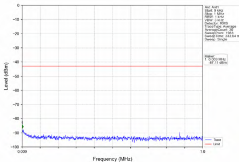
n2_30kHz_SISO_NTNV_20MHz_DFT-s-OFDM_QPSK_1860MHz_Outer_Full
