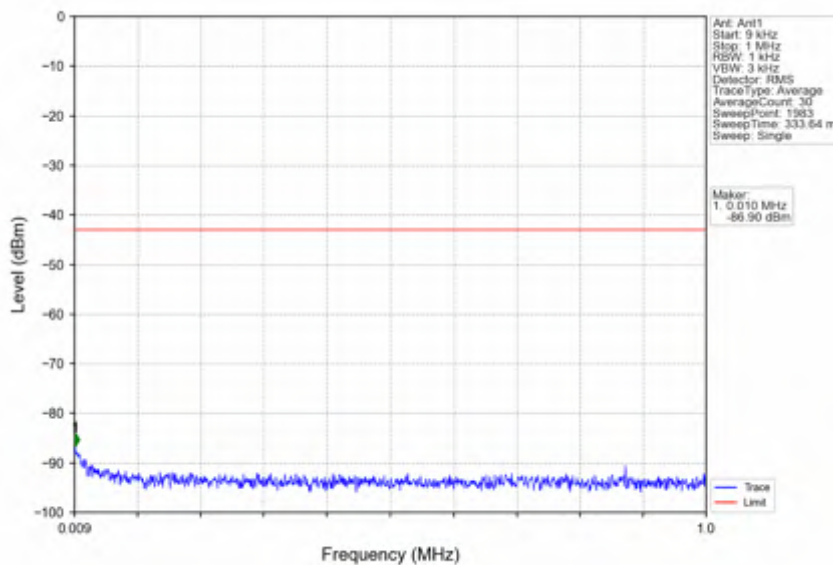
n2_30kHz_SISO_NTNV_20MHz_DFT-s-OFDM_QPSK_1900MHz_Outer_Full
