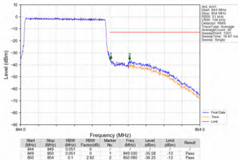
n5_15kHz_SISO_NTNV_5MHz_CP-OFDM QPSK_846.5MHz_Outer_Full
