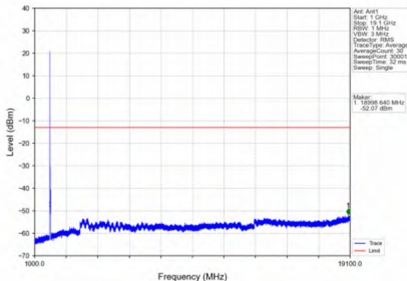
n2_30kHz_SISO_NTNV_20MHz_DFT-s-OFDM QPSK_1900MHz_Edge_1RB_Right
