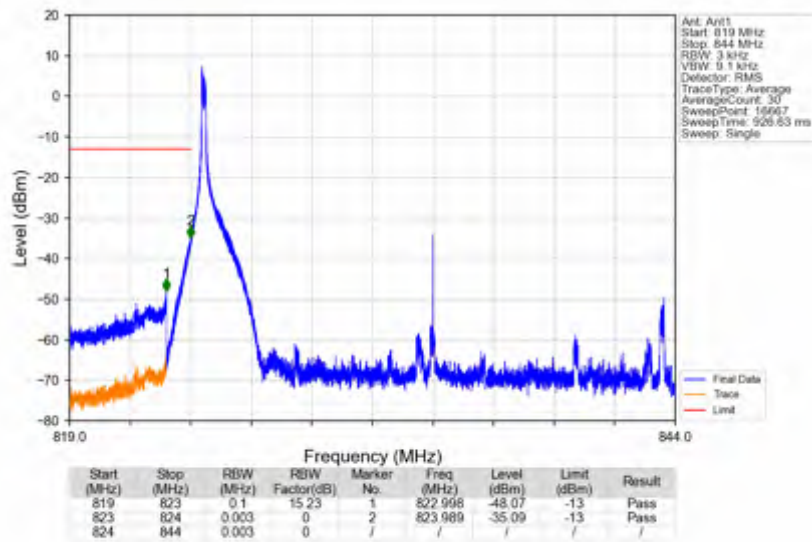
n5_15kHz_SISO_NTNV_20MHz_DFT-s-OFDM_PI/2_BPSK_834MHz_Edge_1RB_Left
