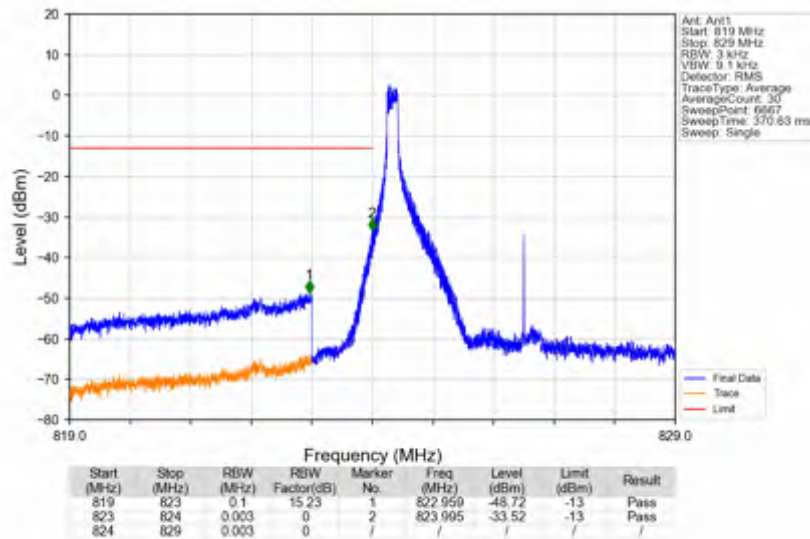
n5_15kHz_SISO_NTNV_5MHz_CP-OFDM_QPSK_826.5MHz_Edge_1RB_Left
