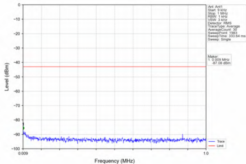
n2_30kHz_SISO_NTNV_20MHz_DFT-s-OFDM PI/2 BPSK_1860MHz_Outer_Full
