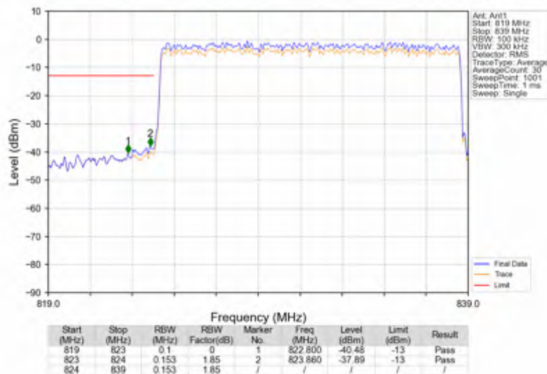
n5_15kHz_SISO_NTNV_15MHz_CP-OFDM QPSK_831.5MHz_Outer_Full
