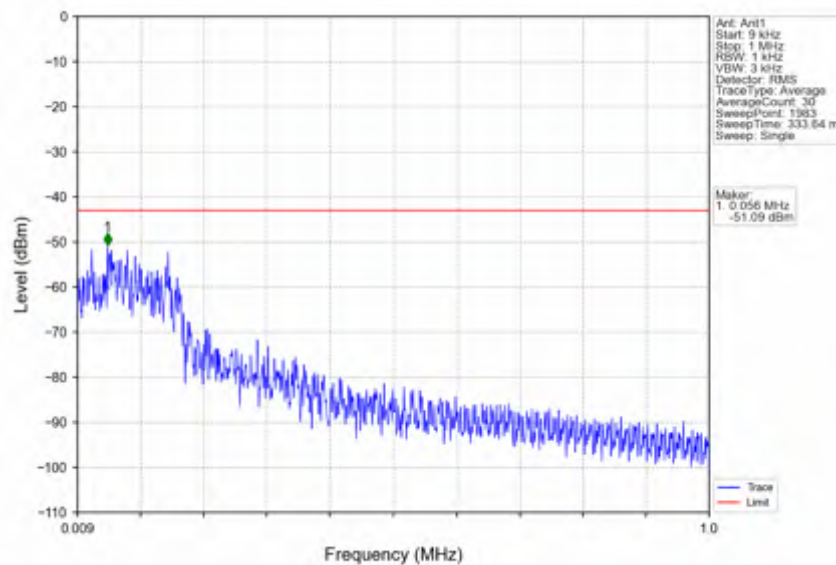
n5_15kHz_SISO_NTNV_10MHz_DFT-s-OFDM QPSK_836.5MHz_Edge_1RB_Left
