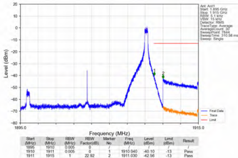
n2_30kHz_SISO_NTNV_15MHz_CP-OFDM_QPSK_1902.5MHz_Edge_1RB_Right
