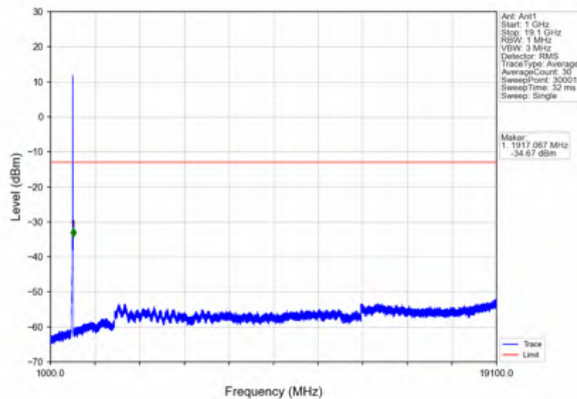
n2_30kHz_SISO_NTNV_20MHz_DFT-s-OFDM PI/2 BPSK_1900MHz_Outer_Full
