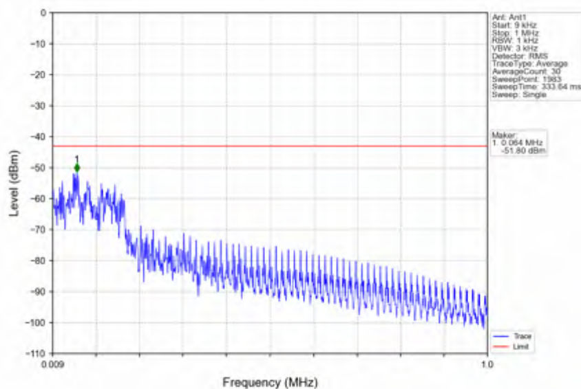
n5_15kHz_SISO_NTNV_15MHz_DFT-s-OFDM PI/2 BPSK 831.5MHz_Edge_1RB_Left
