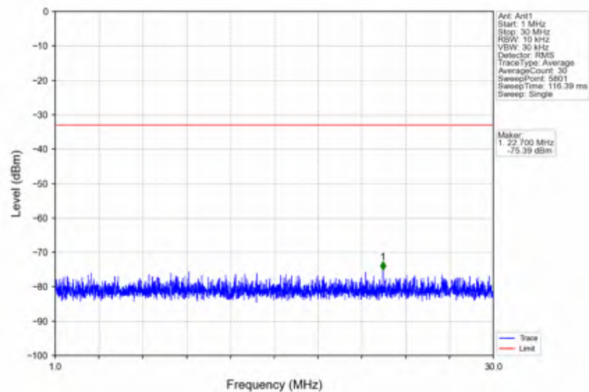
n5_15kHz_SISO_NTNV_10MHz_CP-OFDM_QPSK_829MHz_Edge_1RB_Left
