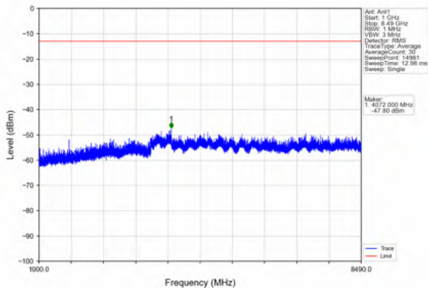
n5_15kHz_SISO_NTNV_15MHz_CP-OFDM_QPSK_841.5MHz_Edge_1RB_Right
