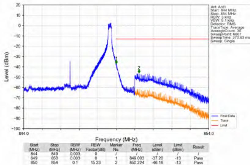
n5_15kHz_SISO_NTNV_5MHz_CP-OFDM QPSK_846.5MHz_Edge_1RB_Right
