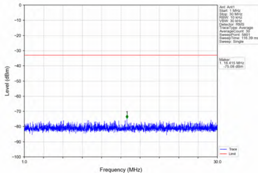
n5_15kHz_SISO_NTNV_15MHz_CP-OFDM_QPSK_836.5MHz_Edge_1RB_Left
