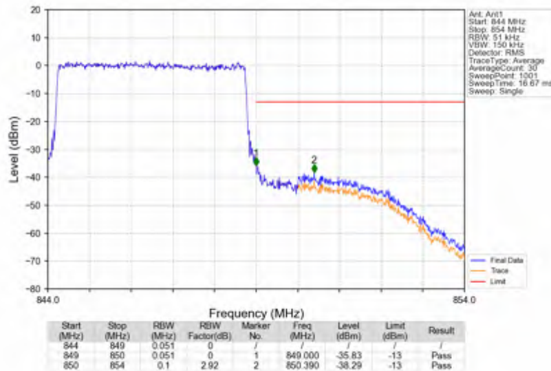
n5_15kHz_SISO_NTNV_5MHz_DFT-s-OFDM QPSK_846.5MHz_Outer_Full
