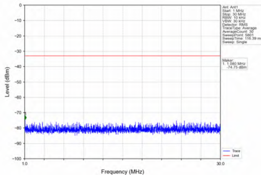
n5_15kHz_SISO_NTNV_15MHz_DFT-s-OFDM_QPSK_836.5MHz_Edge_1RB_Left
