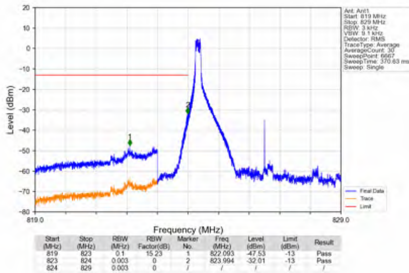
n5_15kHz_SISO_NTNV_5MHz_DFT-s-OFDM_PI/2_BPSK_826.5MHz_Edge_1RB_Left
