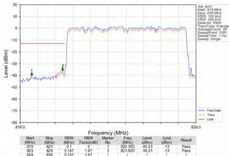
n5_15kHz_SISO_NTNV_15MHz_DFT-s-OFDM QPSK_831.5MHz_Outer_Full
