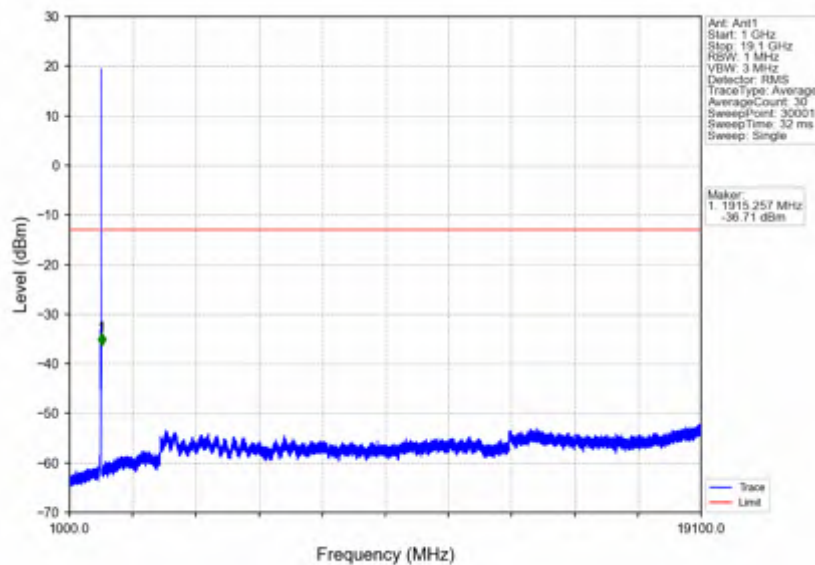
n2_30kHz_SISO_NTNV_15MHz_CP-OFDM QPSK_1902.5MHz_Outer_Full
