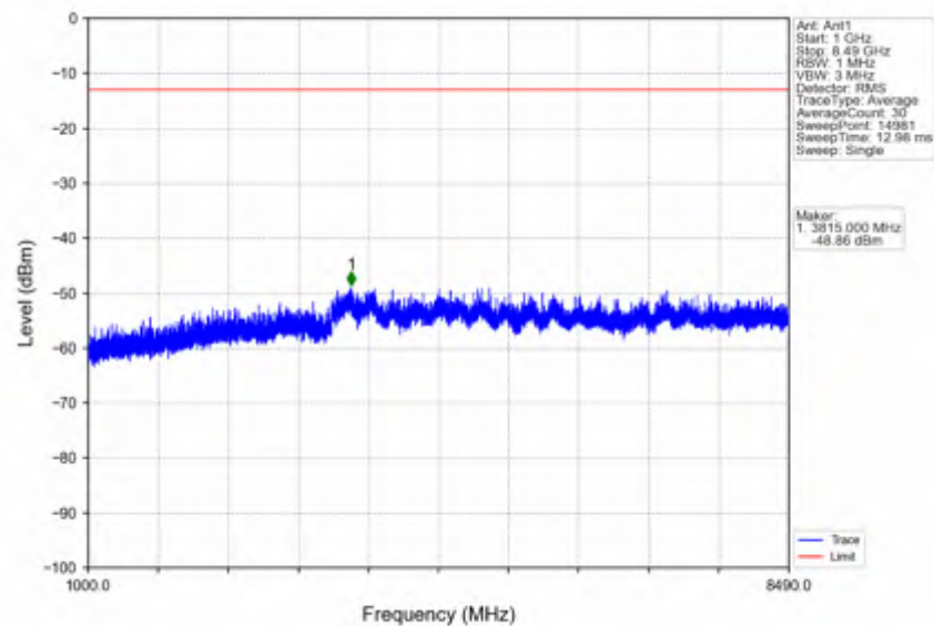
n5_15kHz_SISO_NTNV_15MHz_DFT-s-OFDM QPSK_841.5MHz_Edge_1RB_Right
