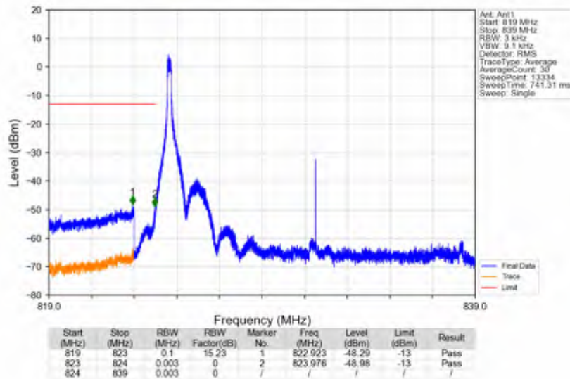
n5_15kHz_SISO_NTV_15MHz_CP-OFDM_QPSK_831.5MHz_Inner_1RB_Left
