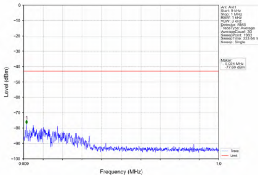
n2_30kHz_SISO_NTNV_15MHz_CP-OFDM_QPSK_1902.5MHz_Inner_1RB_Right
