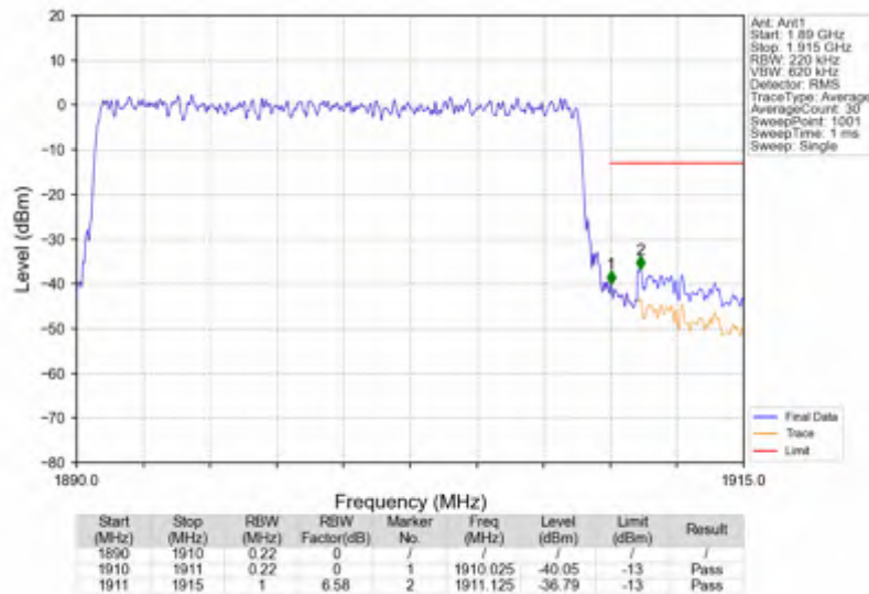
n2_30kHz_SISO_NTNV_20MHz_DFT-s-OFDM_PI/2_BPSK_1900MHz_Outer_Full
