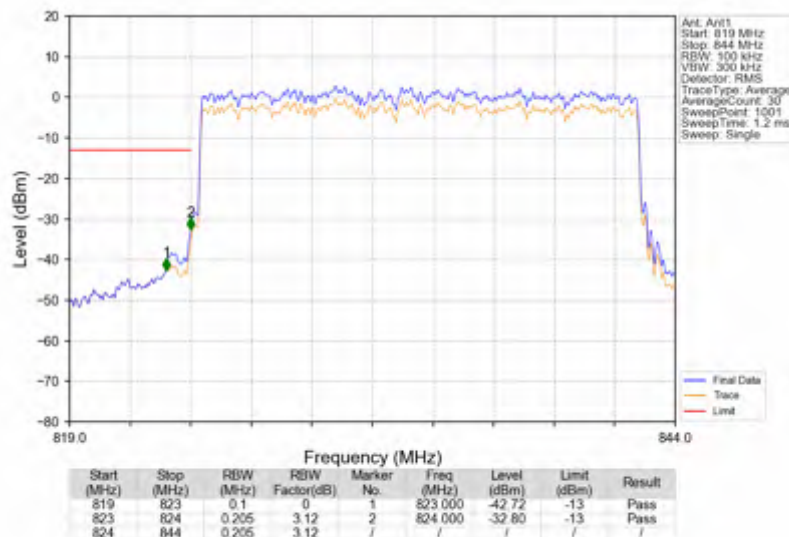
n5_15kHz_SISO_NTNV_20MHz_DFT-s-OFDM PI/2 BPSK_834MHz_Outer_Full
