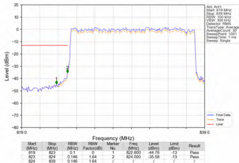
n5_15kHz_SISO_NTNV_15MHz_DFT-s-OFDM PI/2 BPSK_831.5MHz_Outer_Full
