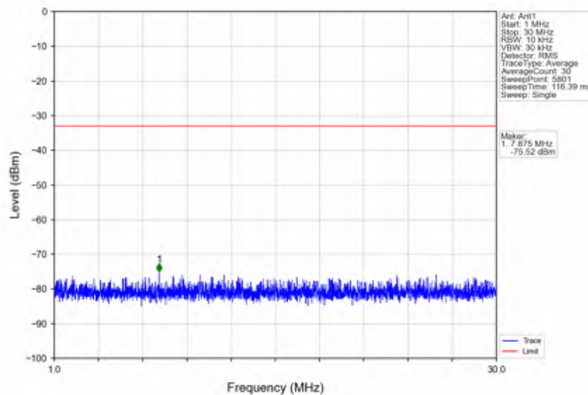
n5_15kHz_SISO_NTNV_20MHz_DFT-s-OFDM QPSK_834MHz_Edge_1RB_Left
