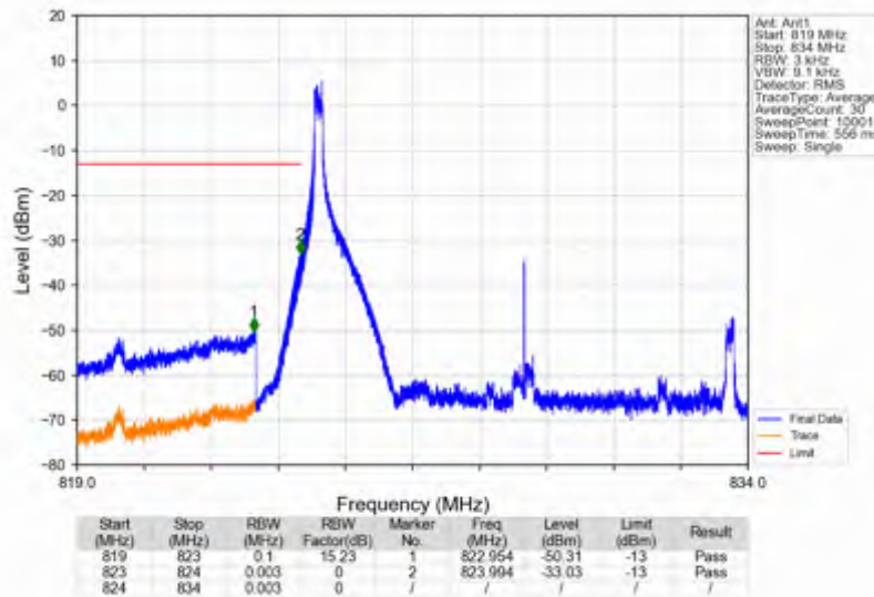
n5_15kHz_SISO_NTNV_10MHz_DFT-s-OFDM_QPSK_829MHz_Edge_1RB_Left
