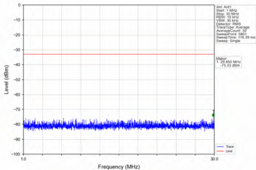
n5_15kHz_SISO_NTNV_20MHz_DFT-s-OFDM QPSK_839MHz_Edge_1RB_Right
