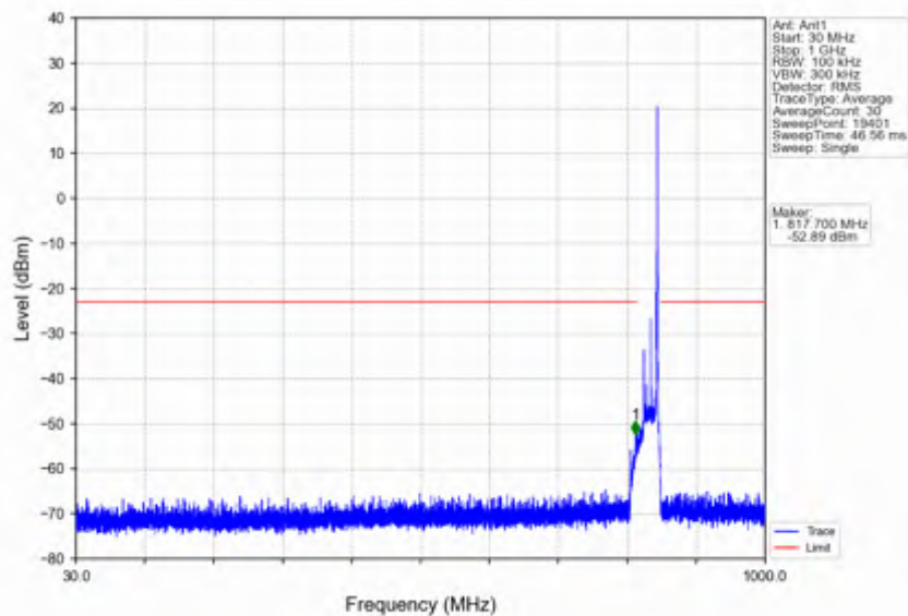
n5_15kHz_SISO_NTNV_20MHz_DFT-s-OFDM_QPSK_839MHz_Edge_1RB_Right
