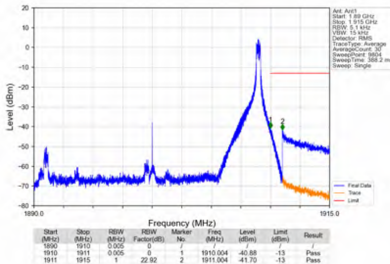
n2_30kHz_SISO_NTNV_20MHz_DFT-s-OFDM QPSK_1900MHz_Edge_1RB_Right
