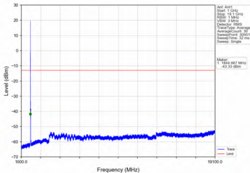
n2_30kHz_SISO_NTNV_15MHz_CP-OFDM QPSK_1880MHz_Edge_1RB_Left
