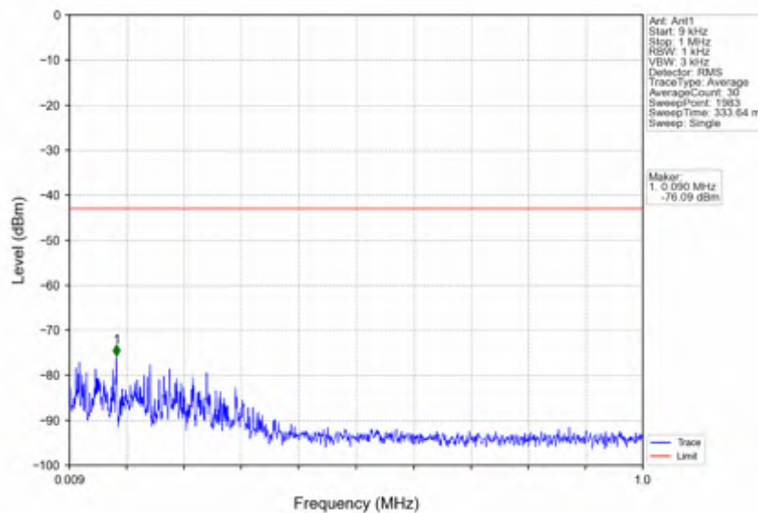
n2_30kHz_SISO_NTNV_15MHz_CP-OFDM_QPSK_1857.5MHz_Inner_1RB_Left
