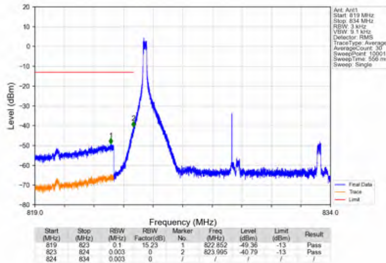
n5_15kHz_SISO_NTNV_10MHz_CP-OFDM QPSK_829MHz_Inner_1RB_Left
