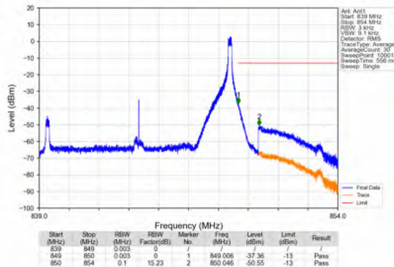
n5_15kHz_SISO_NTNV_10MHz_CP-OFDM QPSK_844MHz_Edge_1RB_Right
