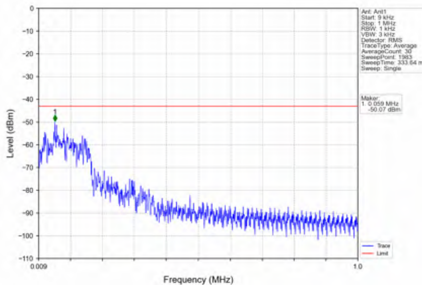
n5_15kHz_SISO_NTNV_20MHz_DFT-s-OFDM_QPSK_834MHz_Edge_1RB_Left
