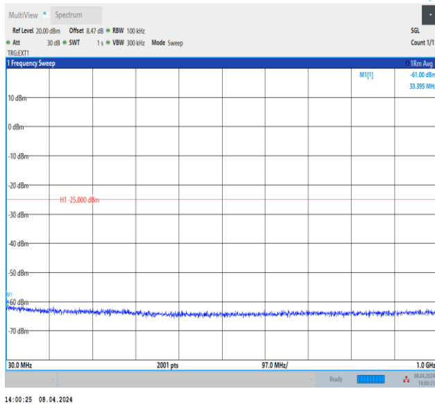
Band38_15MHz_QPSK_38000_1RB#0_30~1000_30~1000
