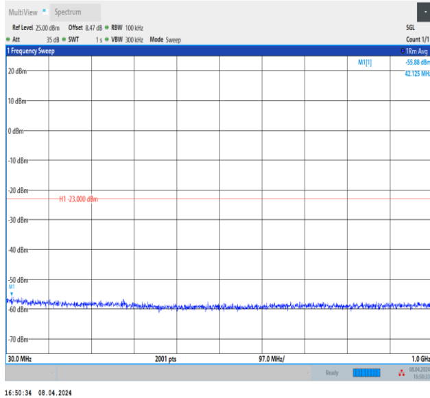
Band66_1.4MHz_QPSK_132665_1RB#0_30~1000_30~100 0
