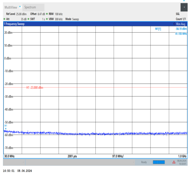
Band66_1.4MHz_QPSK_132322_1RB#0_30~1000_30~100 0
