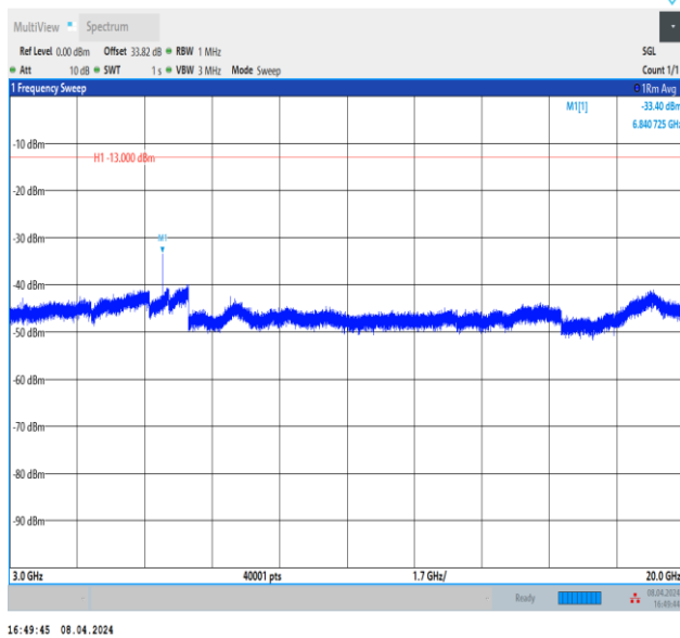
Band66_1.4MHz_QPSK_131979_1RB#0_3000~20000_300 0~20000
