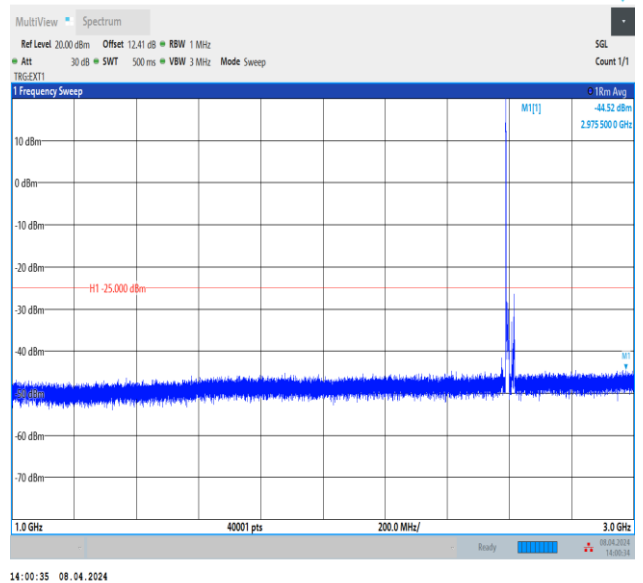
Band38_15MHz_QPSK_38000_1RB#0_1000~3000_1000~3000
