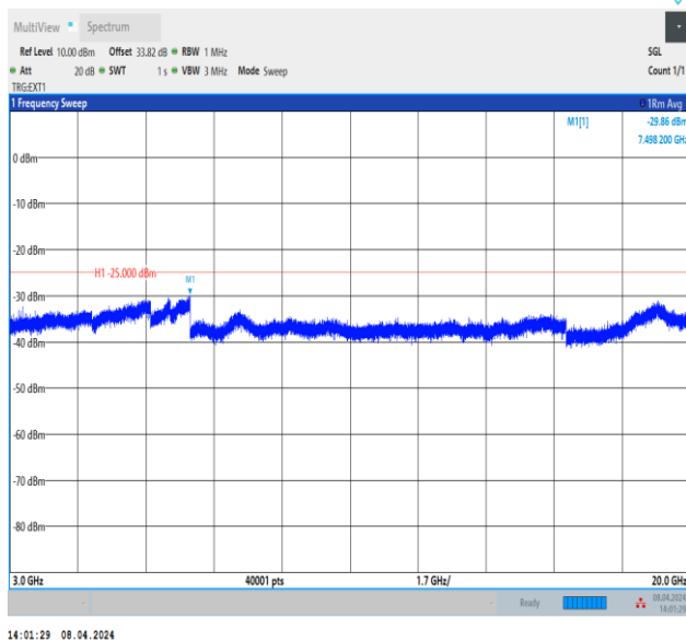
Band38_15MHz_QPSK_38175_1RB#0_3000~20000_3000~20000
