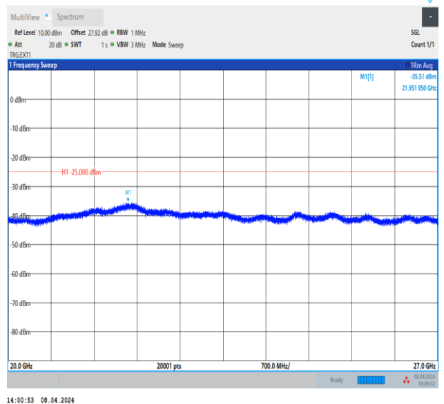
Band38_15MHz_QPSK_38000_1RB#0_20000~27000_20000~27000
