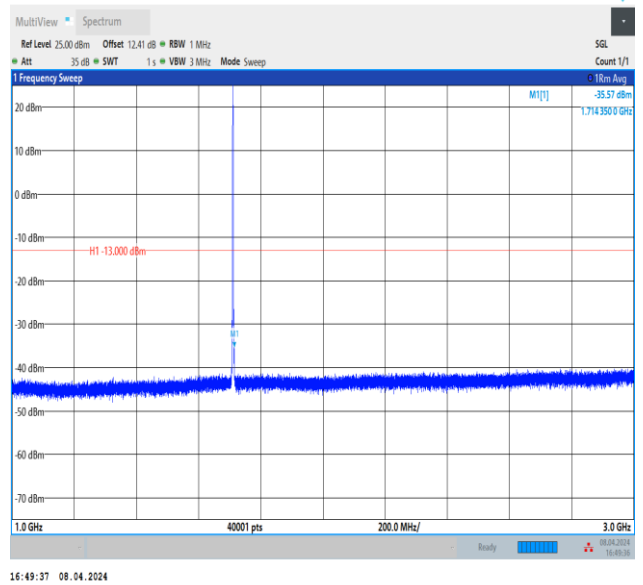
Band66_1.4MHz_QPSK_131979_1RB#0_1000~3000_1000 ~3000
