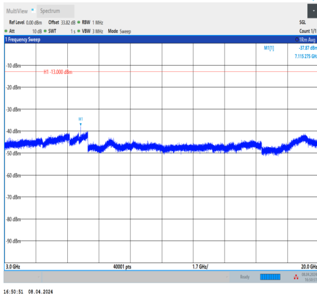
Band66_1.4MHz_QPSK_132665_1RB#0_3000~20000_300 0~20000
