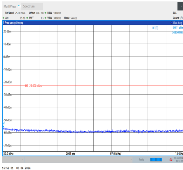
Band66_3MHz_QPSK_132322_1RB#0_30~1000_30~1000
