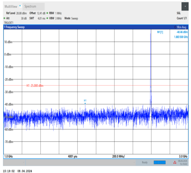
Band41_5MHz_QPSK_40620_1RB#0_1000~3000_1000~3000
