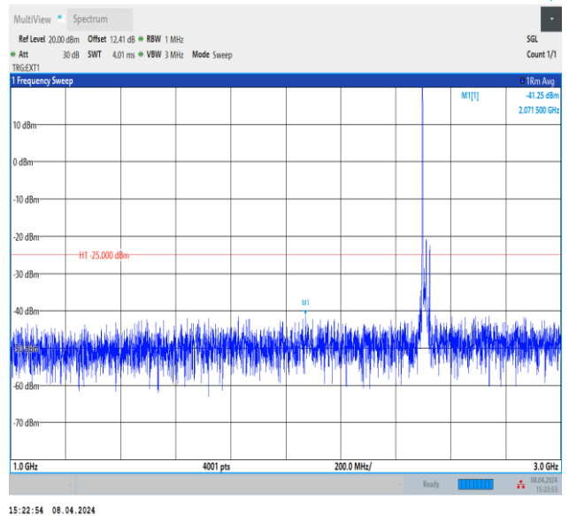
Band41_15MHz_QPSK_39725_1RB#0_1000~3000_1000~3000
