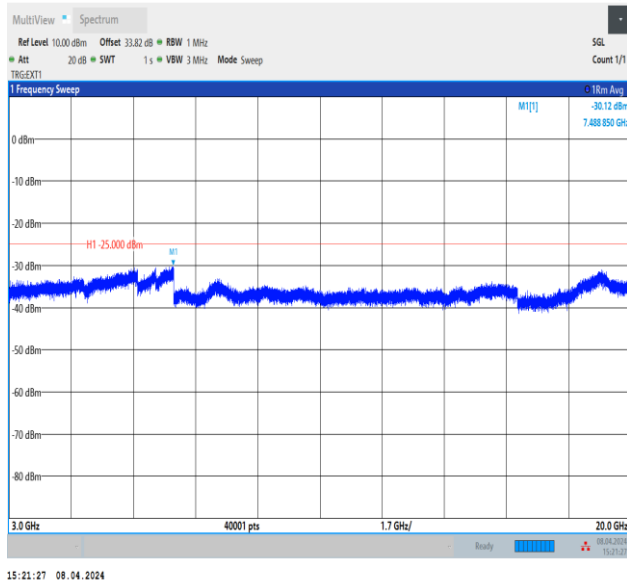
Band41_10MHz_QPSK_40620_1RB#0_3000~20000_3000~20000
