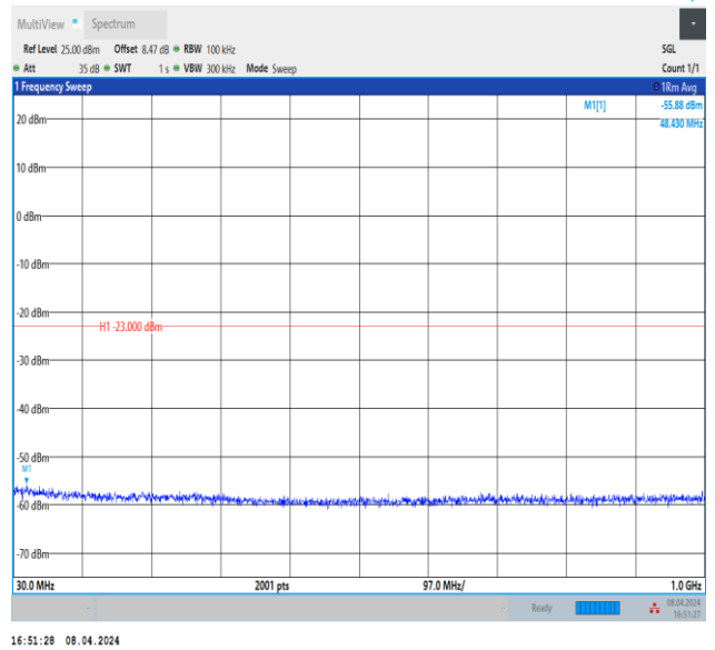
Band66_3MHz_QPSK_131987_1RB#0_30~1000_30~1000
