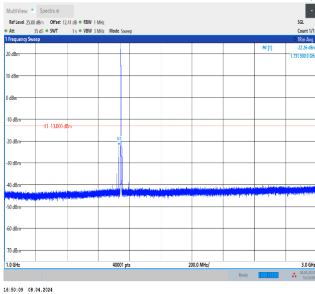
Band66_1.4MHz_QPSK_132322_1RB#0_1000~3000_1000 ~3000
