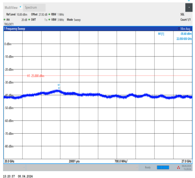
Band41_10MHz_QPSK_39700_1RB#0_20000~27000_20000~27000
