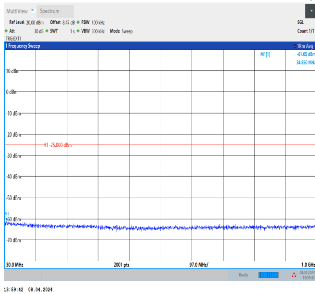
Band38_15MHz_QPSK_37825_1RB#0_30~1000_30~1000
