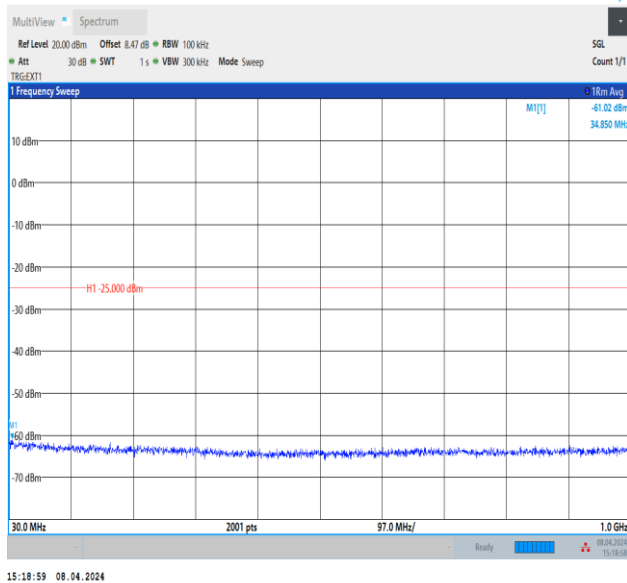
Band41_5MHz_QPSK_40620_1RB#0_30~1000_30~1000
