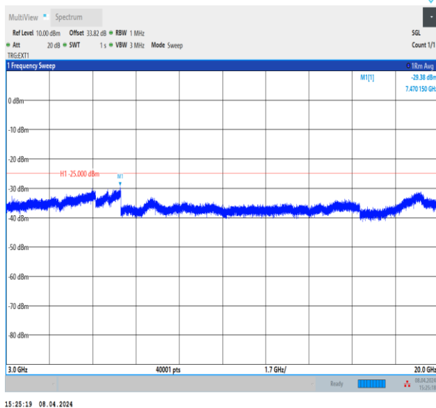
Band41_20MHz_QPSK_39750_1RB#0_3000~20000_3000~20000
