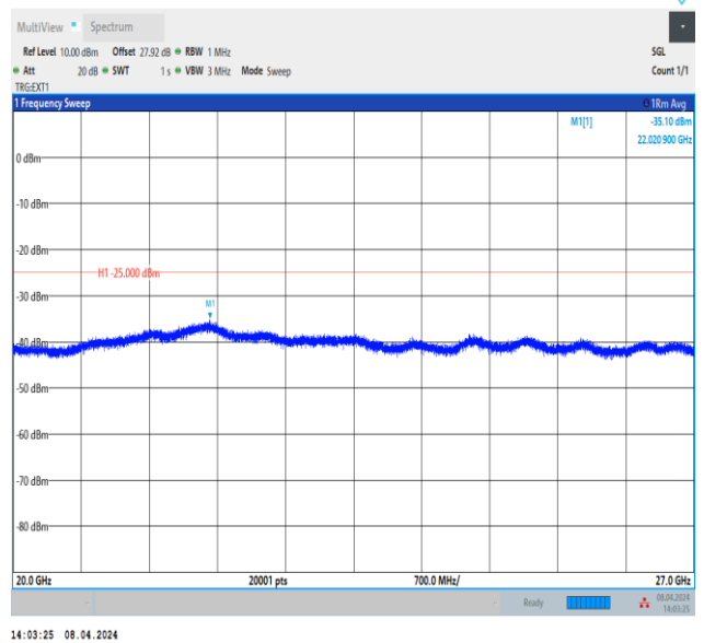
Band38_20MHz_QPSK_38000_1RB#0_20000~27000_20000~27000
