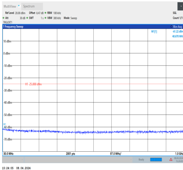
Band41_15MHz_QPSK_41515_1RB#0_30~1000_30~1000
