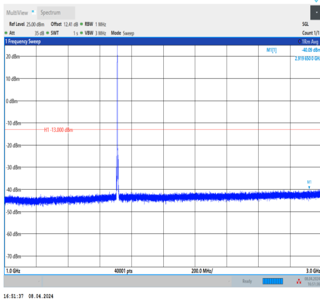
Band66_3MHz_QPSK_131987_1RB#0_1000~3000_1000~3 000
