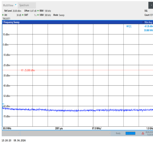
Band41_20MHz_QPSK_41490_1RB#0_30~1000_30~1000
