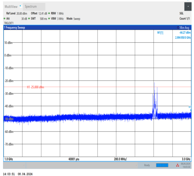
Band38_20MHz_QPSK_38150_1RB#0_1000~3000_1000~3000
