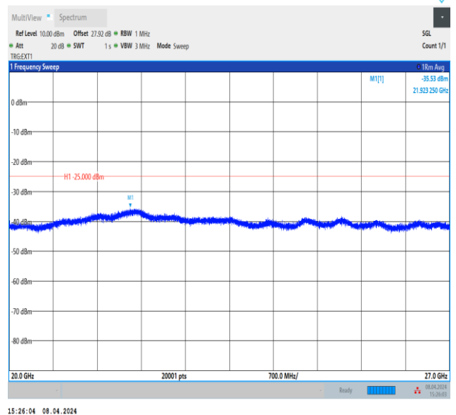
Band41_20MHz_QPSK_40620_1RB#0_20000~27000_20000~27000
