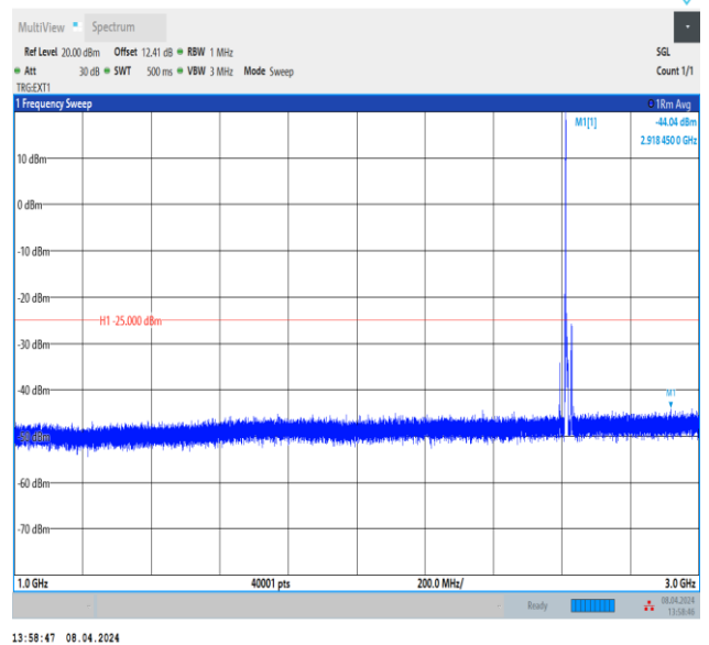
Band38_10MHz_QPSK_38200_1RB#0_1000~3000_1000~3000
