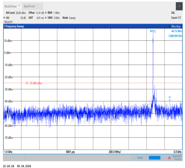
Band41_20MHz_QPSK_41490_1RB#0_1000~3000_1000~3000
