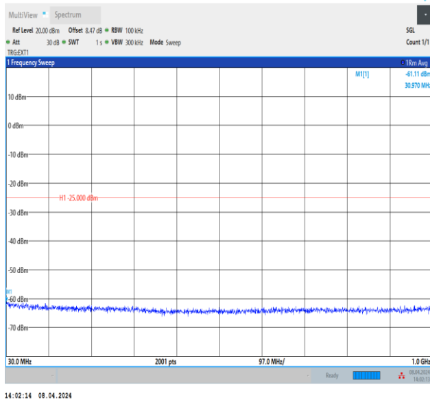
Band38_20MHz_QPSK_37850_1RB#0_30~1000_30~1000
