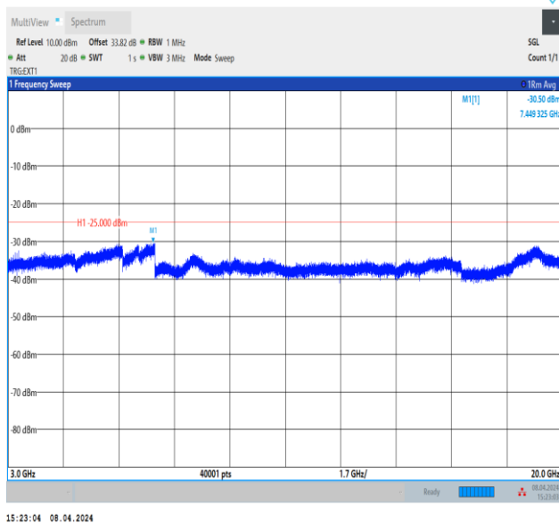
Band41_15MHz_QPSK_39725_1RB#0_3000~20000_3000~20000
