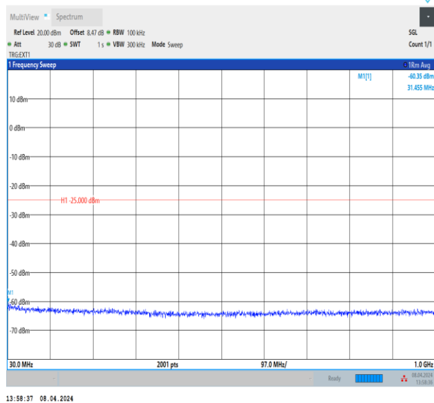
Band38_10MHz_QPSK_38200_1RB#0_30~1000_30~1000
