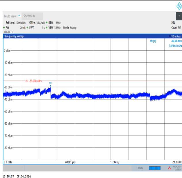
Band38_10MHz_QPSK_38200_1RB#0_3000~20000_3000~ 20000
