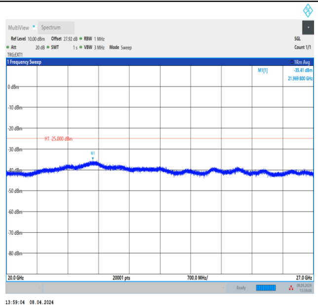
Band38_10MHz_QPSK_38200_1RB#0_20000~27000_2000 0~27000
