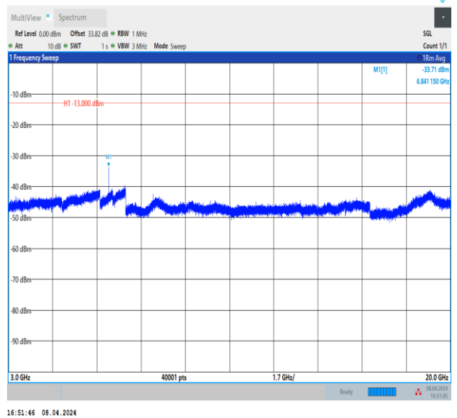
Band66_3MHz_QPSK_131987_1RB#0_3000~20000_3000~ 20000
