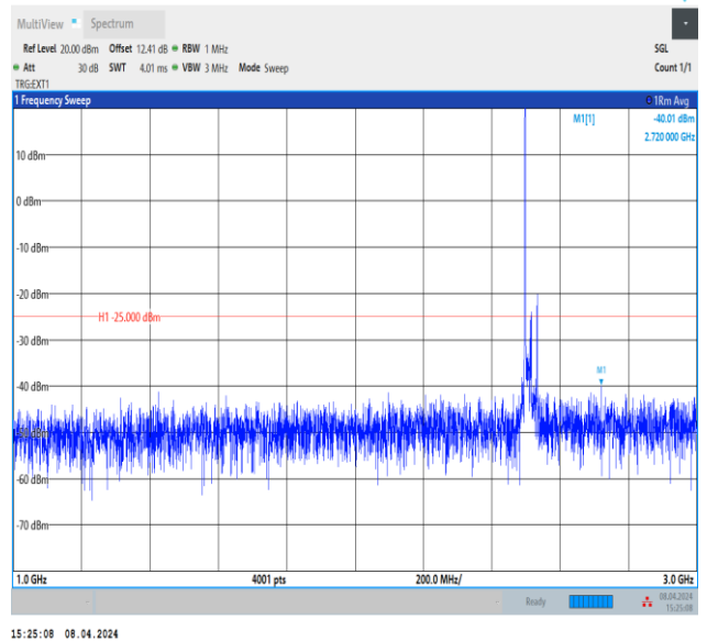
Band41_20MHz_QPSK_39750_1RB#0_1000~3000_1000~3000
