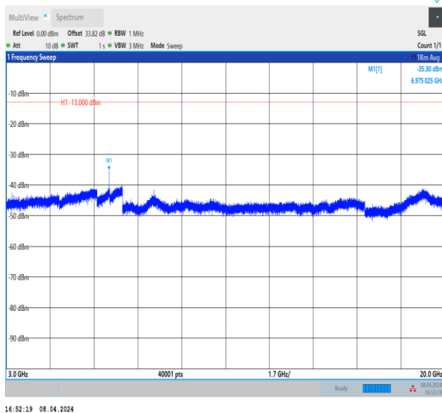
Band66_3MHz_QPSK_132322_1RB#0_3000~20000_3000~20000
