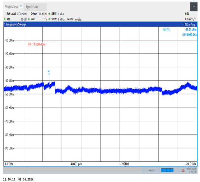
Band66_1.4MHz_QPSK_132322_1RB#0_3000~20000_3000 ~20000
