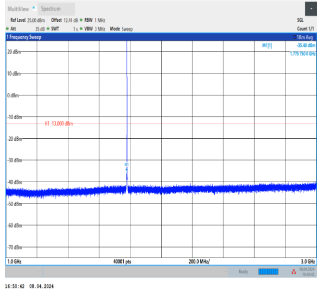
Band66_1.4MHz_QPSK_132665_1RB#0_1000~3000_1000 ~3000
