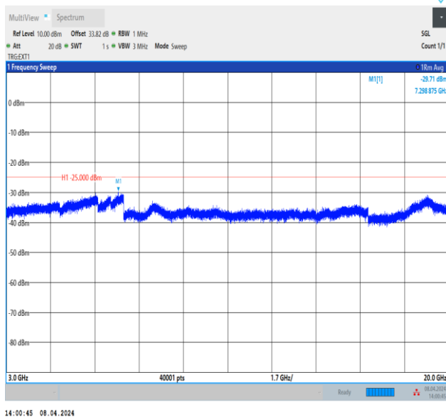
Band38_15MHz_QPSK_38000_1RB#0_3000~20000_3000~20000
