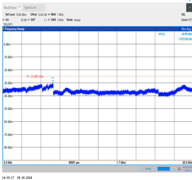
Band38_20MHz_QPSK_38000_1RB#0_3000~20000_3000~20000
