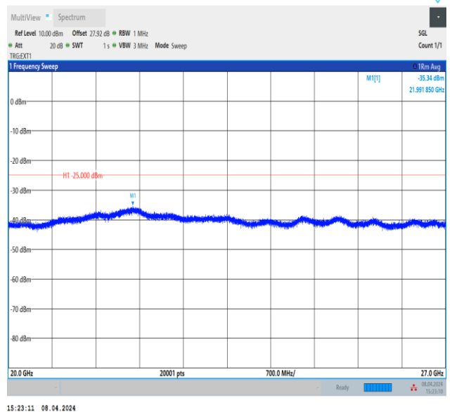
Band41_15MHz_QPSK_39725_1RB#0_20000~27000_20000~27000
