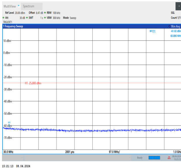
Band41_10MHz_QPSK_40620_1RB#0_30~1000_30~1000
