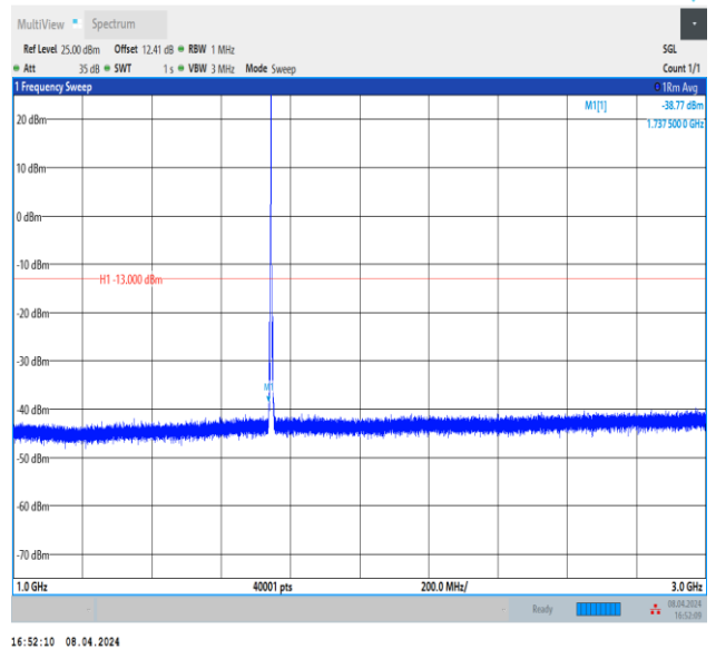
Band66_3MHz_QPSK_132322_1RB#0_1000~3000_1000~3000
