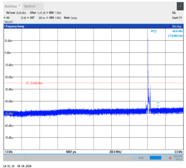
Band38_15MHz_QPSK_38175_1RB#0_1000~3000_1000~3000
