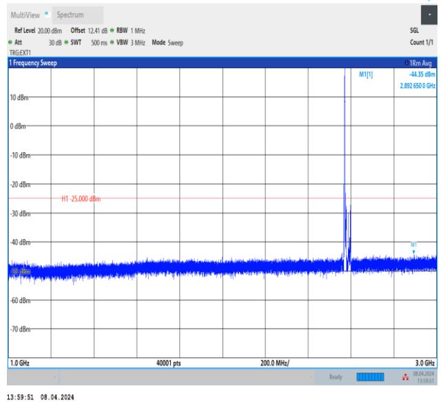
Band38_15MHz_QPSK_37825_1RB#0_1000~3000_1000~3000
