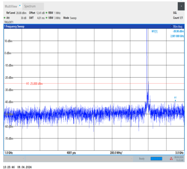
Band41_20MHz_QPSK_40620_1RB#0_1000~3000_1000~3000
