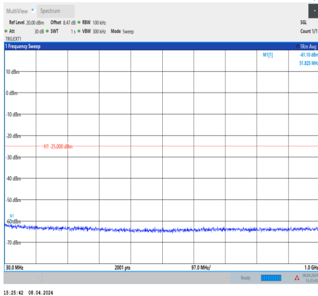
Band41_20MHz_QPSK_40620_1RB#0_30~1000_30~1000
