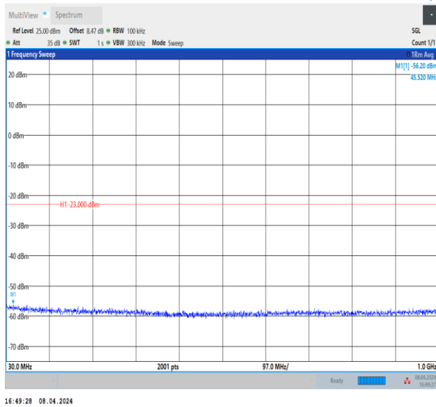
Band66_1.4MHz_QPSK_131979_1RB#0_30~1000_30~100 0
