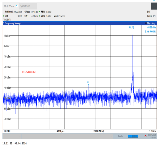
Band41_10MHz_QPSK_41540_1RB#0_1000~3000_1000~3000
