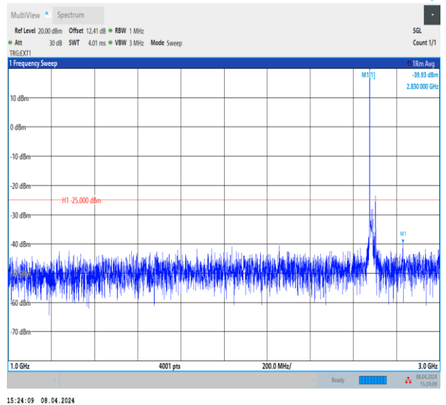
Band41_15MHz_QPSK_41515_1RB#0_1000~3000_1000~3000
