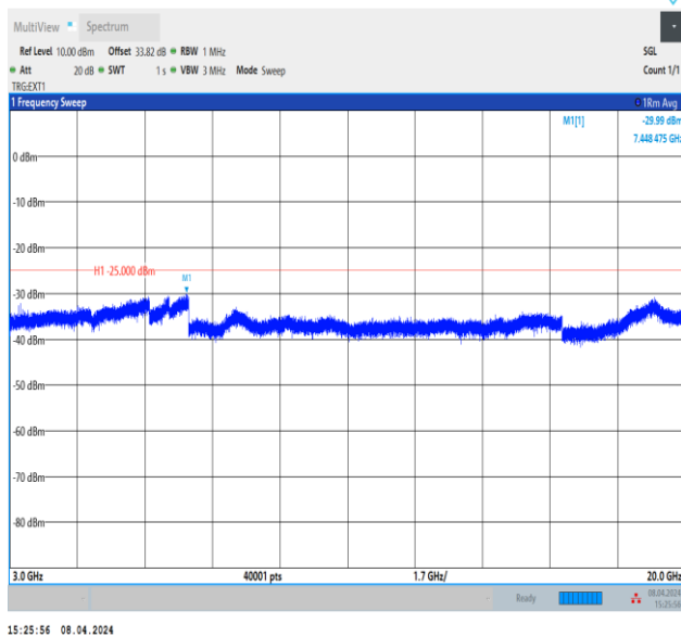
Band41_20MHz_QPSK_40620_1RB#0_3000~20000_3000~20000
