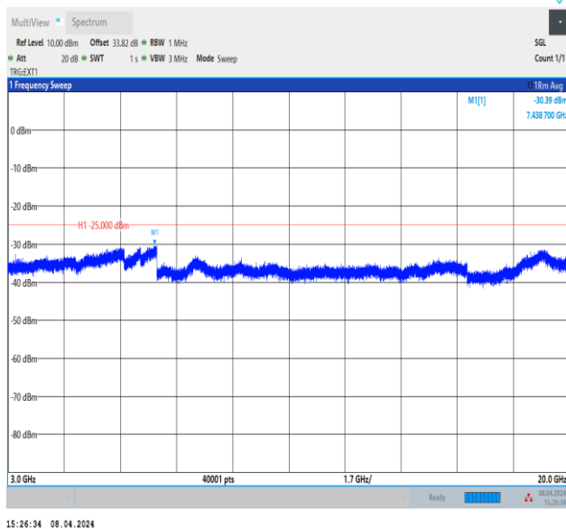
Band41_20MHz_QPSK_41490_1RB#0_3000~20000_3000~20000
