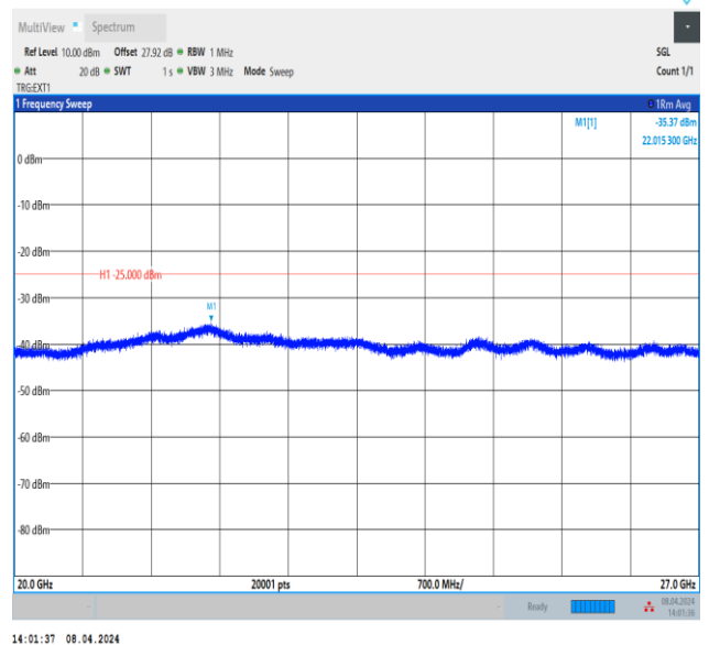
Band38_15MHz_QPSK_38175_1RB#0_20000~27000_20000~27000
