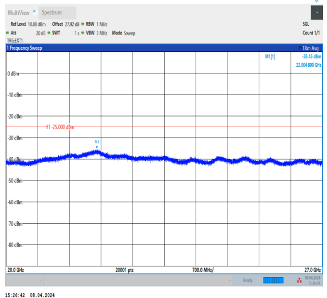
Band41_20MHz_QPSK_41490_1RB#0_20000~27000_20000~27000
