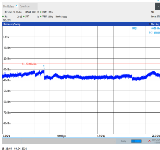
Band41_10MHz_QPSK_41540_1RB#0_3000~20000_3000~20000
