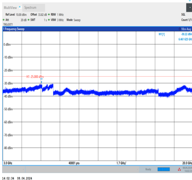
Band38_20MHz_QPSK_37850_1RB#0_3000~20000_3000~20000
