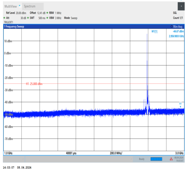
Band38_20MHz_QPSK_38000_1RB#0_1000~3000_1000~3000
