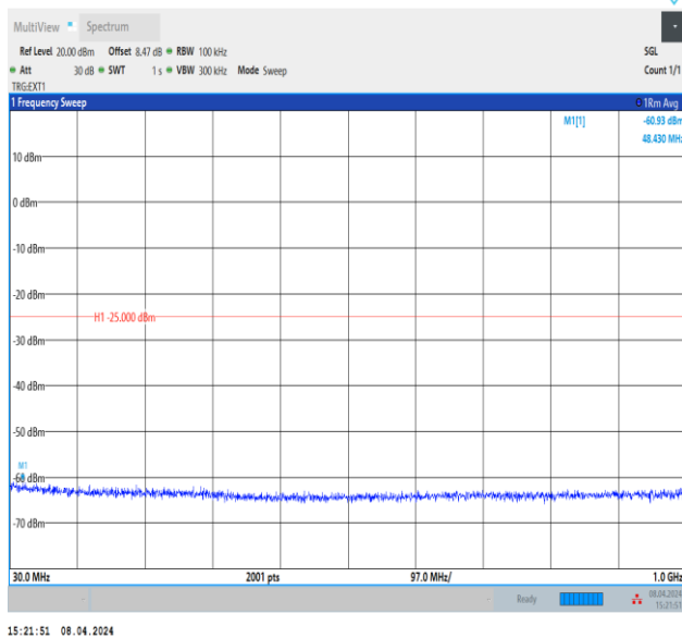
Band41_10MHz_QPSK_41540_1RB#0_30~1000_30~1000
