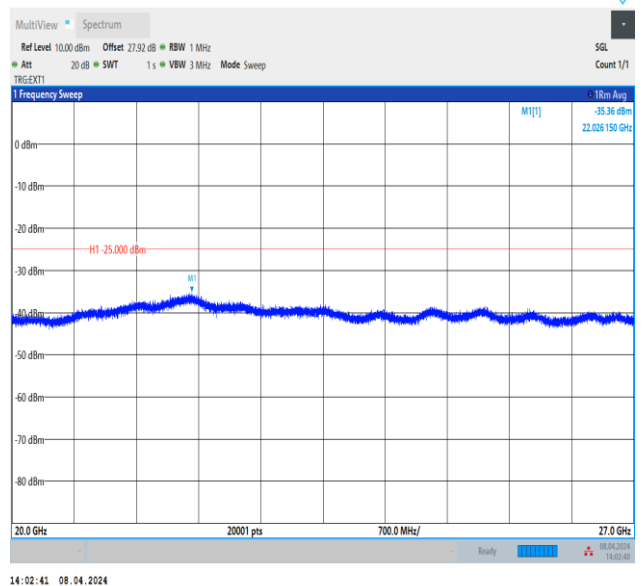
Band38_20MHz_QPSK_37850_1RB#0_20000~27000_2000~27000
