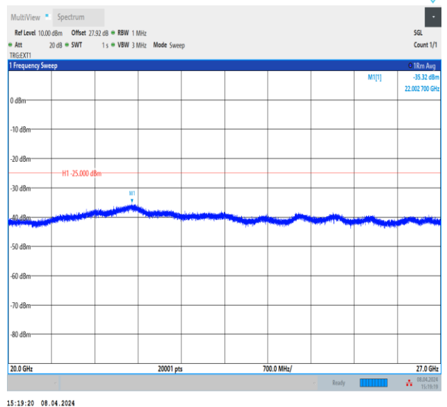
Band41_5MHz_QPSK_40620_1RB#0_20000~27000_20000~27000
