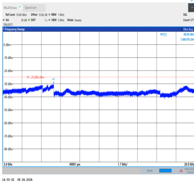
Band38_15MHz_QPSK_37825_1RB#0_3000~20000_3000~20000
