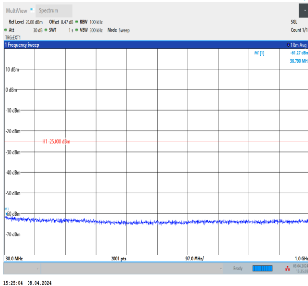
Band41_20MHz_QPSK_39750_1RB#0_30~1000_30~1000
