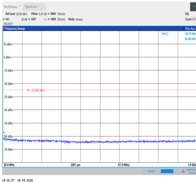
Band38_20MHz_QPSK_38000_1RB#0_30~1000_30~1000
