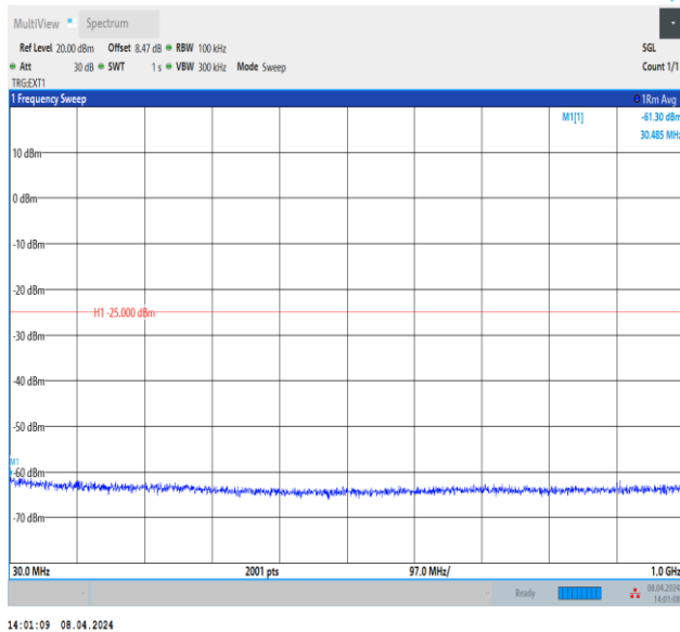
Band38_15MHz_QPSK_38175_1RB#0_30~1000_30~1000
