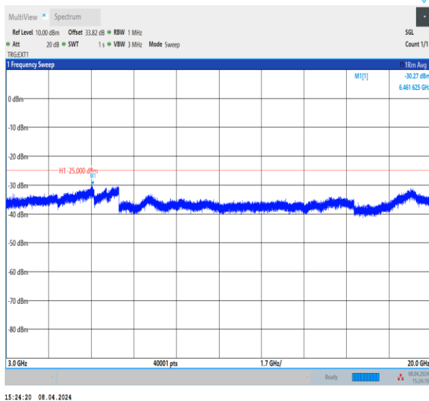
Band41_15MHz_QPSK_41515_1RB#0_3000~20000_3000~20000
