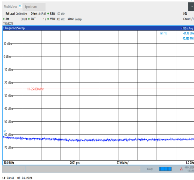
Band38_20MHz_QPSK_38150_1RB#0_30~1000_30~1000
