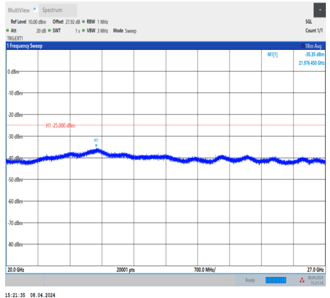
Band41_10MHz_QPSK_40620_1RB#0_20000~27000_20000~27000
