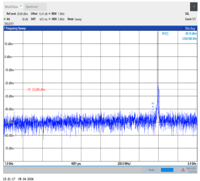
Band41_10MHz_QPSK_40620_1RB#0_1000~3000_1000~3000
