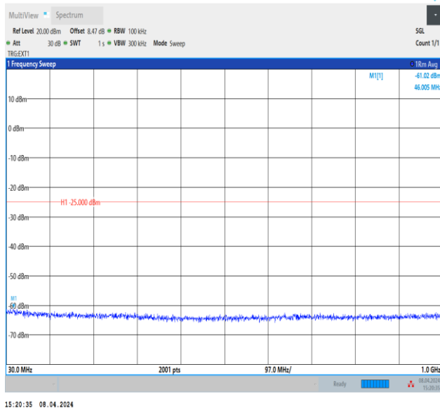
Band41_10MHz_QPSK_39700_1RB#0_30~1000_30~1000
