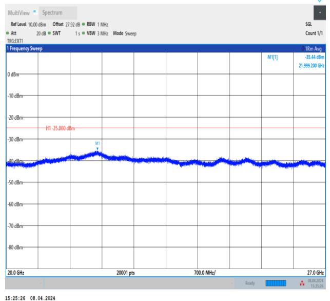
Band41_20MHz_QPSK_39750_1RB#0_20000~27000_20000~27000
