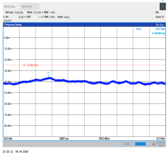
Band41_10MHz_QPSK_41540_1RB#0_20000~27000_20000~27000
