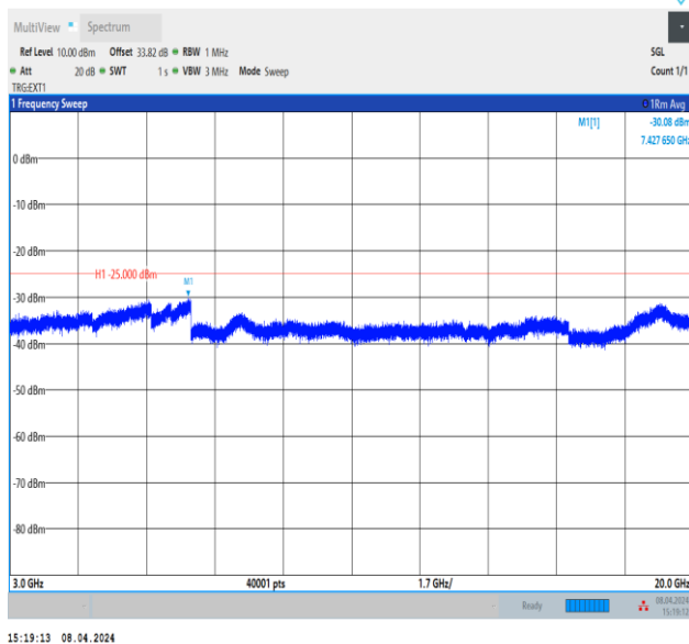
Band41_5MHz_QPSK_40620_1RB#0_3000~20000_3000~20000
