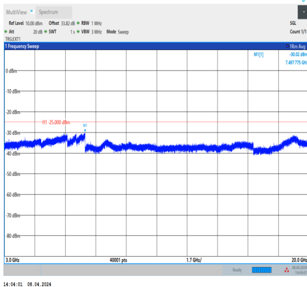
Band38_20MHz_QPSK_38150_1RB#0_3000~20000_3000~20000
