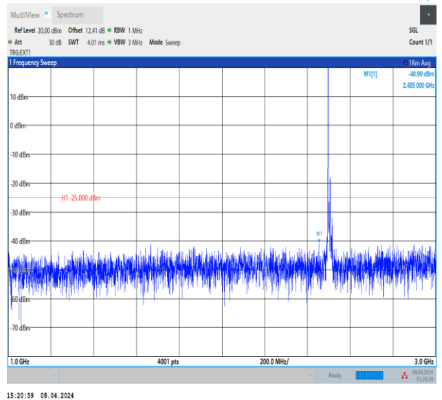
Band41_10MHz_QPSK_39700_1RB#0_1000~3000_1000~3000
