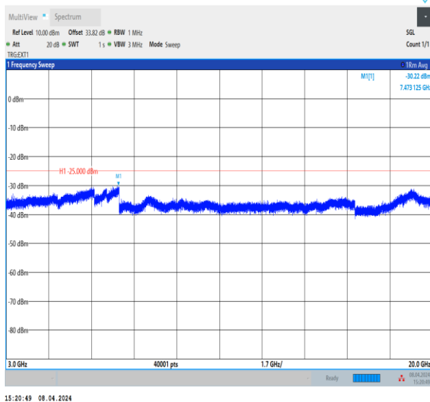
Band41_10MHz_QPSK_39700_1RB#0_3000~20000_3000~20000
