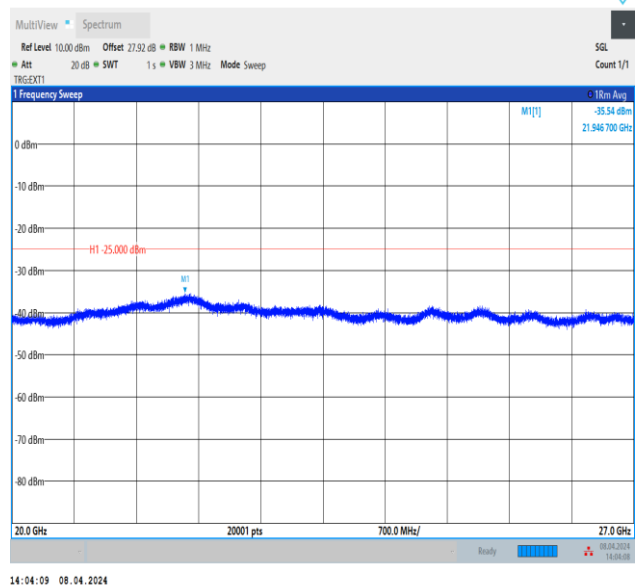
Band38_20MHz_QPSK_38150_1RB#0_20000~27000_20000~27000
