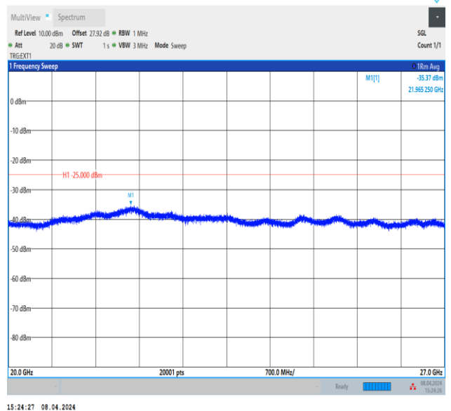
Band41_15MHz_QPSK_41515_1RB#0_20000~27000_20000~27000
