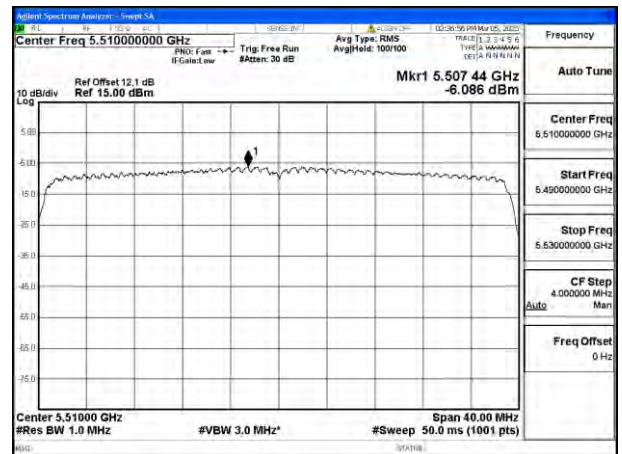
Mode:802.11ax HE40 Tone:484T Frequency:5510MHz Ant:Chain1
