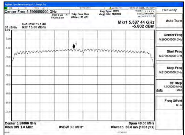
Mode:802.11ax HE40 Tone:484T Frequency:5590MHz Ant:Chain0
