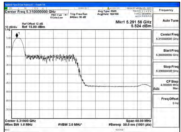
Mode:802.11ax HE40 Tone:26T Frequency:5310MHz Ant:Chain0
