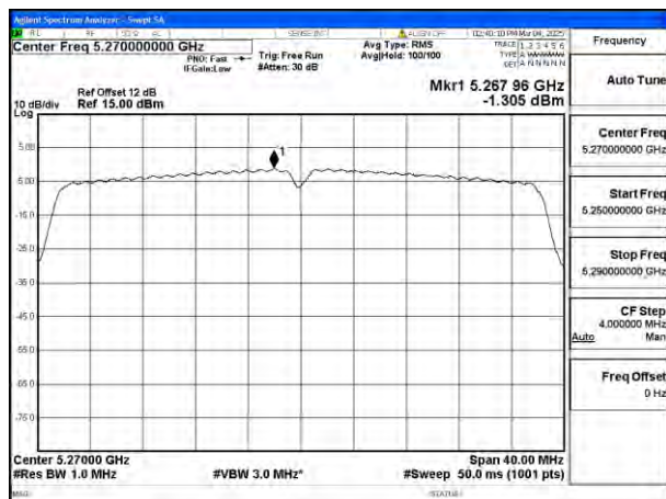
Mode:802.11ac VHT40 Frequency:5270MHz Ant:Chain0
