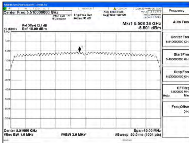
Mode:802.11ax HE40 Tone:484T Frequency:5510MHz Ant:Chain0
