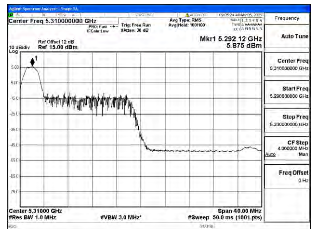
Mode:802.11ax HE40 Tone:26T Frequency:5310MHz Ant:Chain1
