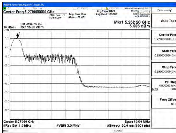
Mode:802.11ax HE40 Tone:26T Frequency:5270MHz Ant:Chain0
