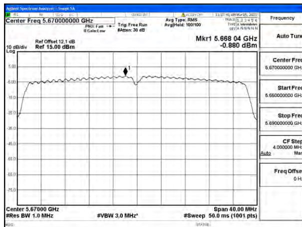
Mode:802.11n HT40 Frequency:5670MHz Ant:Chain0
