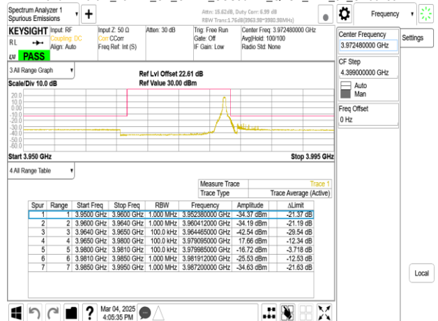
Band77-Part27_15MHz_CP_OFDM_SCS30kHz_QPSK_RB38_0_CH664832
