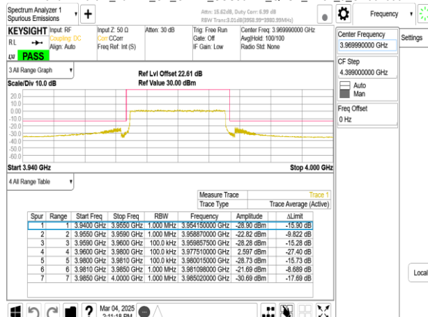
Band77-Part27_20MHz_CP_OFDM_SCS30kHz_QPSK_RB51_0_CH664666
