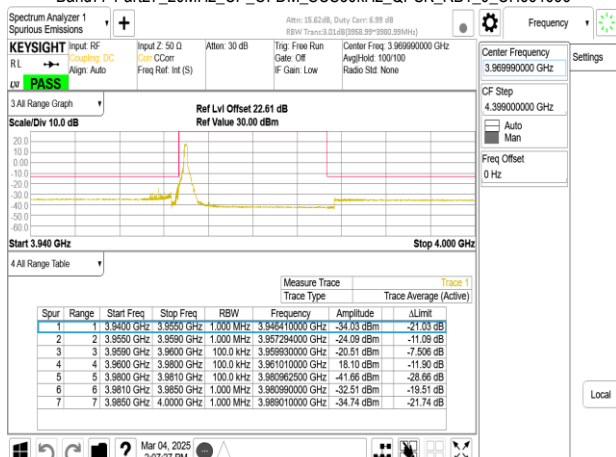
Band77-Part27_20MHz_CP_OFDM_SCS30kHz_QPSK_RB1_0_CH664666
