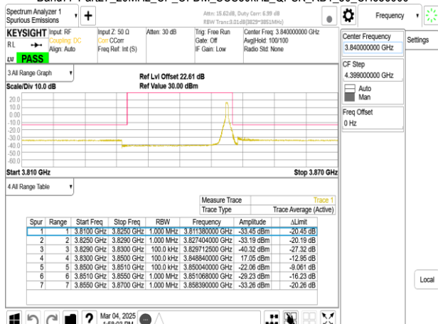
Band77-Part27_20MHz_CP_OFDM_SCS30kHz_QPSK_RB51_0_CH6566000
