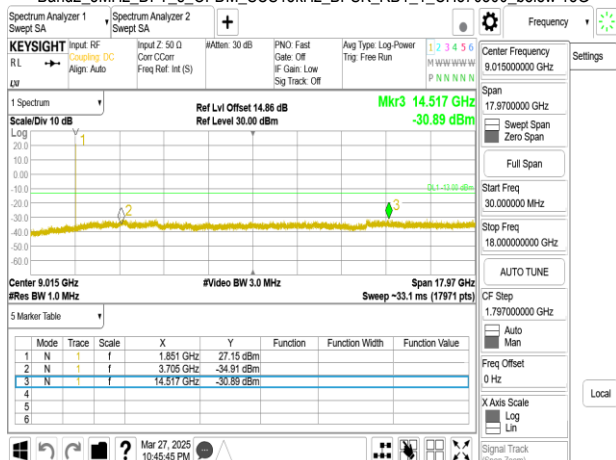
Band2_5MHz_DFT_s_OFDM_SCS15kHz_BPSK_RB1_1_CH370500upper 18G
