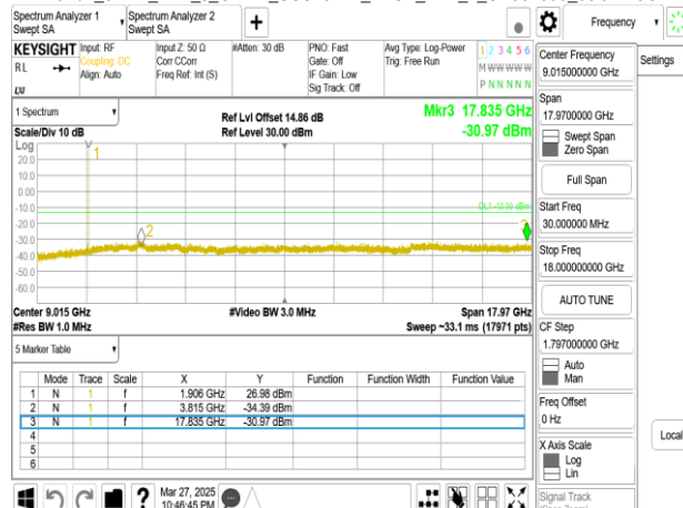
Band2_5MHz_DFT_s_OFDM_SCS15kHz_BPSK_RB1_1_CH381500upper 18G
