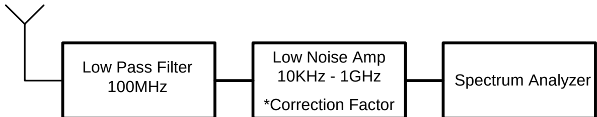
Figure 2 Radiated Emission test 10 KHz – 30MHz
