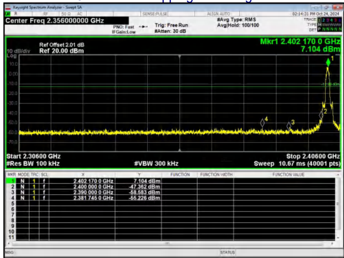
8-DPSK No-hopping Band edge-left side
