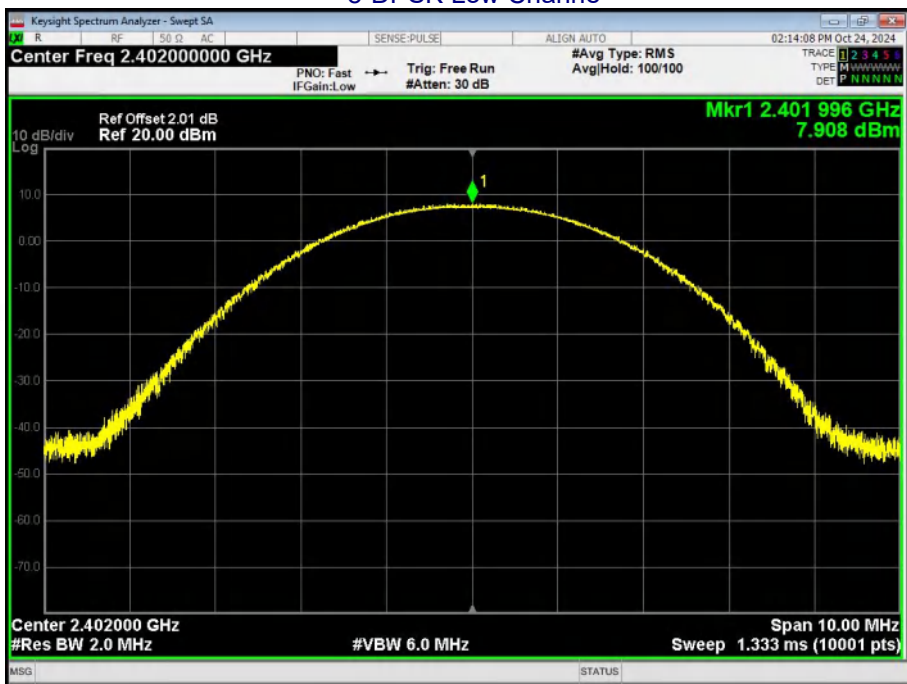
8-DPSK Low Channe
