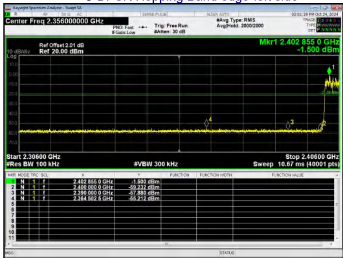
8-DPSK Hopping Band edge-left side
