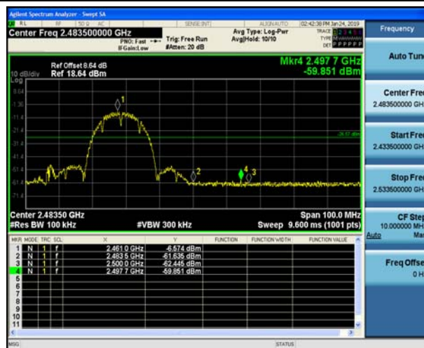
Spurious emission
