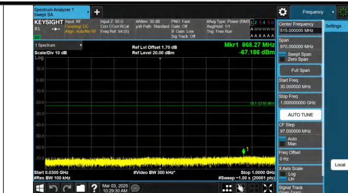
Band2-3MHz-QPSK-19185-1RB#14-30~1000-PASS
