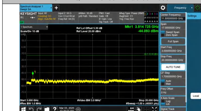
Band2-3MHz-QPSK-19185-1RB#0-3000~20000-PASS
