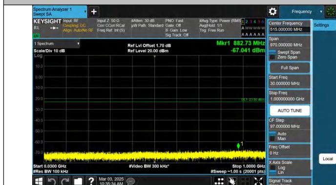
Band2-5MHz-QPSK-18625-1RB#0-30~1000-PASS
