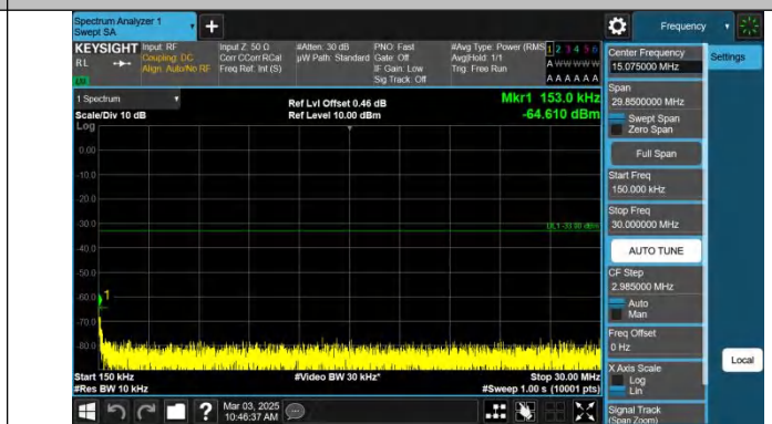
Band2-10MHz-QPSK-18900-1RB#0-0.15~30-PASS
