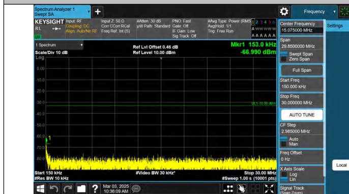
Band2-5MHz-QPSK-18625-1RB#24-0.15~30-PASS
