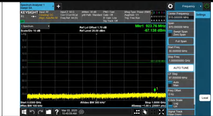
Band2-10MHz-QPSK-18650-1RB#49-30~1000-PASS
