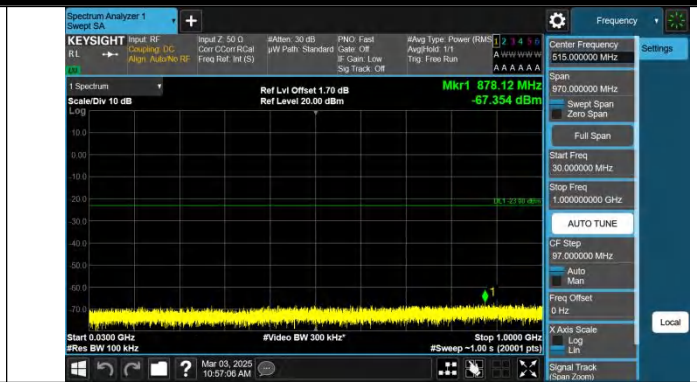
Band2-15MHz-QPSK-18900-1RB#74-30~1000-PASS
