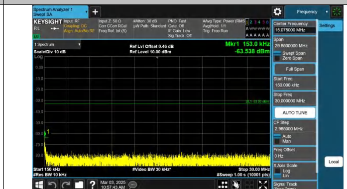
Band2-15MHz-QPSK-19125-1RB#0-0.15~30-PASS
