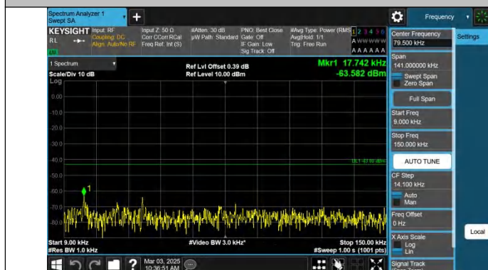
Band2-5MHz-QPSK-18900-1RB#0-0.009~0.15-PASS
