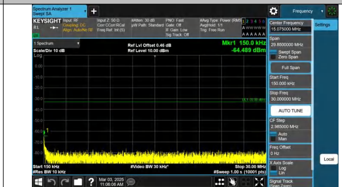
Band2-20MHz-QPSK-19100-1RB#0-0.15~30-PASS
