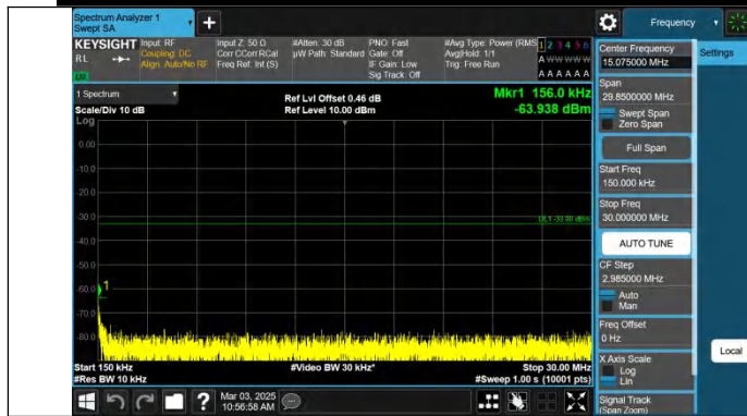
Band2-15MHz-QPSK-18900-1RB#74-0.15~30-PASS
