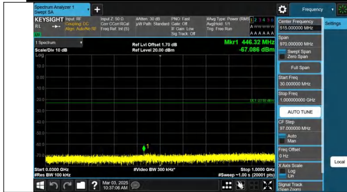
Band2-5MHz-QPSK-18900-1RB#0-30~1000-PASS
