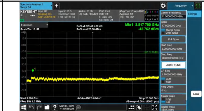
Band2-20MHz-QPSK-19100-1RB#99-3000~20000-PASS
