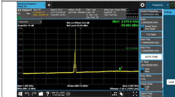
Band2-20MHz-QPSK-19100-1RB#99-1000~3000-PASS
