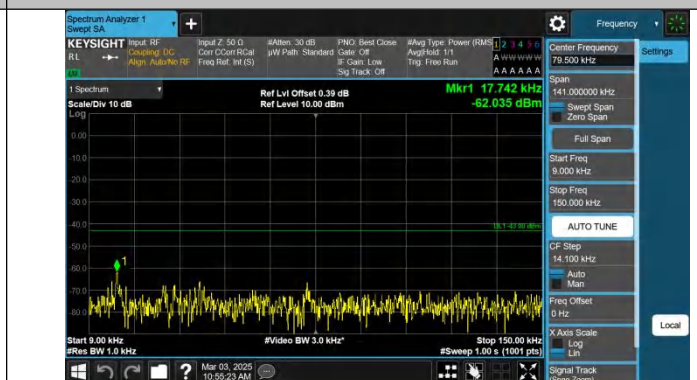
Band2-15MHz-QPSK-18675-1RB#74-0.009~0.15-PASS
