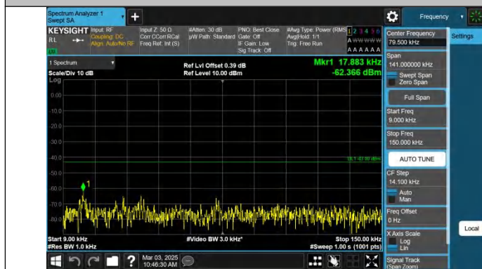
Band2-10MHz-QPSK-18900-1RB#0-0.009~0.15-PASS
