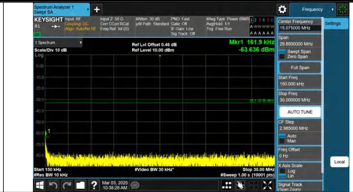
Band2-5MHz-QPSK-19175-1RB#0-0.15~30-PASS
