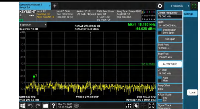
Band2-15MHz-QPSK-19125-1RB#74-0.009~0.15-PASS
