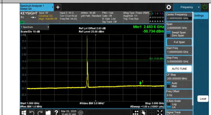
Band2-10MHz-QPSK-18900-1RB#0-1000~3000-PASS
