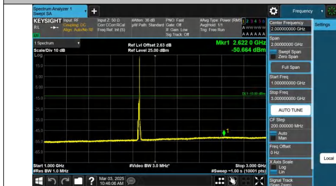
Band2-10MHz-QPSK-18650-1RB#49-1000~3000-PASS
