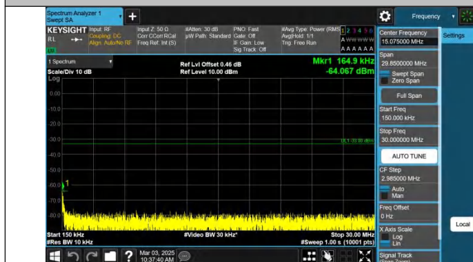
Band2-5MHz-QPSK-18900-1RB#24-0.15~30-PASS
