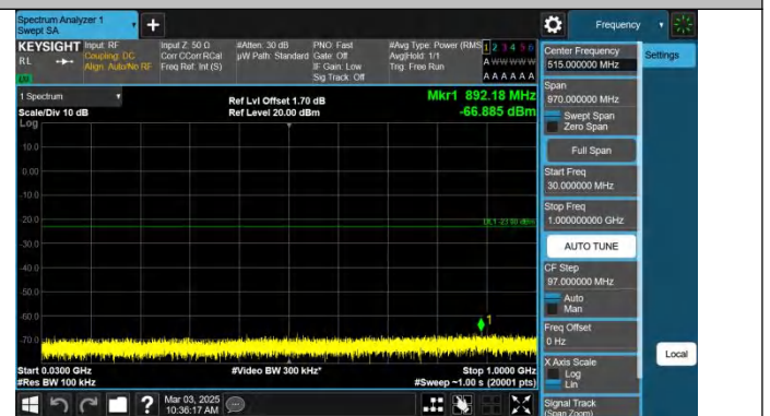
Band2-5MHz-QPSK-18625-1RB#24-30~1000-PASS
