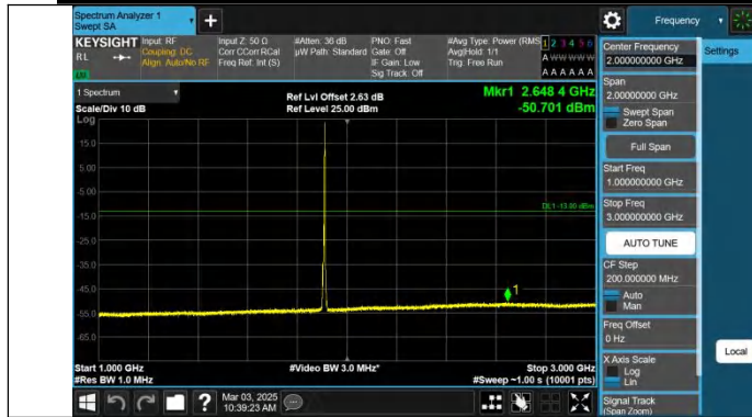
Band2-5MHz-QPSK-19175-1RB#24-1000~3000-PASS
