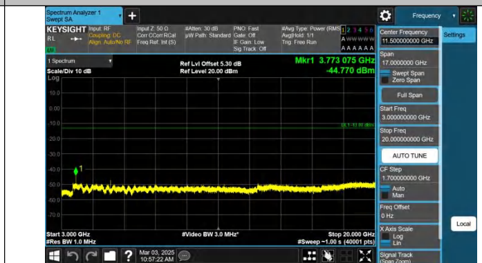
Band2-15MHz-QPSK-18900-1RB#74-3000~20000-PASS
