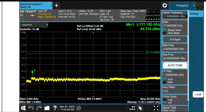
Band2-20MHz-QPSK-18900-1RB#99-3000~20000-PASS
