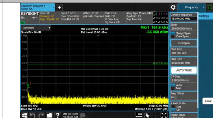
Band2-5MHz-QPSK-18625-1RB#0-0.15~30-PASS
