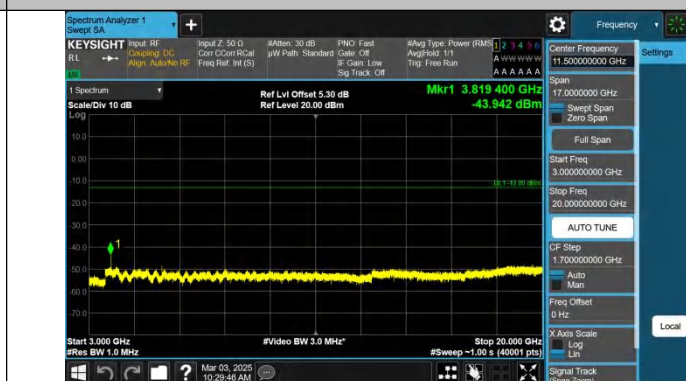
Band2-3MHz-QPSK-19185-1RB#14-3000~20000-PASS
