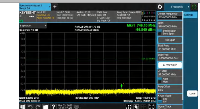
Band2-5MHz-QPSK-19175-1RB#24-30~1000-PASS
