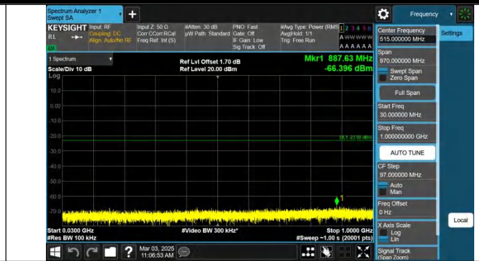
Band2-20MHz-QPSK-19100-1RB#99-30~1000-PASS
