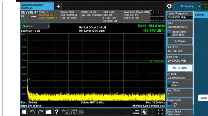
Band2-20MHz-QPSK-19100-1RB#99-0.15~30-PASS
