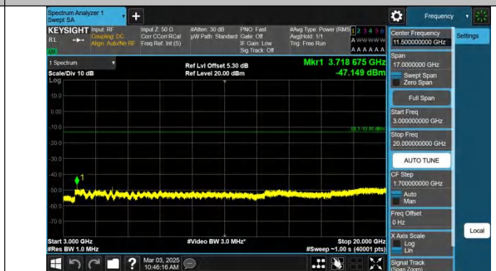
Band2-10MHz-QPSK-18650-1RB#49-3000~20000-PASS
