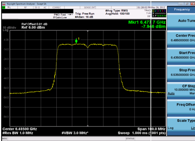
Plot 7-168. Power Spectral Density Plot Antenna 5b (40MHz 802.11ax (UNII Band 6) – Ch. 107, MCS11)
