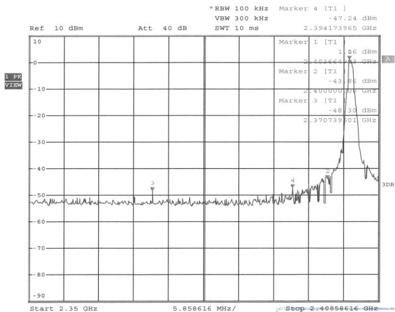
20140814 DW-24H Band edge Emission H
