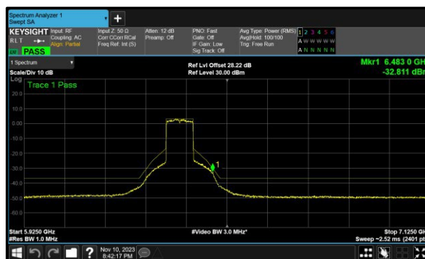
Figure 225 - B(Core 1) 802.11ax HE80 SU SP 6385 MHz (CH87)
