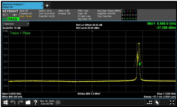
Figure 227 - B(Core 1) 802.11ax HE20 RU106 SP 6855 MHz (CH181)
