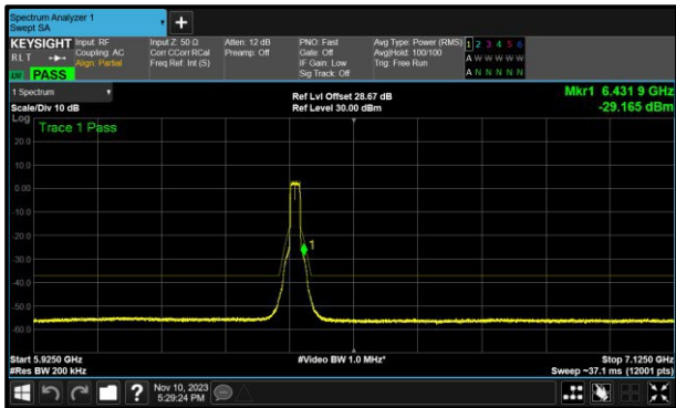
Figure 195 - A(Core 0) 802.11a SP 6415 MHz (CH93)
