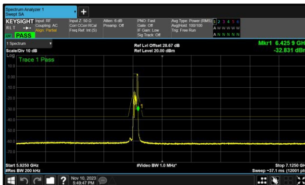
Figure 202- A(Core 0) 802.11ax HE20 RU52 SP 6415 MHz (CH93)
