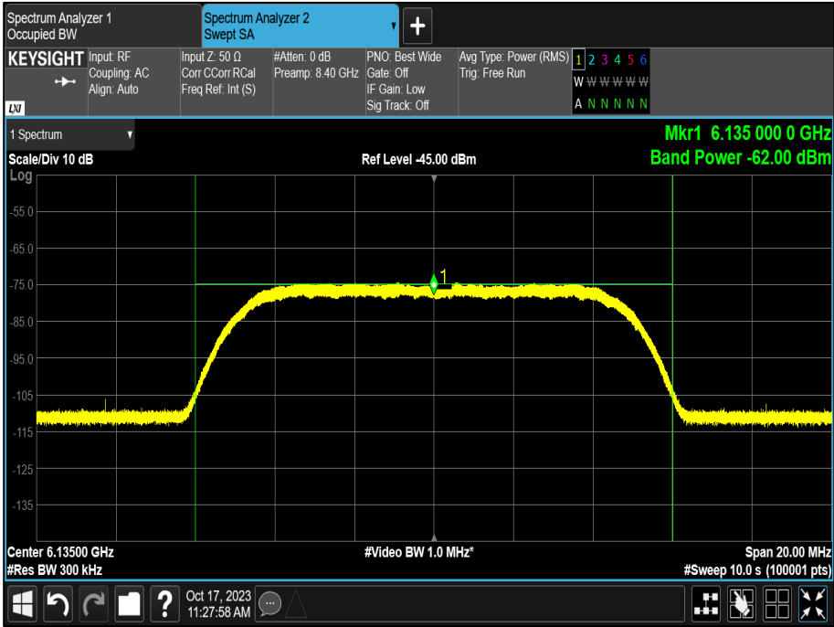
Figure 193 - Example of AWGN Signal
