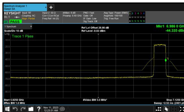
Figure 205 - A(Core 0) 802.11ax HE80 SU LPI 6945 MHz (CH199)
