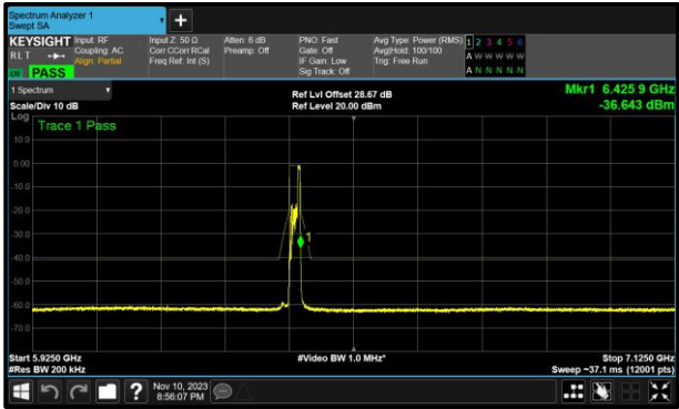
Figure 229 - A(Core 0) 802.11ax HE20 RU52 SP 6415 MHz (CH93)
