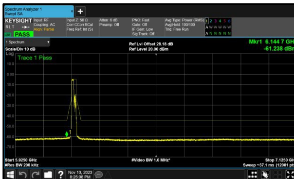
Figure 213 - A(Core 0) 802.11ax HE20 RU106 SP 6175 MHz (CH45)
