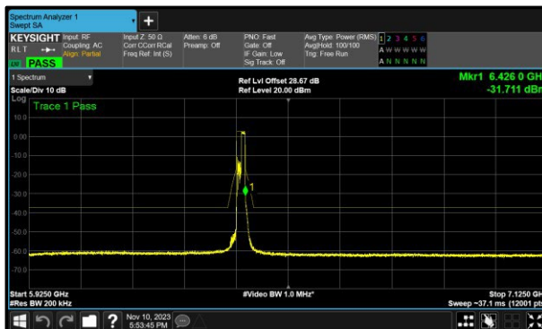
Figure 200- A(Core 0) 802.11ax HE20 RU106 SP 6415 MHz (CH93)
