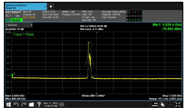
Figure 208- A(Core 0) 802.11ax HE20 RU52 LPI 6475 MHz (CH105)
