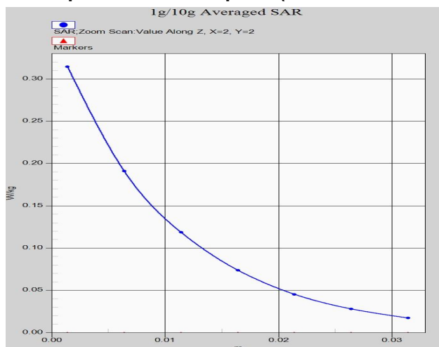
Z-Scan at power reference point (WCDMA1900 ANT31)
