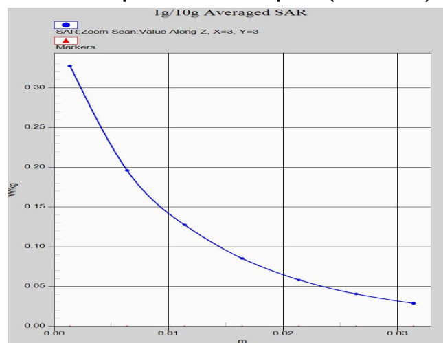
Z-Scan at power reference point (N5 ANT41)
