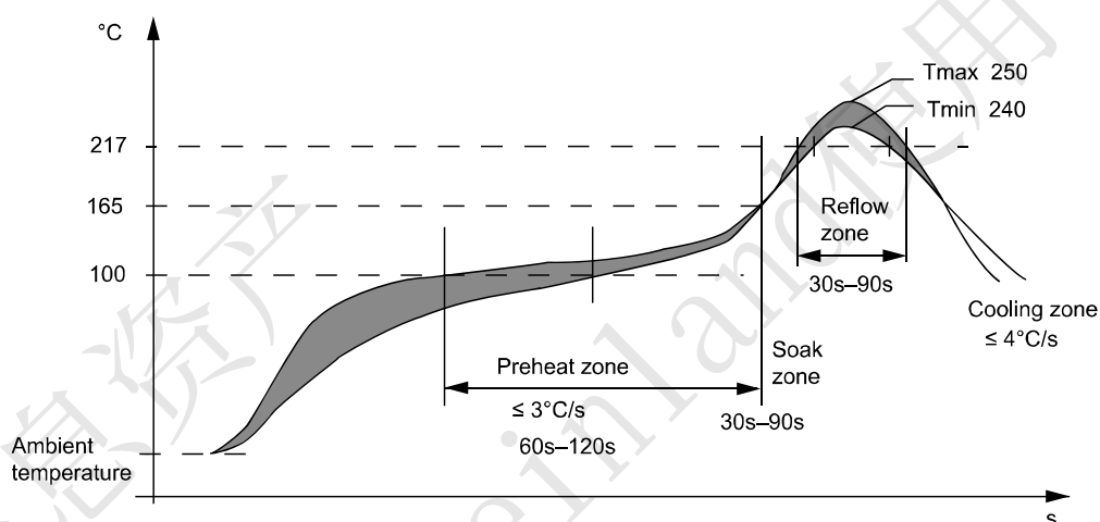
Figure 6-24 Temperature graph of rework
