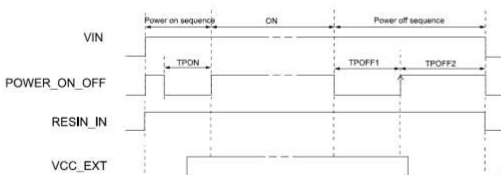
Figure 3-6 Recommended power on timing sequence
