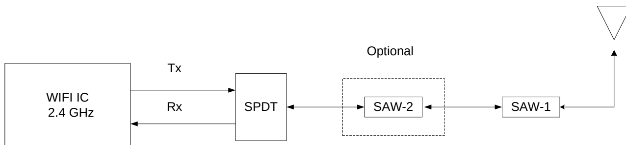
Figure 4-1 Recommended Structure
