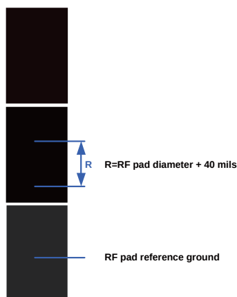
Figure 3-24 RF Pad design
