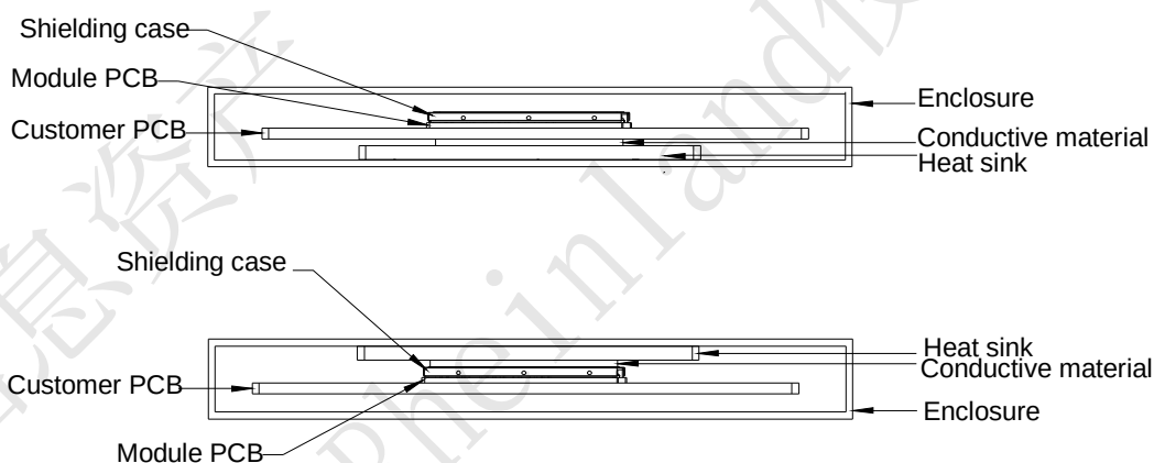
Figure 6-20 Adding enclosure to enhance the heat dissipation of the module
