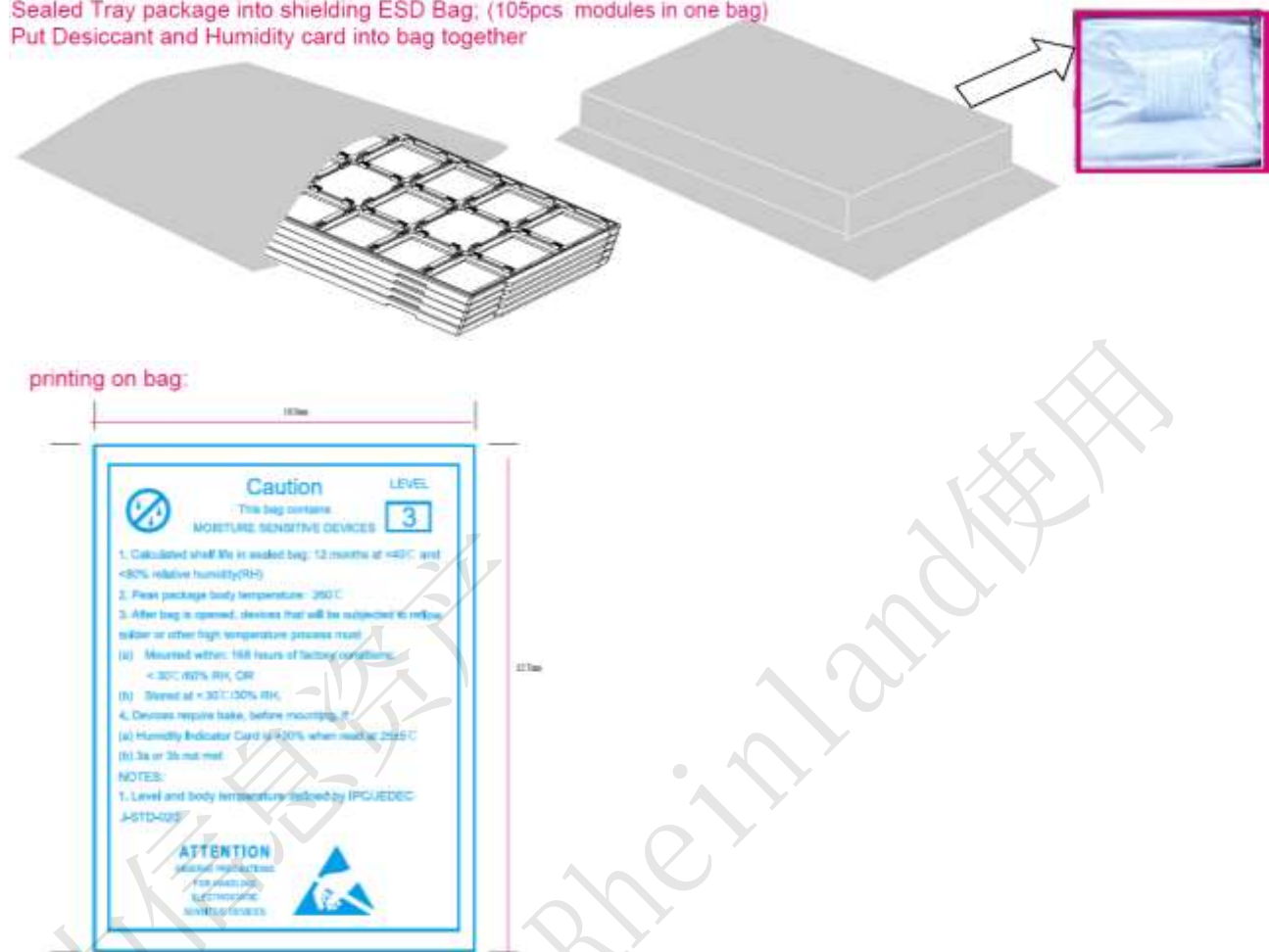
Figure 6-4 ESD packaging
