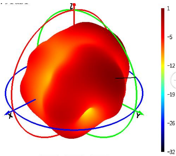
Bluetooth
