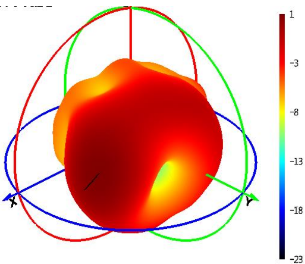
Bluetooth
