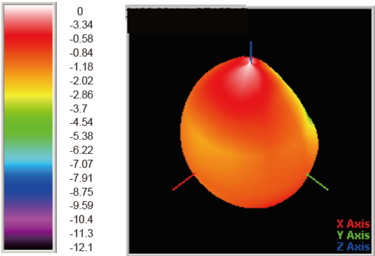
◎ 3D Gain Pattern (2450 MHz) Unit:dBi
