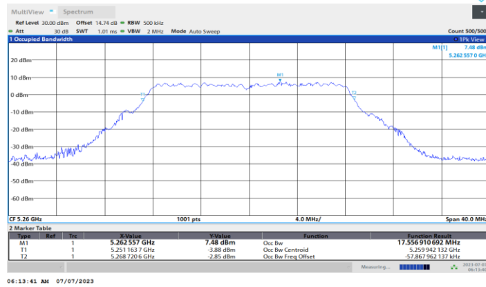
11A-CDD_Ant3_5260
